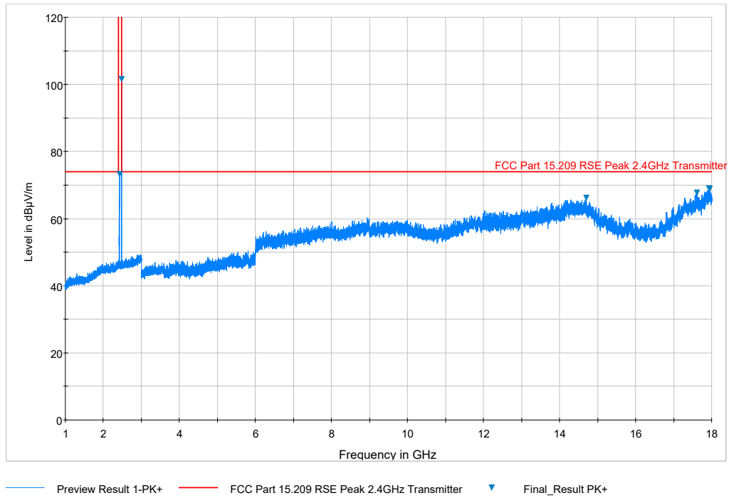
Plot 7-46. Radiated Spurious Plot above 1GHz (BT – Ch. 78, Ant. Pol. H)
