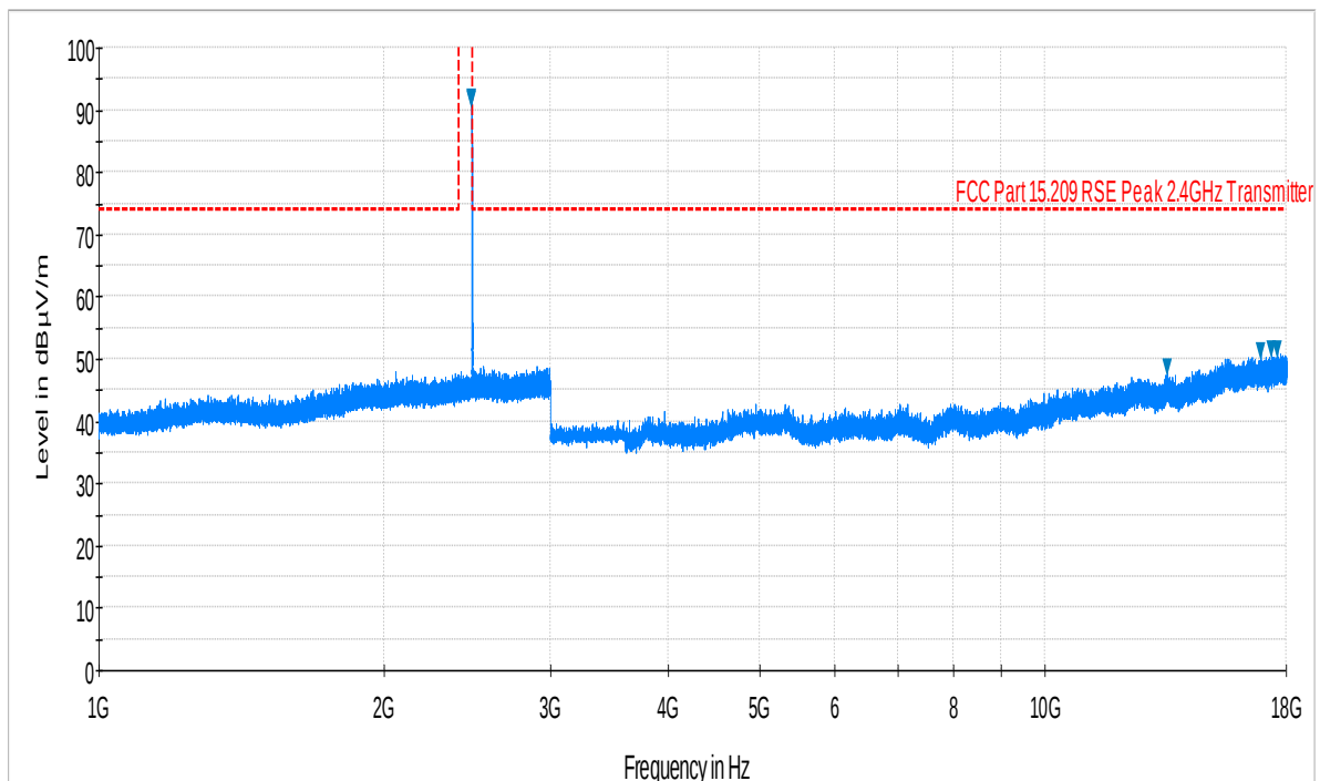
Plot 6-6. Radiated Spurious Plot above 1GHz (Bluetooth LE – Ch. 39, Ant. Pol. V)
