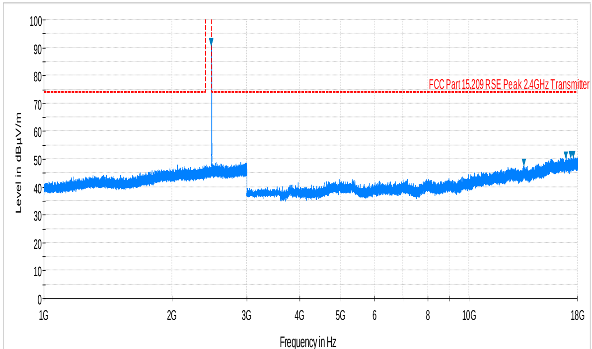
Plot 6-5. Radiated Spurious Plot above 1GHz (Bluetooth LE – Ch. 39, Ant. Pol. H)
