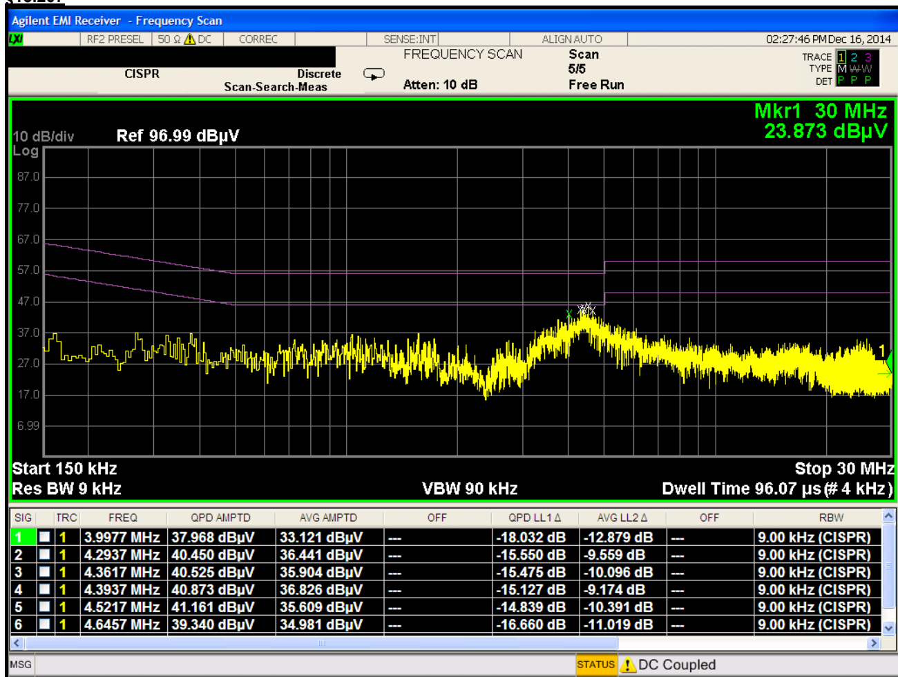
Plot 6-35. Line Conducted Plot with 802.11b (L1)
