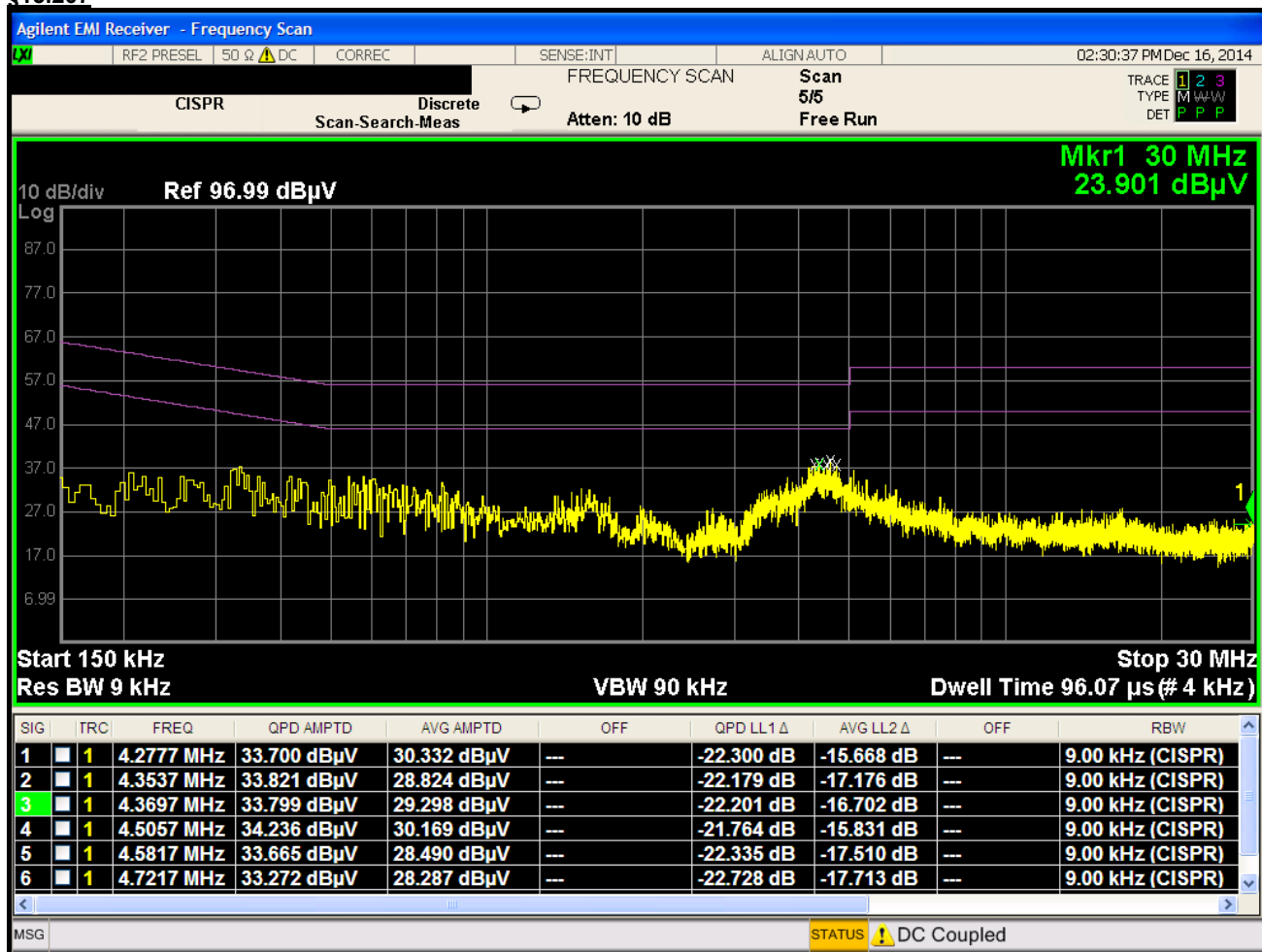
Plot 6-36. Line Conducted Plot with 802.11b (N)
