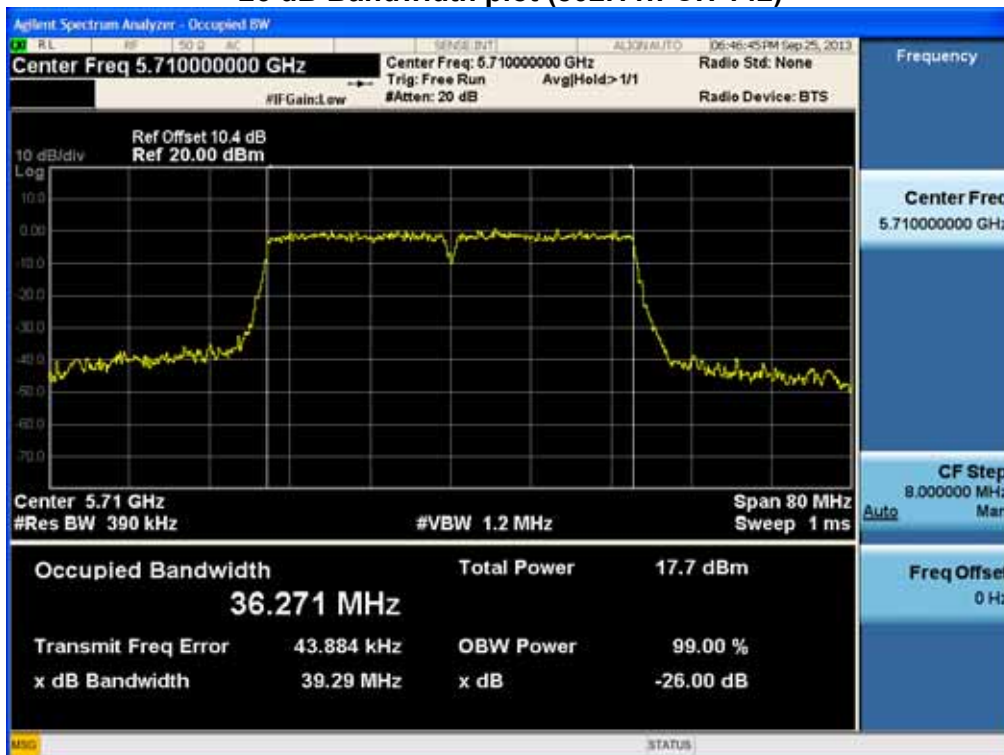
26 dB Bandwidth plot (802.11n-CH 142)
