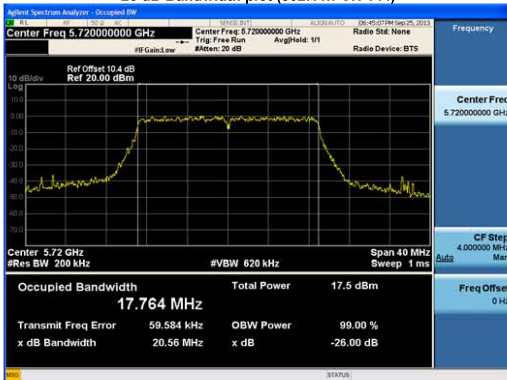
26 dB Bandwidth plot (802.11n-CH 144)
