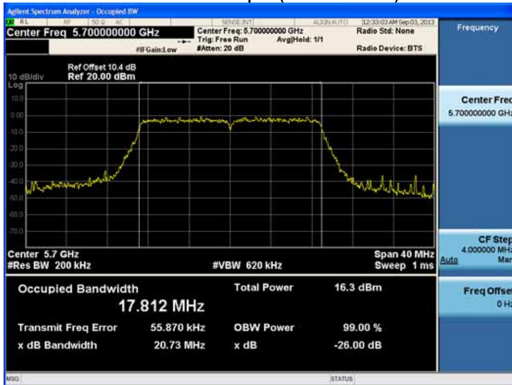
26 dB Bandwidth plot (802.11n-CH 140)
