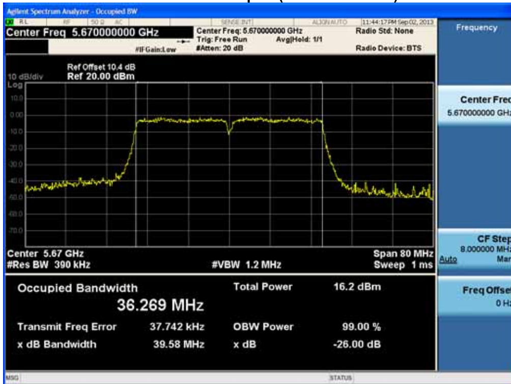
26 dB Bandwidth plot (802.11n-CH 134)
