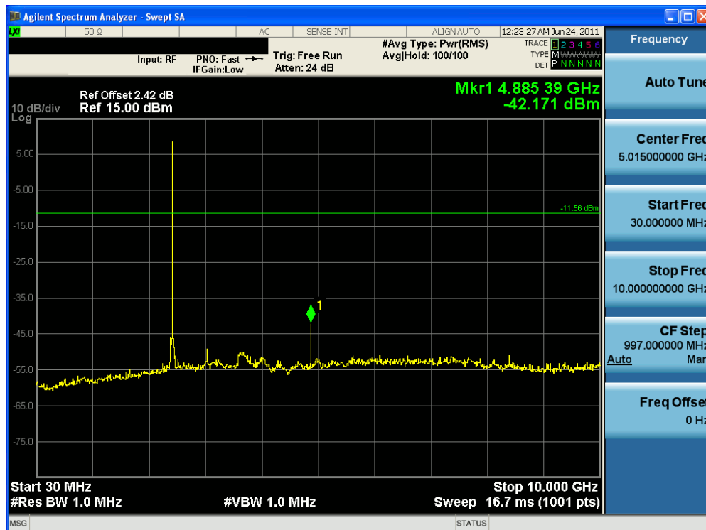
Plot 6-20. Conducted Spurious Plot (Bluetooth, 3Mbps – Ch. 39)
