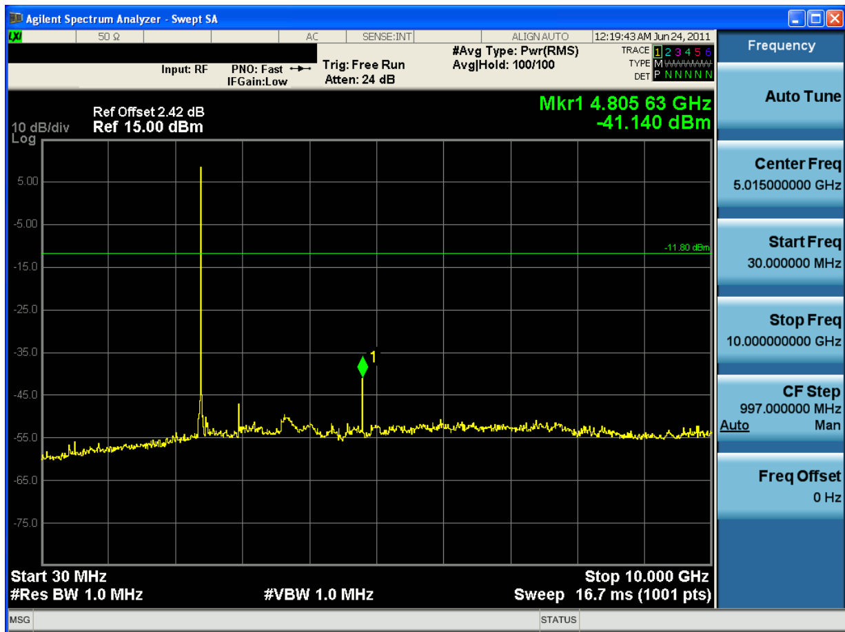
Plot 6-18. Conducted Spurious Plot (Bluetooth, 3Mbps – Ch. 0)
