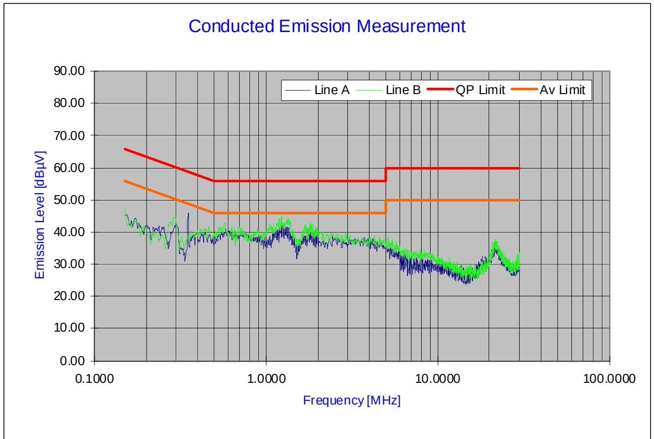
Plot 6-33. Line Conducted Plot with 802.11n
