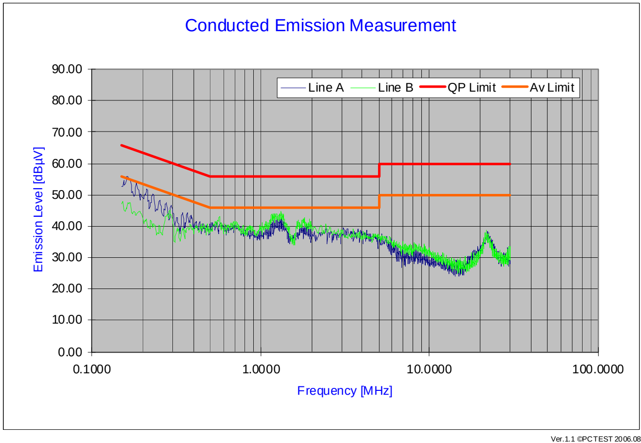
Plot 6-31. Line Conducted Plot with 802.11b
