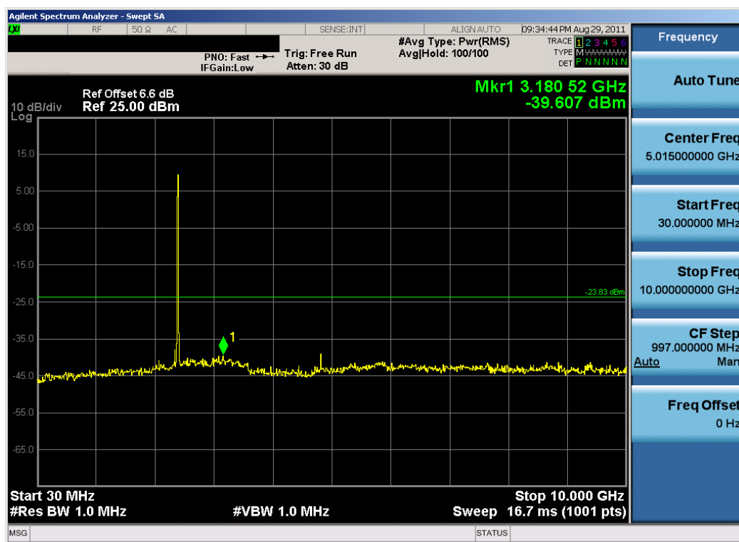
Plot 6-25. Conducted Spurious Plot (802.11b – Ch. 1)
