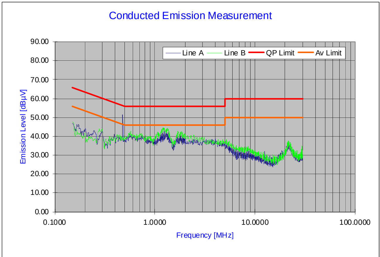
Plot 6-32. Line Conducted Plot with 802.11g
