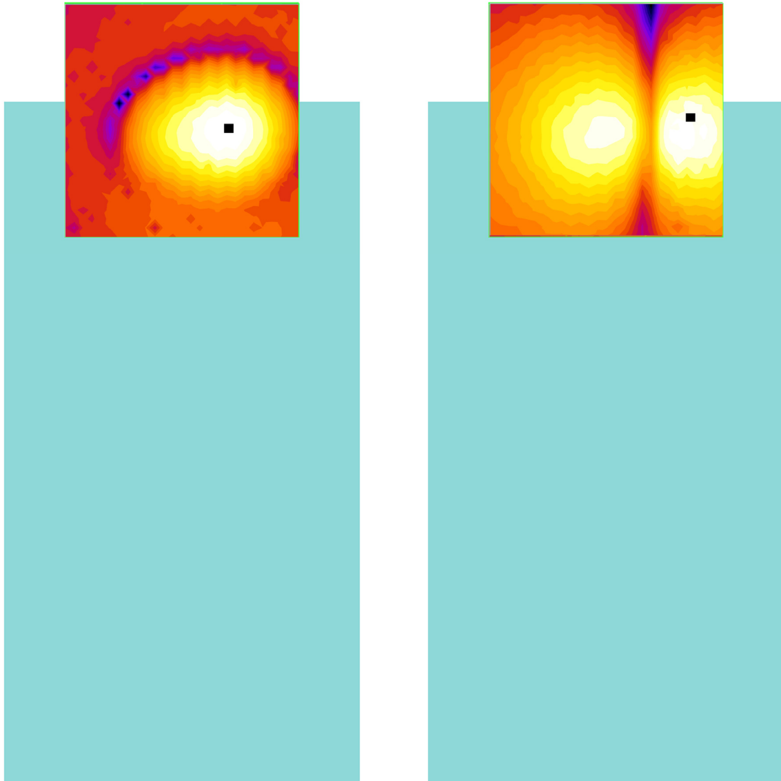
Figure 7-1 T-Coil Scan Overlay Magnetic Field Distributions
