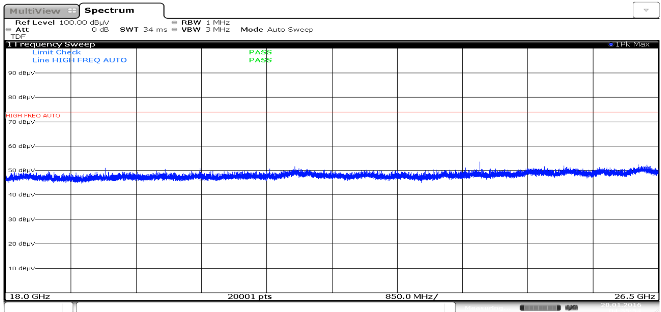
Plot 7-8. Radiated Spurious Plot above 18GHz (Pol. V)
