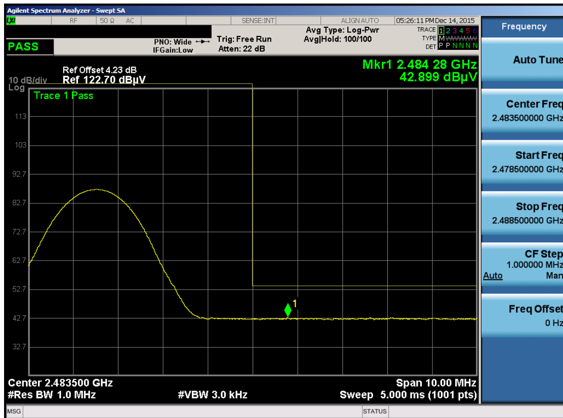
Plot 7-18. Radiated Restricted Upper Band Edge Measurement (Average)
