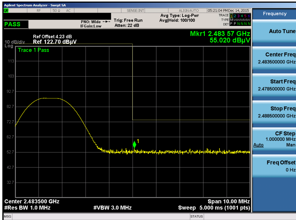
Plot 7-19. Radiated Restricted Upper Band Edge Measurement (Peak)
