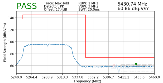
Plot 7-104. Radiated Upper Band Edge Plot (Peak – UNII Band 2A)
