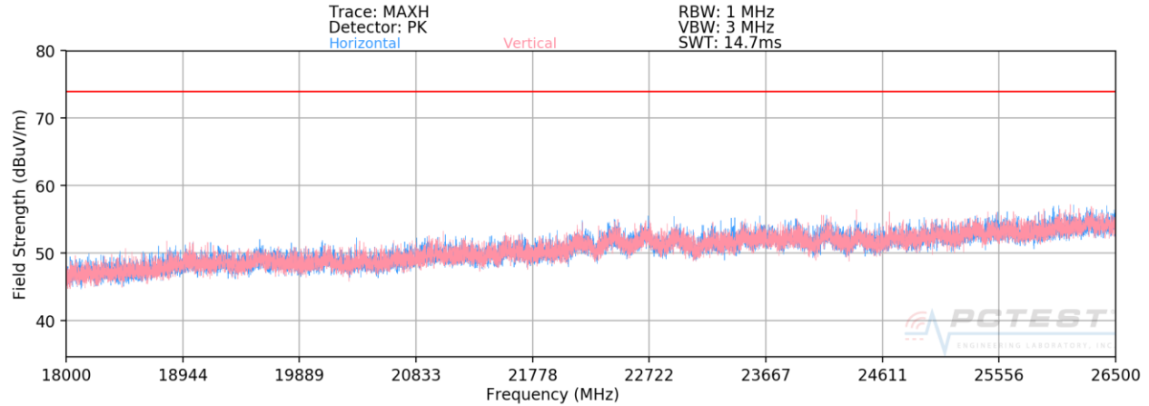
Plot 7-81. Radiated Spurious Plot 18GHz - 26.5GHz (802.11a)
