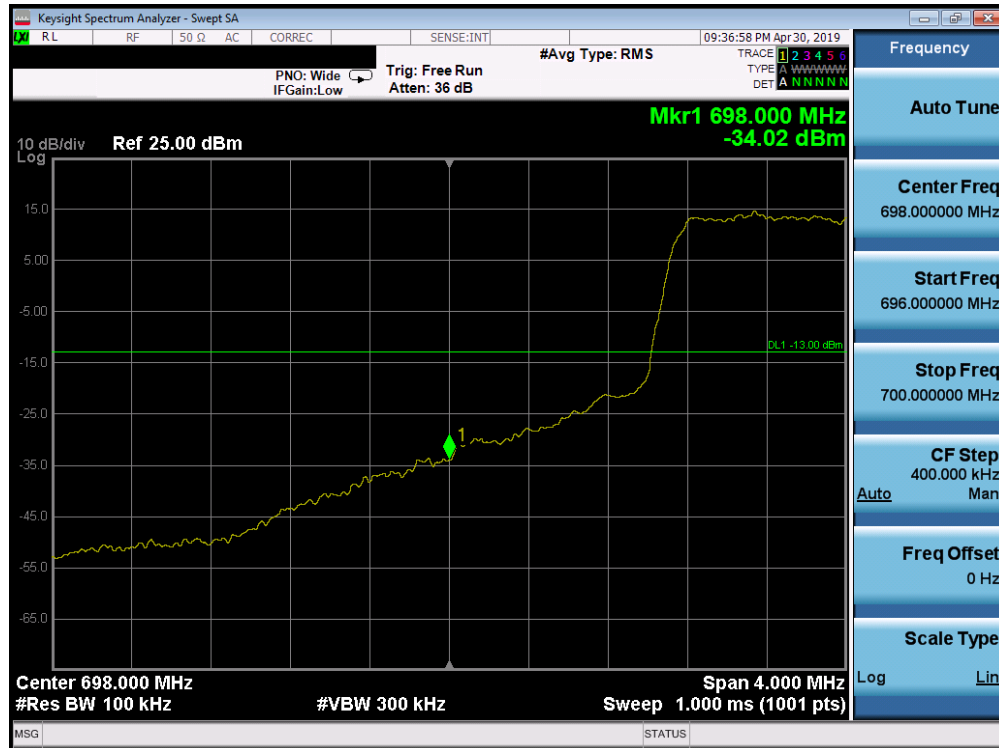
Plot 7-141. Lower Band Edge Plot (Band 12 - 1.4MHz QPSK - Full RB Configuration)
