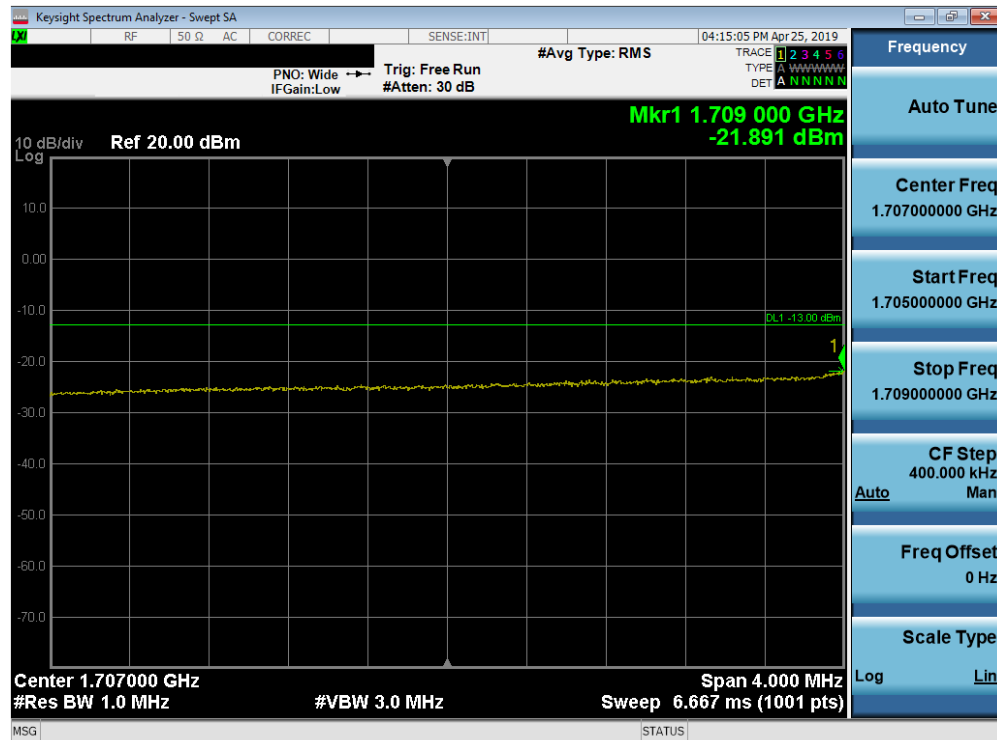
Plot 7-190. Lower Extended Band Edge Plot (Band 66/4 - 15.0MHz QPSK - Full RB Configuration)
