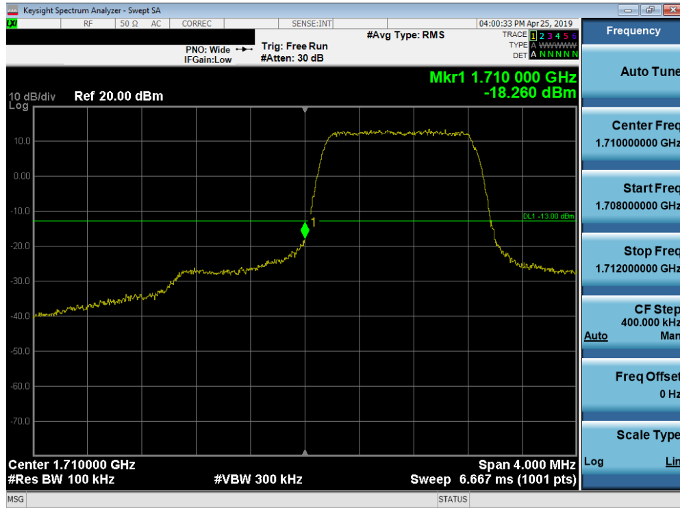
Plot 7-165. Lower Band Edge Plot (Band 66/4 - 1.4MHz QPSK - Full RB Configuration)
