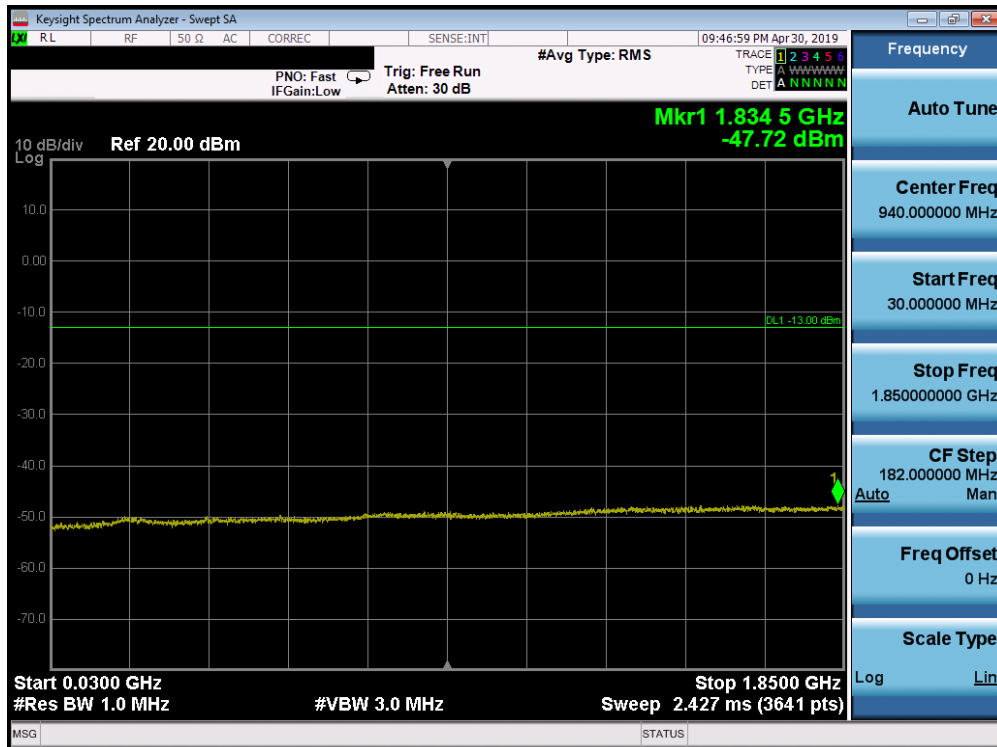
Plot 7-130. Conducted Spurious Plot (Band 2 - 15.0MHz QPSK - RB Size 1, RB Offset 0 - High Channel)
