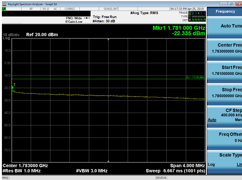
Plot 7-188. Upper Extended Band Edge Plot (Band 66 - 10.0MHz QPSK - Full RB Configuration)
