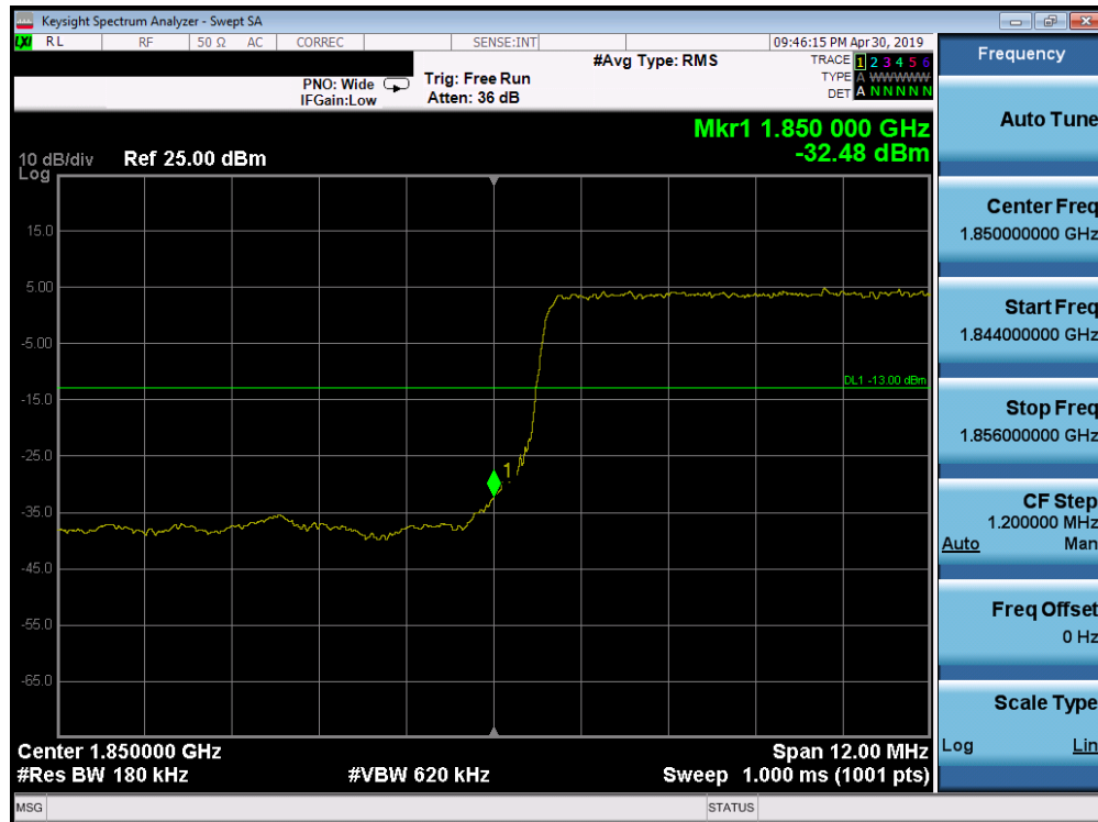
Plot 7-217. Lower Band Edge Plot (Band 2 - 15.0MHz QPSK - Full RB Configuration)
