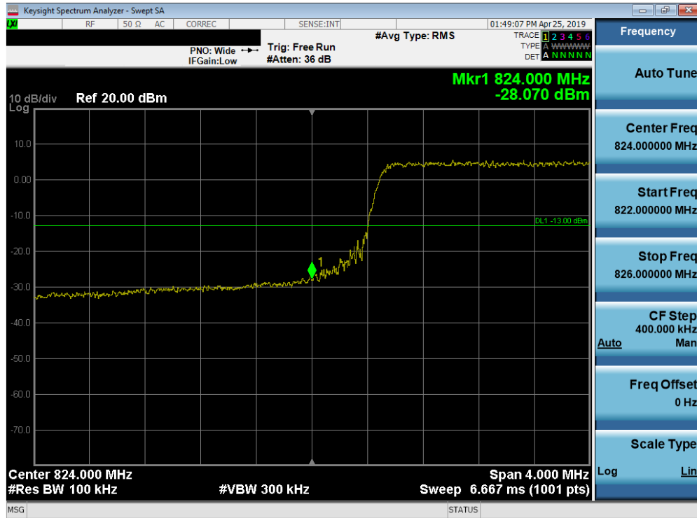
Plot 7-163. Lower Band Edge Plot (Band 5 - 10.0MHz QPSK - Full RB Configuration)
