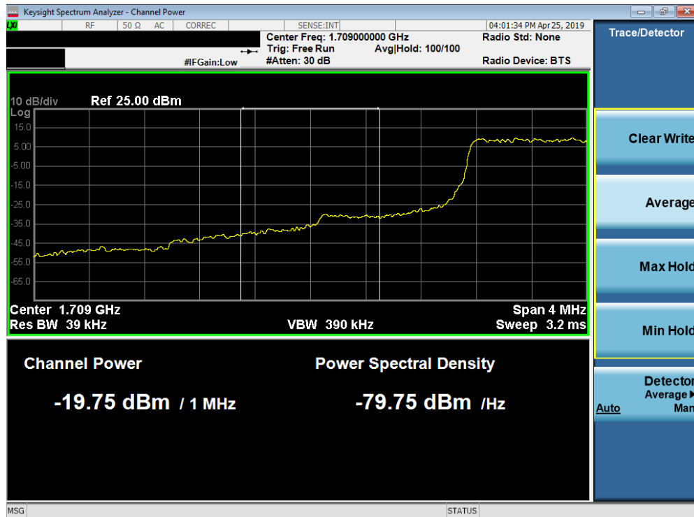
Plot 7-166. Lower Extended Band Edge Plot (Band 66/4 - 1.4MHz QPSK - Full RB Configuration)
