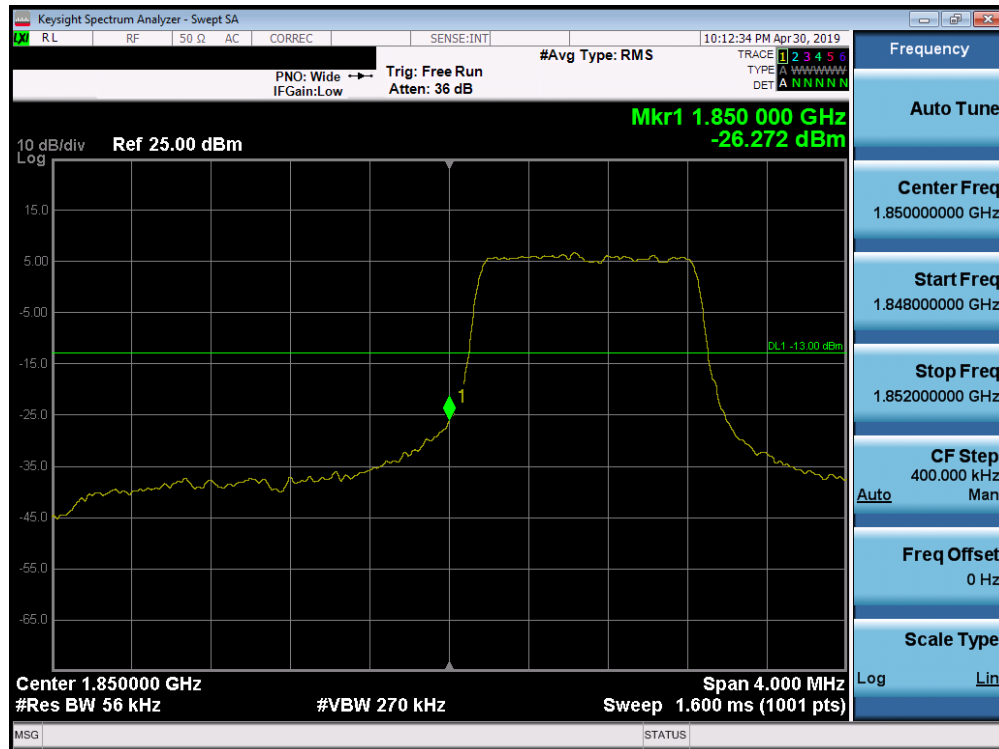
Plot 7-201. Lower Band Edge Plot (Band 2 - 1.4MHz QPSK - Full RB Configuration)
