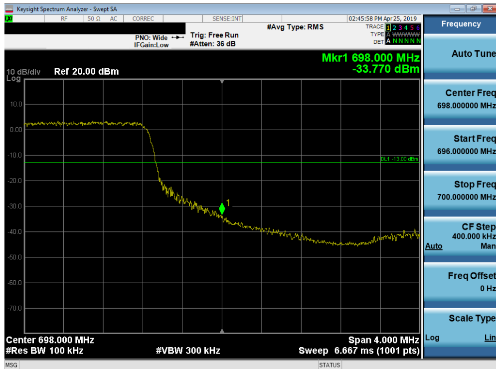
Plot 7-138. Upper Band Edge Plot (Band 71 - 15.0MHz QPSK - Full RB Configuration)
