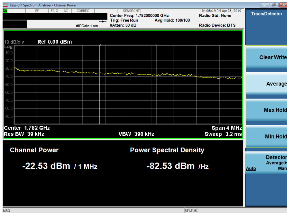
Plot 7-182. Upper Extended Band Edge Plot (Band 66 - 5.0MHz QPSK - Full RB Configuration)
