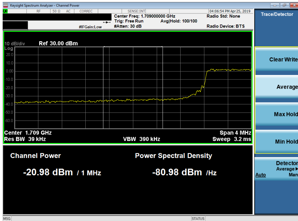
Plot 7-178. Lower Extended Band Edge Plot (Band 66/4 - 5.0MHz QPSK - Full RB Configuration)
