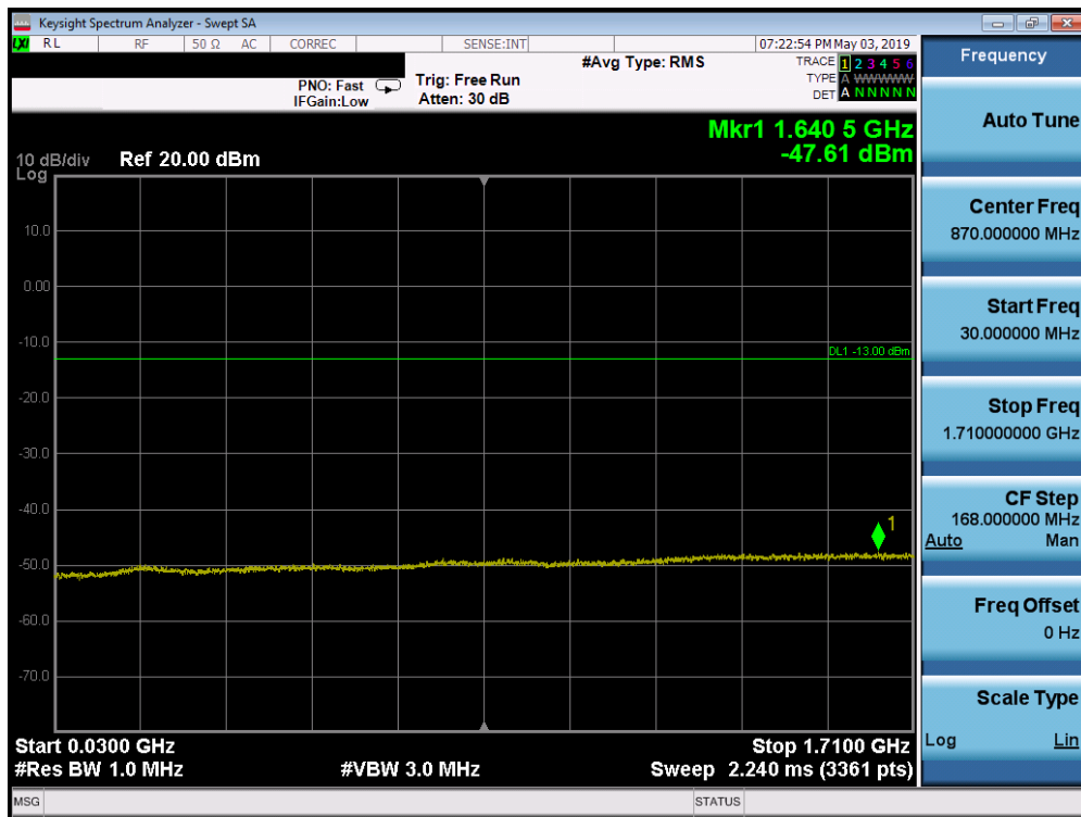
Plot 7-118. Conducted Spurious Plot (Band 66/4 - 20.0MHz QPSK - RB Size 1, RB Offset 0 - Mid Channel)
