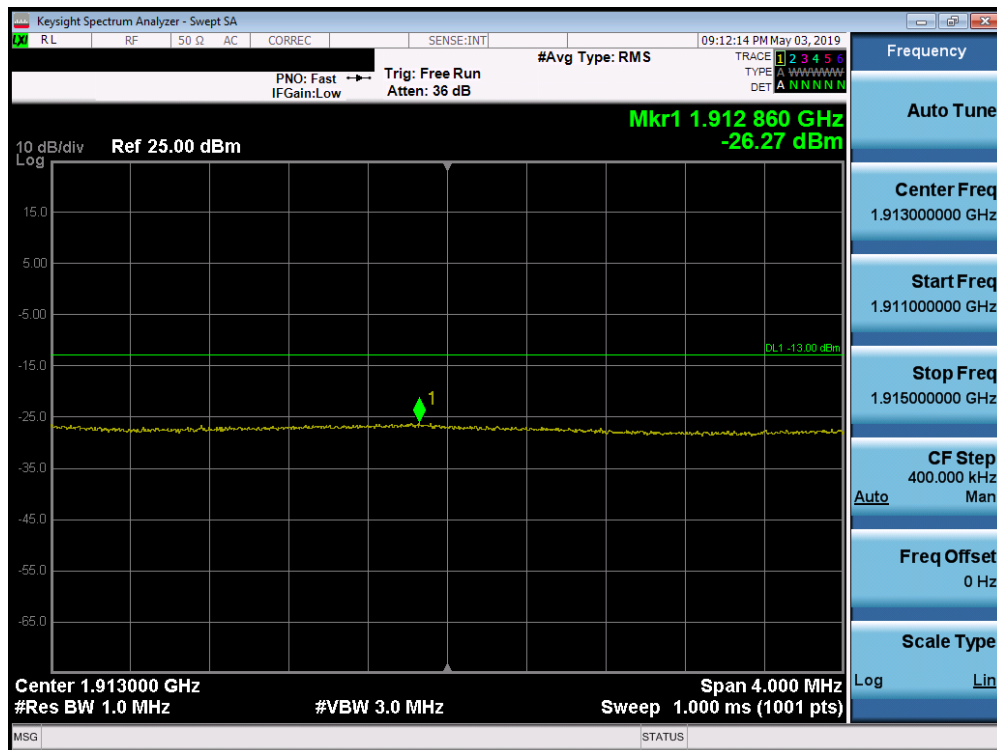
Plot 7-220. Upper Extended Band Edge Plot (Band 2 - 15MHz QPSK - Full RB Configuration)
