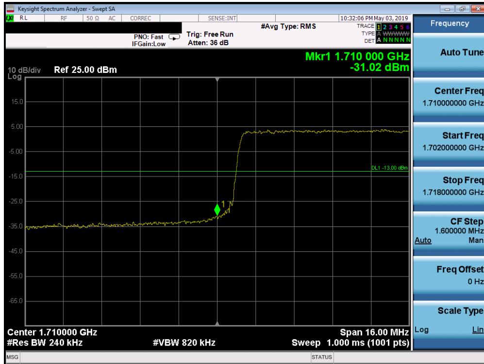
Plot 7-195. Lower Band Edge Plot (Band 66/4 - 20.0MHz QPSK - Full RB Configuration)
