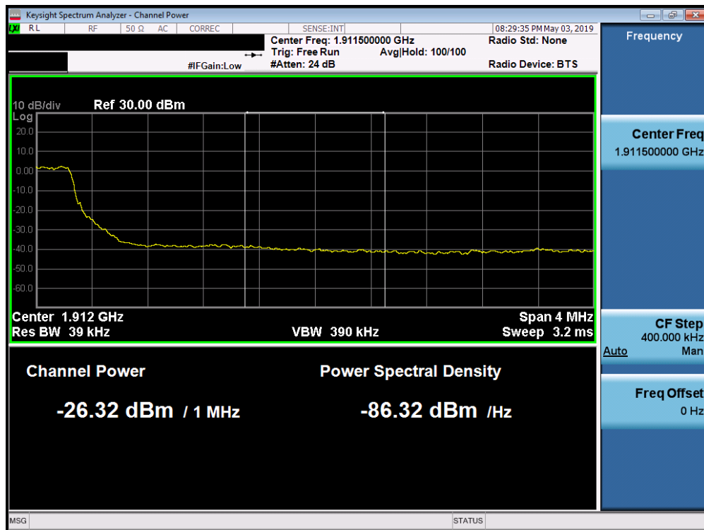
Plot 7-212. Upper Extended Band Edge Plot (Band 2 - 5MHz QPSK - Full RB Configuration)
