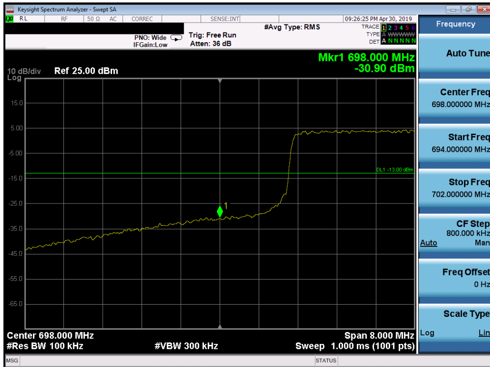
Plot 7-147. Lower Band Edge Plot (Band 12 - 10.0MHz QPSK - Full RB Configuration)
