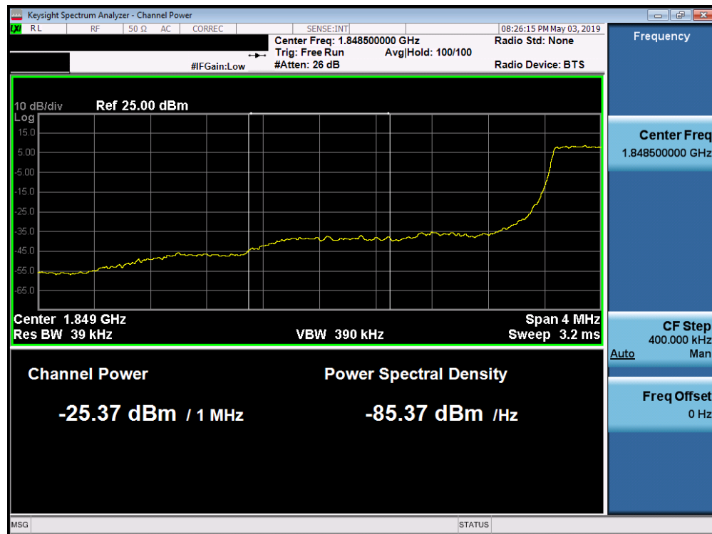
Plot 7-202. Lower Extended Band Edge Plot (Band 2 - 1.4MHz QPSK - Full RB Configuration)
