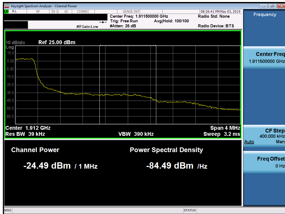
Plot 7-204. Upper Extended Band Edge Plot (Band 2 - 1.4MHz QPSK - Full RB Configuration)
