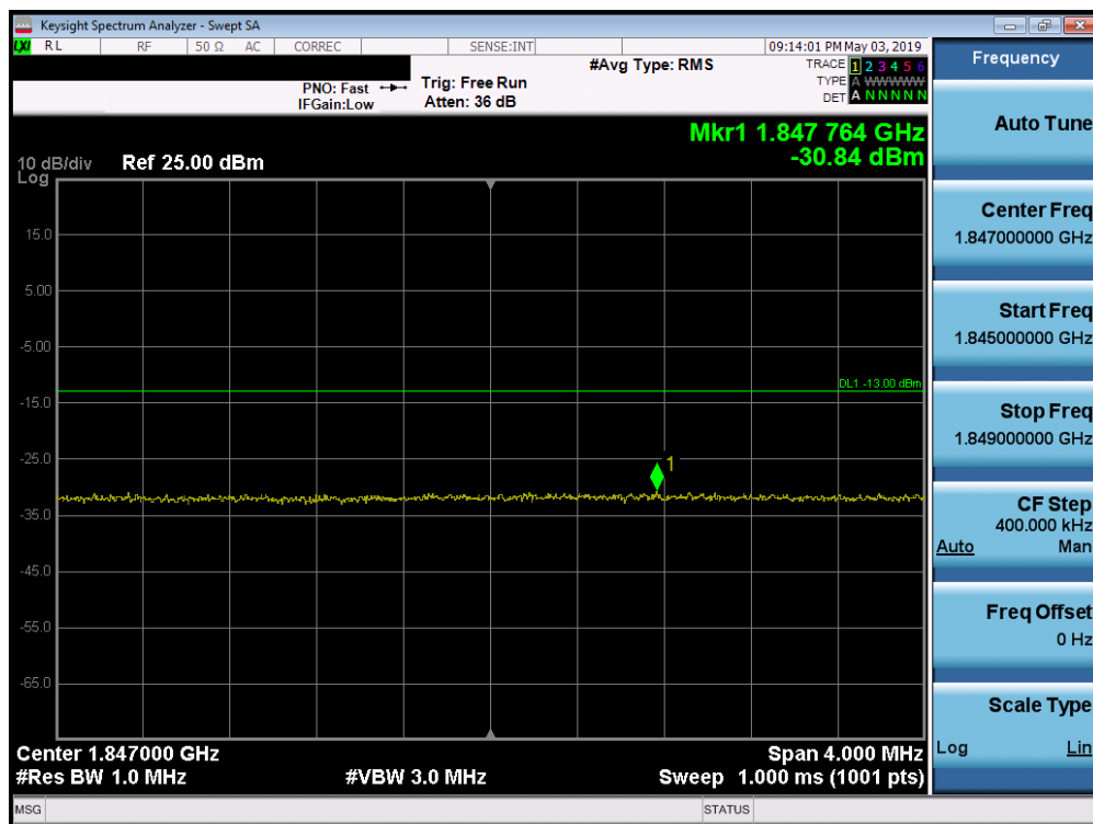
Plot 7-222. Lower Extended Band Edge Plot (Band 2 - 20MHz QPSK - Full RB Configuration)
