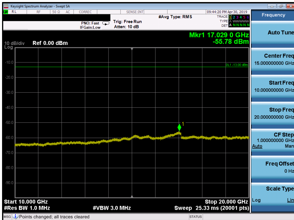
Plot 7-129. Conducted Spurious Plot (Band 2 - 15.0MHz QPSK - RB Size 1, RB Offset 0 - Mid Channel)
