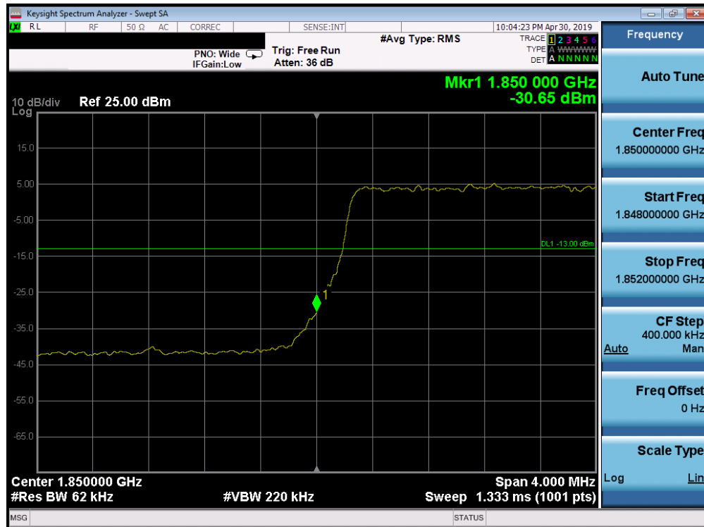
Plot 7-209. Lower Band Edge Plot (Band 2 - 5.0MHz QPSK - Full RB Configuration)
