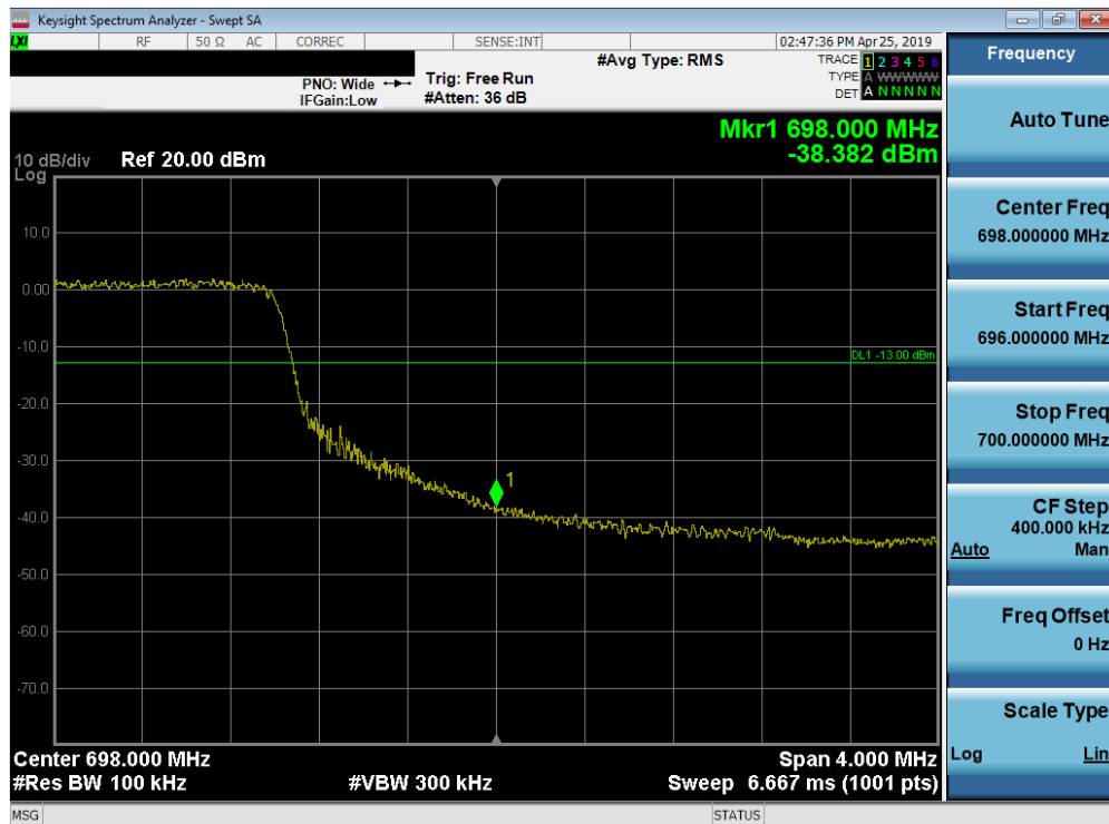
Plot 7-140. Upper Band Edge Plot (Band 71 - 20.0MHz QPSK - Full RB Configuration)
