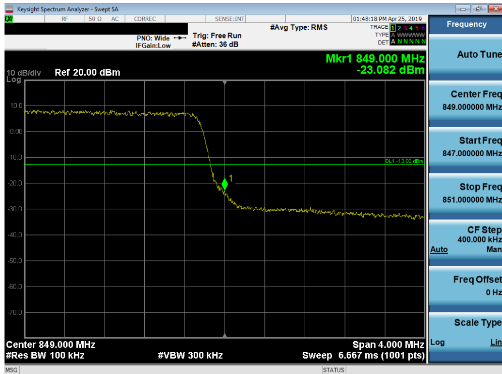
Plot 7-162. Upper Band Edge Plot (Band 5 - 5.0MHz QPSK - Full RB Configuration)
