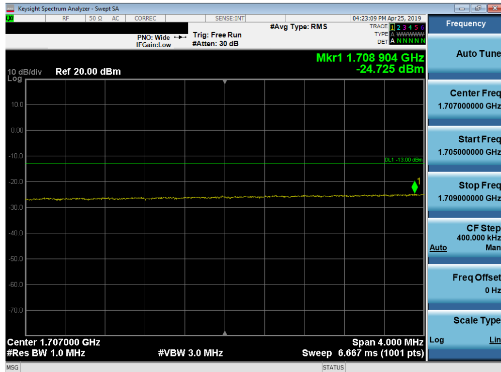
Plot 7-196. Lower Extended Band Edge Plot (Band 66/4 - 20.0MHz QPSK - Full RB Configuration)
