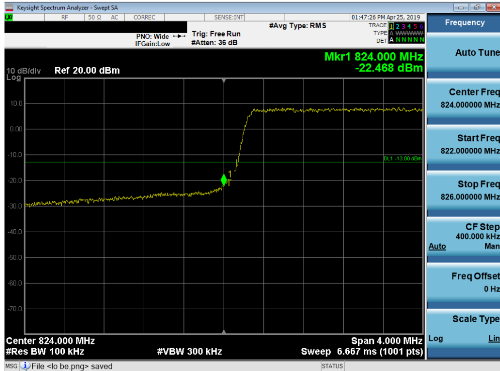
Plot 7-161. Lower Band Edge Plot (Band 5 - 5.0MHz QPSK - Full RB Configuration)
