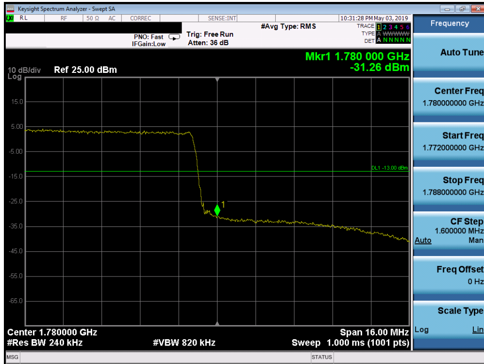
Plot 7-199. Upper Band Edge Plot (Band 66 - 20.0MHz QPSK - Full RB Configuration)
