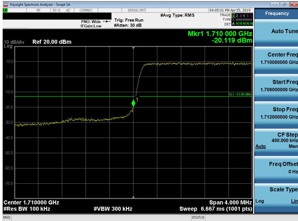
Plot 7-171. Lower Band Edge Plot (Band 66/4 - 3.0MHz QPSK - Full RB Configuration)
