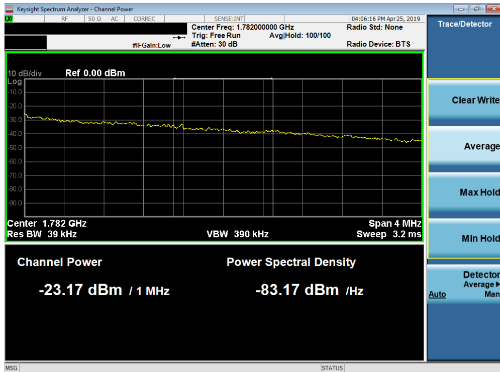
Plot 7-176. Upper Extended Band Edge Plot (Band 66 - 3.0MHz QPSK - Full RB Configuration)
