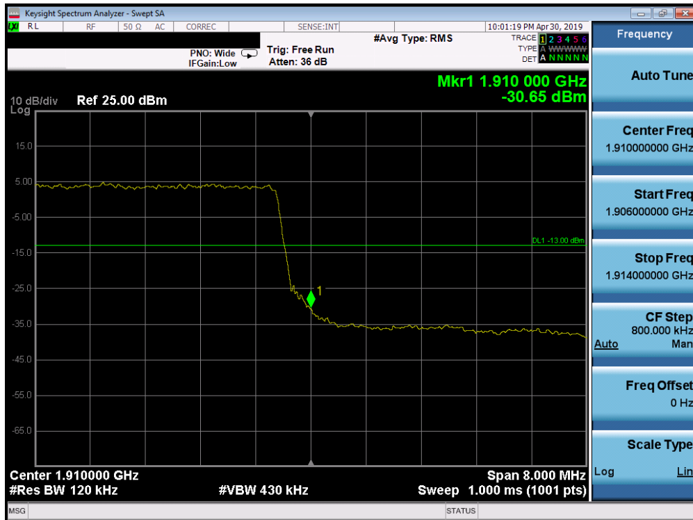
Plot 7-215. Upper Band Edge Plot (Band 2 - 10.0MHz QPSK - Full RB Configuration)
