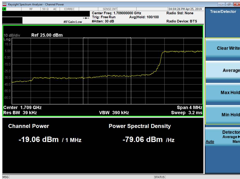
Plot 7-172. Lower Extended Band Edge Plot (Band 66/4 - 3.0MHz QPSK - Full RB Configuration)
