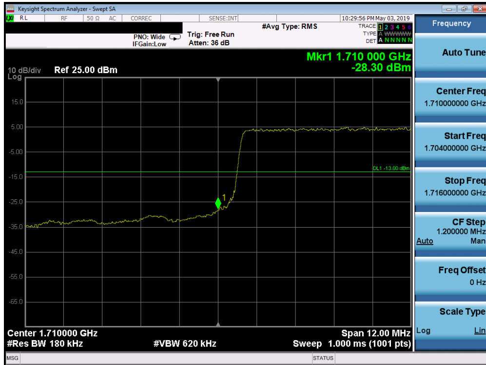
Plot 7-189. Lower Band Edge Plot (Band 66/4 - 15.0MHz QPSK - Full RB Configuration)
