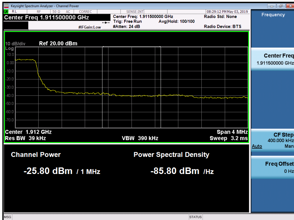
Plot 7-208. Upper Extended Band Edge Plot (Band 2 - 3MHz QPSK - Full RB Configuration)
