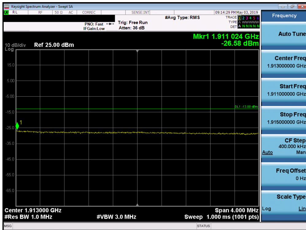
Plot 7-224. Upper Extended Band Edge Plot (Band 2 - 3MHz QPSK - Full RB Configuration)
