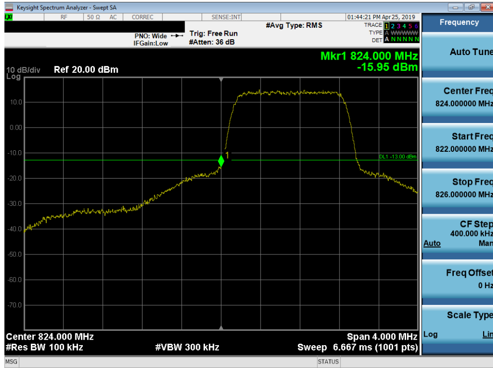
Plot 7-157. Lower Band Edge Plot (Band 5 - 1.4MHz QPSK - Full RB Configuration)
