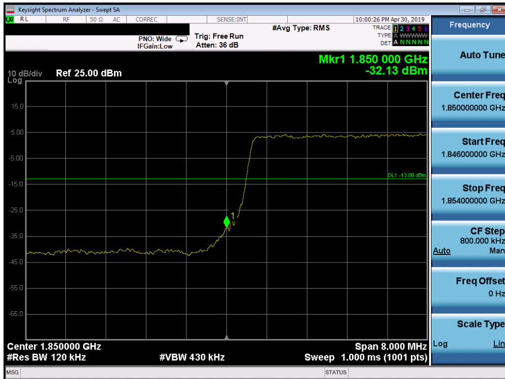
Plot 7-213. Lower Band Edge Plot (Band 2 - 10.0MHz QPSK - Full RB Configuration)
