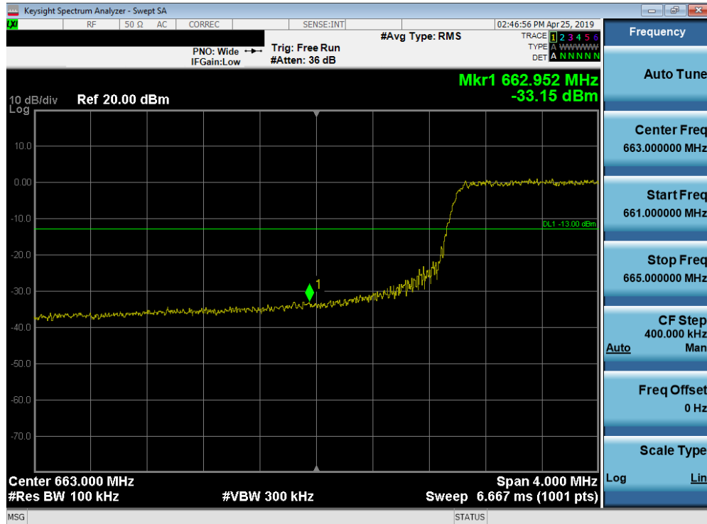
Plot 7-139. Lower Band Edge Plot (Band 71 - 20.0MHz QPSK - Full RB Configuration)
