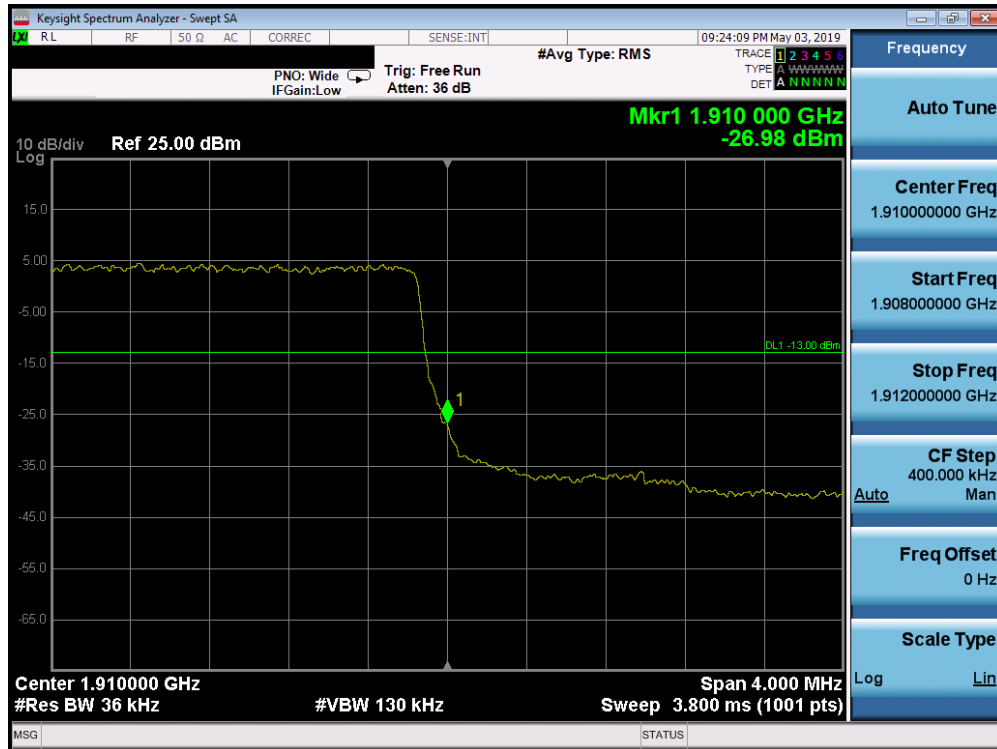
Plot 7-207. Upper Band Edge Plot (Band 2 - 3MHz QPSK - Full RB Configuration)
