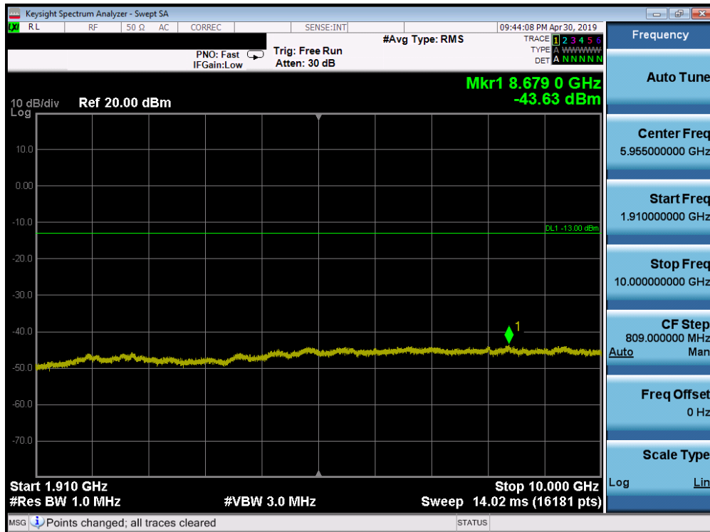
Plot 7-128. Conducted Spurious Plot (Band 2 - 15.0MHz QPSK - RB Size 1, RB Offset 0 - Mid Channel)
