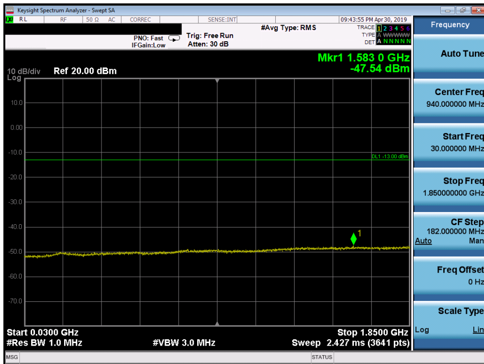
Plot 7-127. Conducted Spurious Plot (Band 2 - 15.0MHz QPSK - RB Size 1, RB Offset 0 - Mid Channel)
