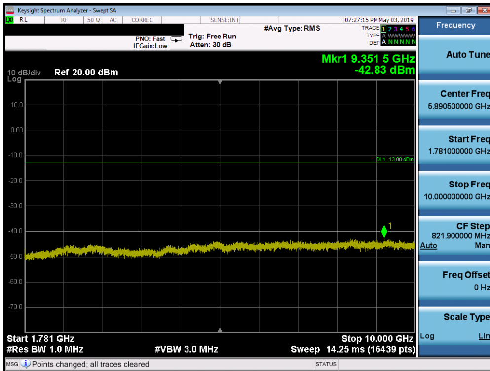
Plot 7-122. Conducted Spurious Plot (Band 66/4 - 20.0MHz QPSK - RB Size 1, RB Offset 0 - High Channel)
