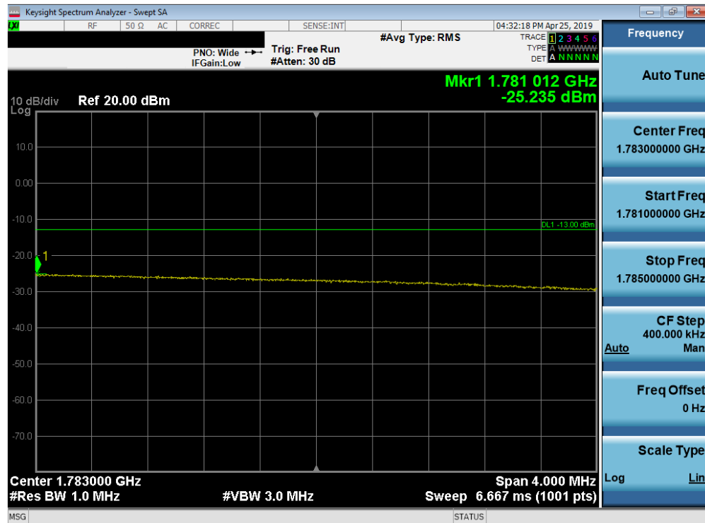
Plot 7-200. Upper Extended Band Edge Plot (Band 66 - 20.0MHz QPSK - Full RB Configuration)
