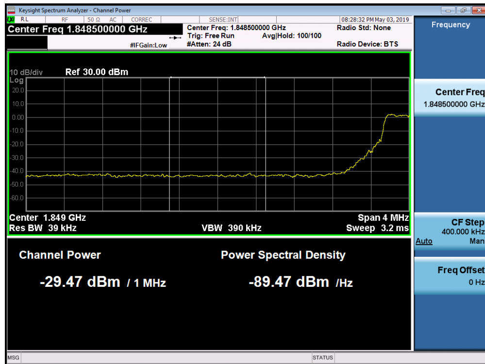
Plot 7-210. Lower Extended Band Edge Plot (Band 2 - 5MHz QPSK - Full RB Configuration)
