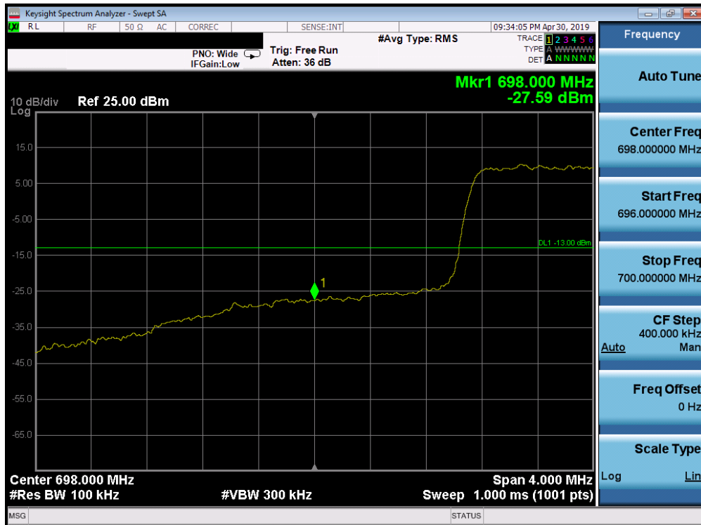
Plot 7-143. Lower Band Edge Plot (Band 12 - 3.0MHz QPSK - Full RB Configuration)
