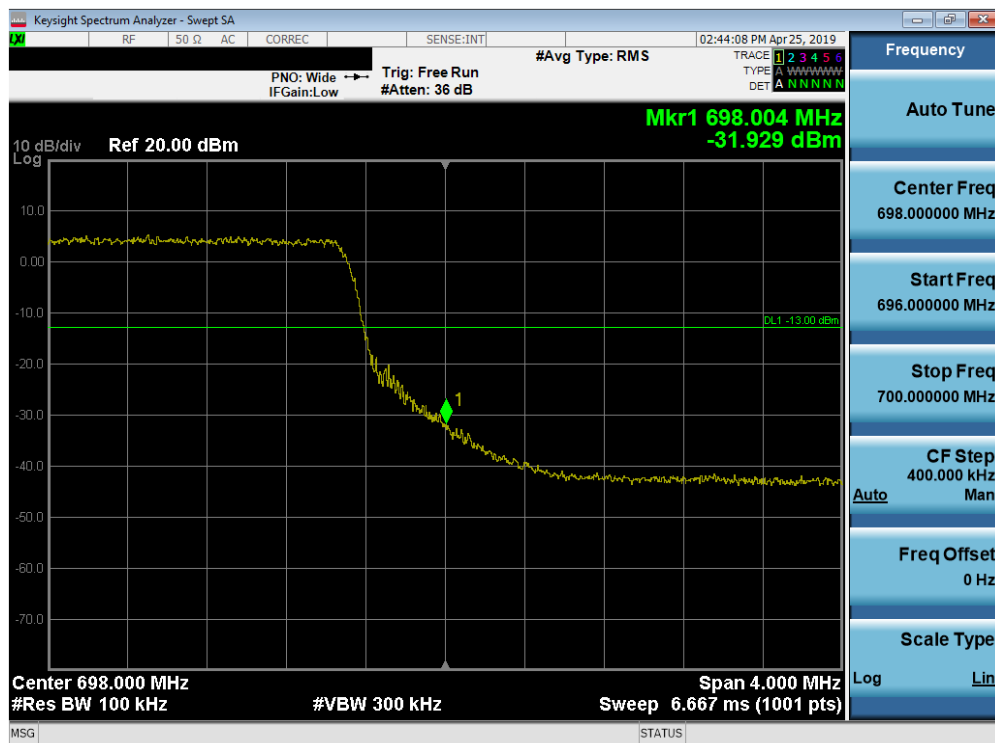
Plot 7-136. Upper Band Edge Plot (Band 71 - 10.0MHz QPSK - Full RB Configuration)
