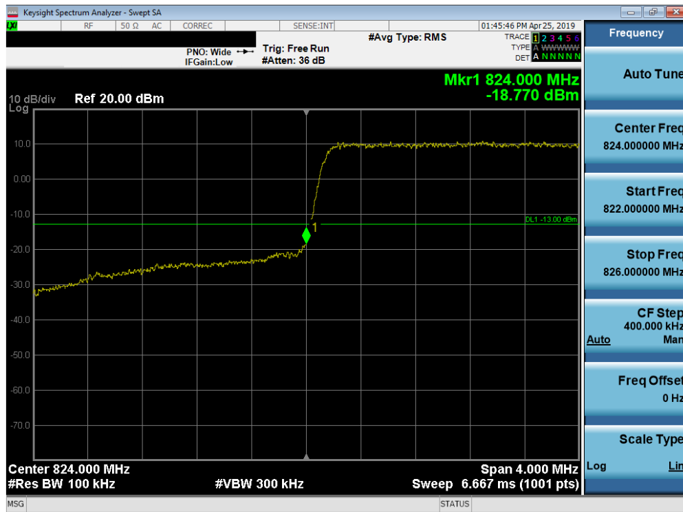
Plot 7-159. Lower Band Edge Plot (Band 5 - 3.0MHz QPSK - Full RB Configuration)
