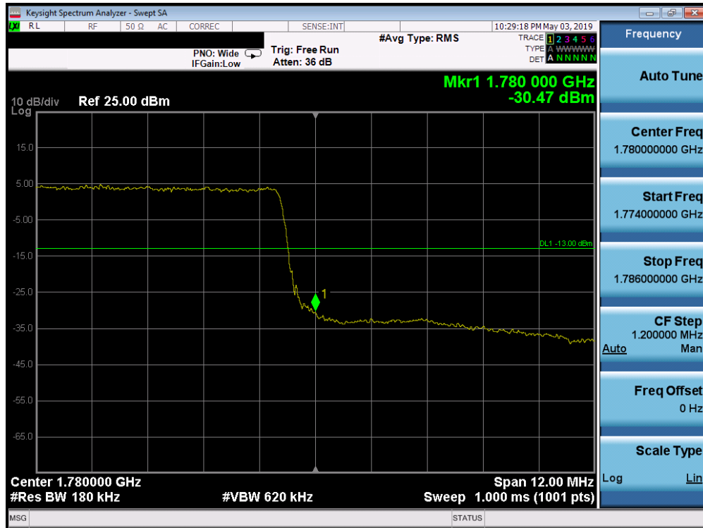
Plot 7-193. Upper Band Edge Plot (Band 66 - 15.0MHz QPSK - Full RB Configuration)
