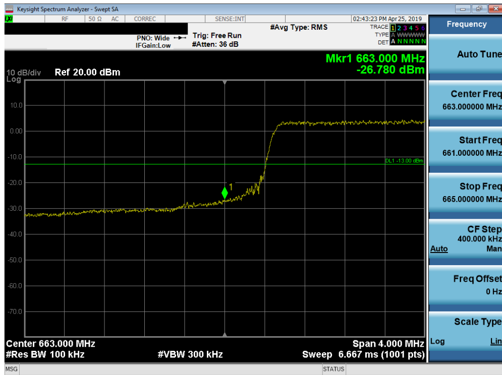
Plot 7-135. Lower Band Edge Plot (Band 71 - 10.0MHz QPSK - Full RB Configuration)
