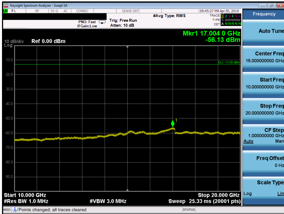
Plot 7-126. Conducted Spurious Plot (Band 2 - 15.0MHz QPSK - RB Size 1, RB Offset 0 - Low Channel)
