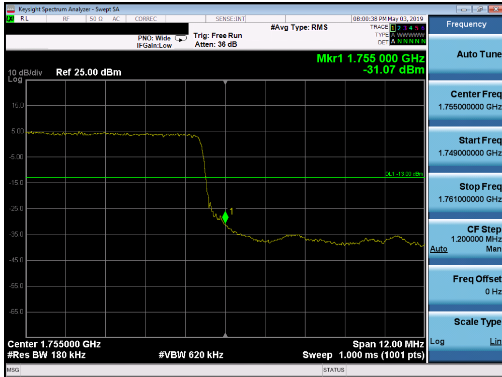
Plot 7-191. Upper Band Edge Plot (Band 4 - 15.0MHz QPSK - Full RB Configuration)
