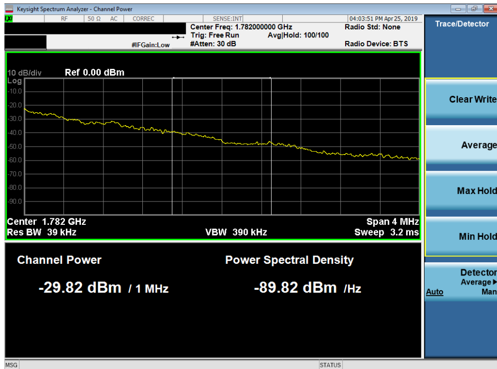
Plot 7-170. Upper Extended Band Edge Plot (Band 66 - 1.4MHz QPSK - Full RB Configuration)
