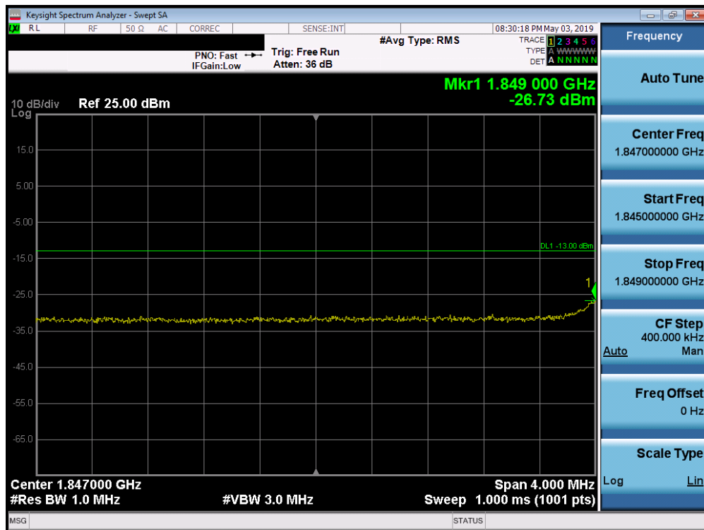
Plot 7-214. Lower Extended Band Edge Plot (Band 2 - 10MHz QPSK - Full RB Configuration)
