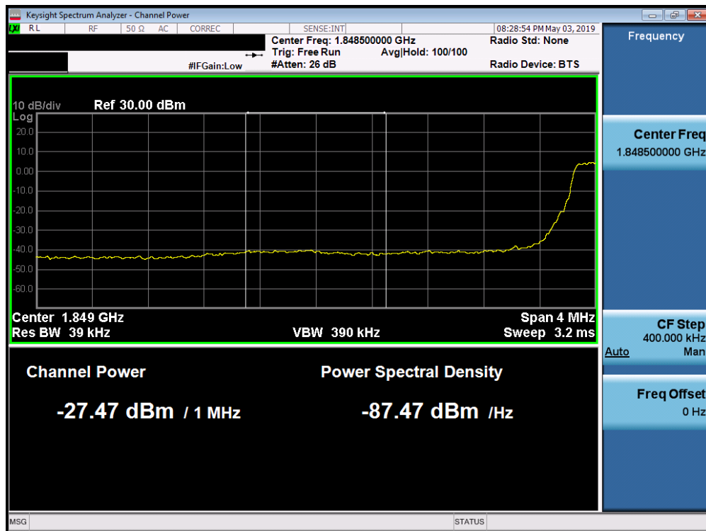
Plot 7-206. Lower Extended Band Edge Plot (Band 2 - 3MHz QPSK - Full RB Configuration)
