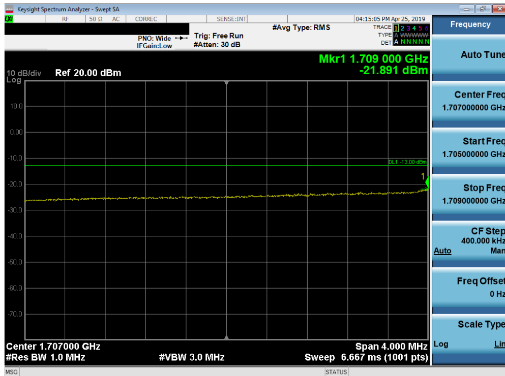
Plot 7-184. Lower Extended Band Edge Plot (Band 66/4 - 10.0MHz QPSK - Full RB Configuration)
