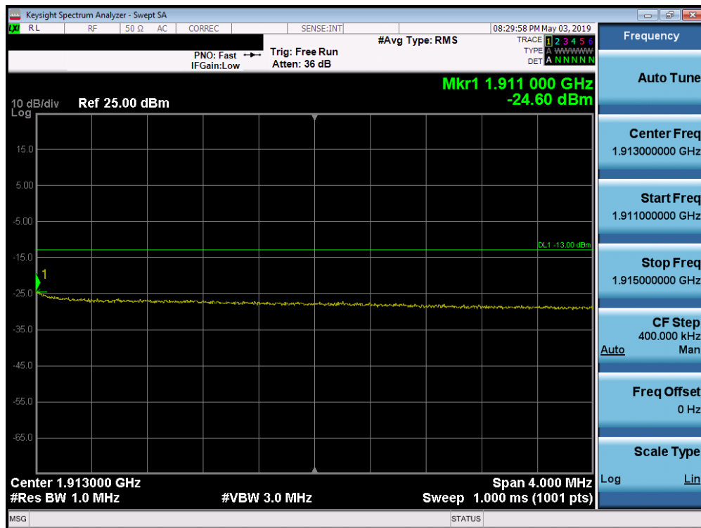
Plot 7-216. Upper Extended Band Edge Plot (Band 2 - 10MHz QPSK - Full RB Configuration)
