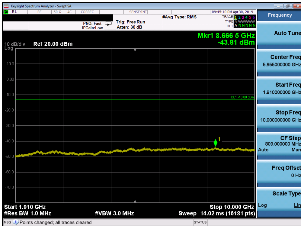
Plot 7-125. Conducted Spurious Plot (Band 2 - 15.0MHz QPSK - RB Size 1, RB Offset 0 - Low Channel)
