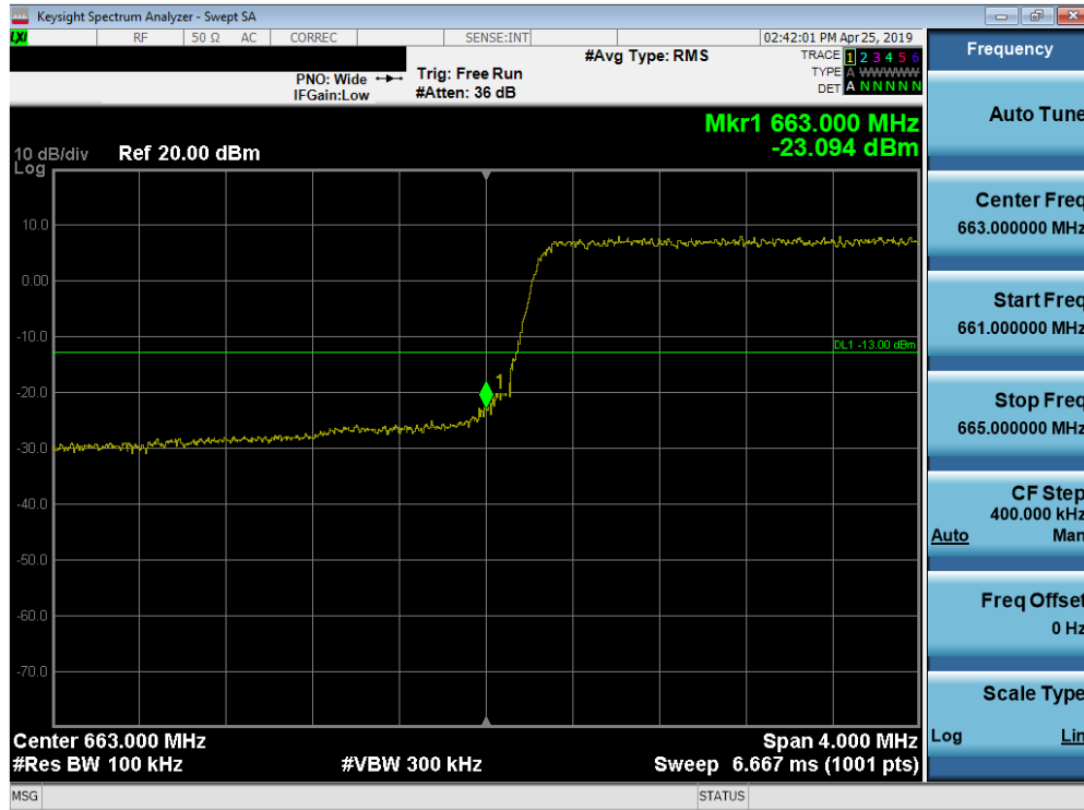
Plot 7-133. Lower Band Edge Plot (Band 71 - 5.0MHz QPSK - Full RB Configuration)
