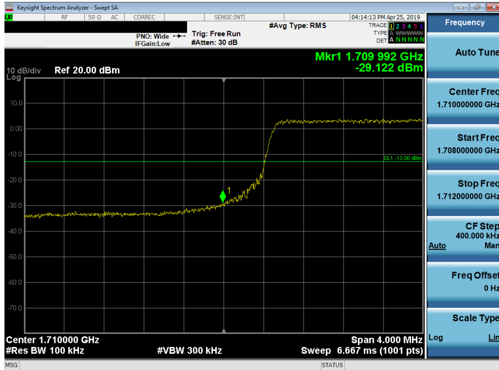
Plot 7-183. Lower Band Edge Plot (Band 66/4 - 10.0MHz QPSK - Full RB Configuration)
