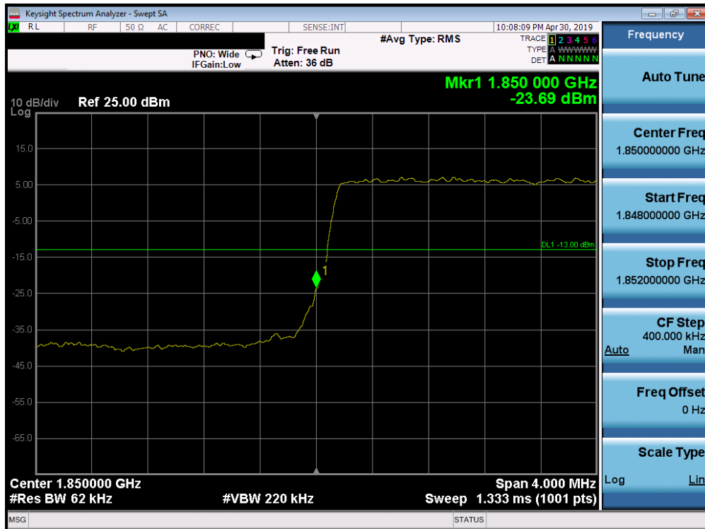
Plot 7-205. Lower Band Edge Plot (Band 2 - 3.0MHz QPSK - Full RB Configuration)
