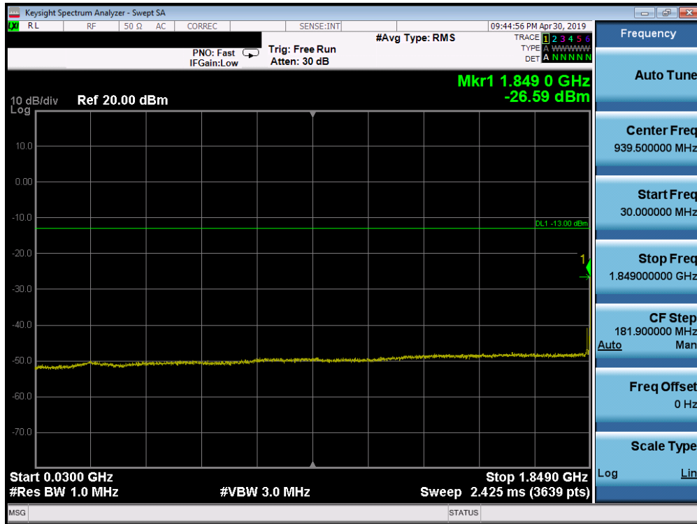
Plot 7-124. Conducted Spurious Plot (Band 2 - 15.0MHz QPSK - RB Size 1, RB Offset 0 - Low Channel)
