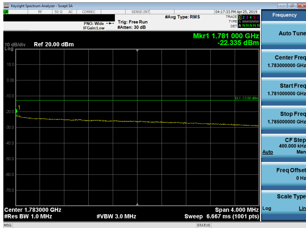
Plot 7-194. Upper Extended Band Edge Plot (Band 66 - 15.0MHz QPSK - Full RB Configuration)
