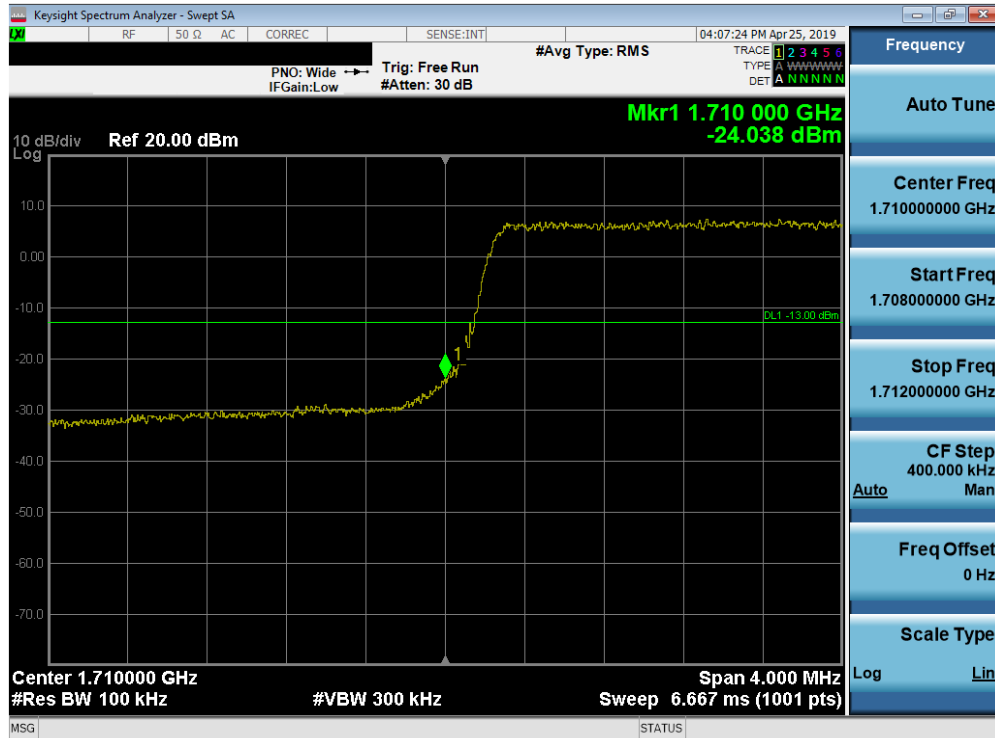
Plot 7-177. Lower Band Edge Plot (Band 66/4 - 5.0MHz QPSK - Full RB Configuration)
