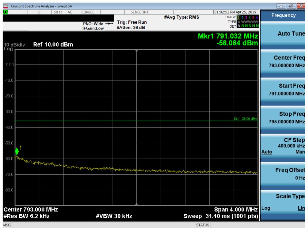
Plot 7-152. Upper Emission Mask Edge Plot (Band 13 - 5.0MHz QPSK - Full RB Configuration)
