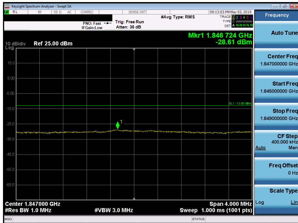
Plot 7-218. Lower Extended Band Edge Plot (Band 2 - 15MHz QPSK - Full RB Configuration)
