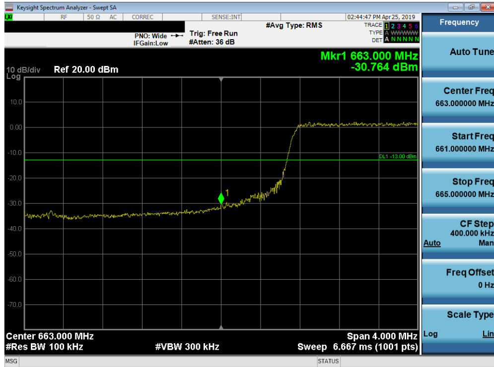
Plot 7-137. Lower Band Edge Plot (Band 71 - 15.0MHz QPSK - Full RB Configuration)
