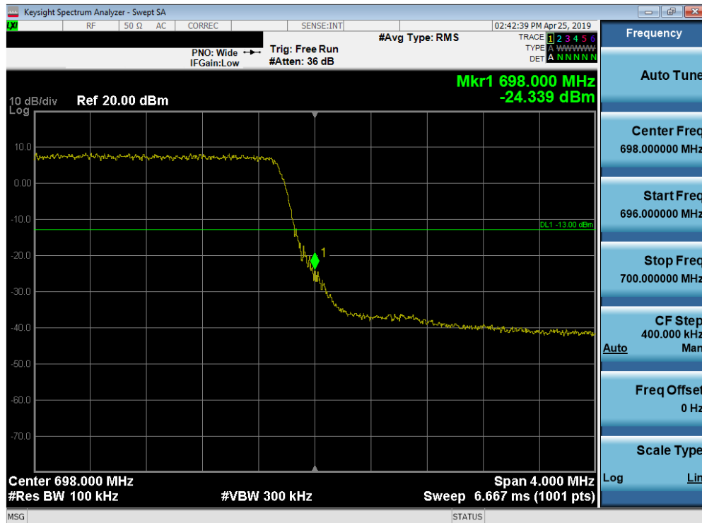
Plot 7-134. Upper Band Edge Plot (Band 71 - 5.0MHz QPSK - Full RB Configuration)
