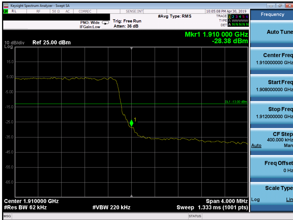
Plot 7-211. Upper Band Edge Plot (Band 2 - 5.0MHz QPSK - Full RB Configuration)
