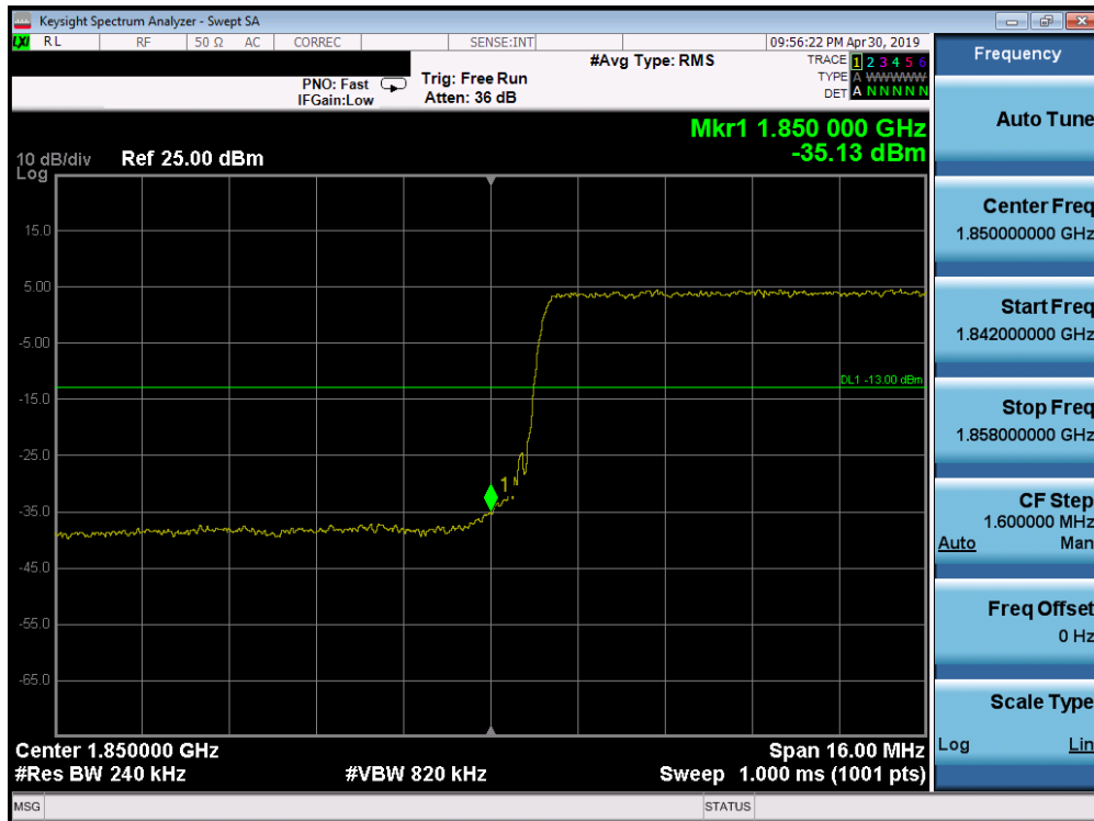
Plot 7-221. Lower Band Edge Plot (Band 2 - 20.0MHz QPSK - Full RB Configuration)
