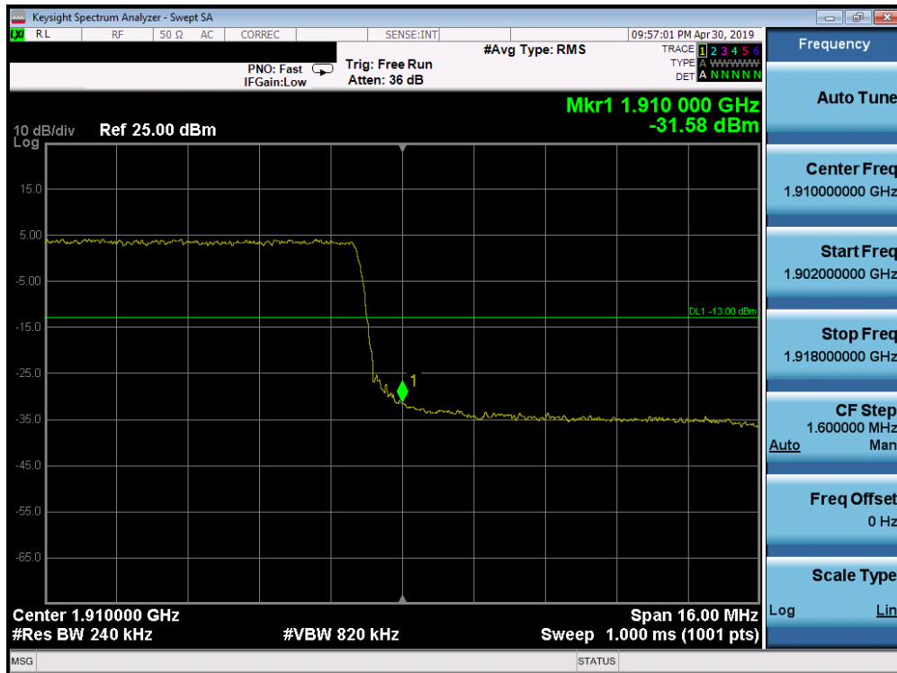
Plot 7-223. Upper Band Edge Plot (Band 2 - 20.0MHz QPSK - Full RB Configuration)
