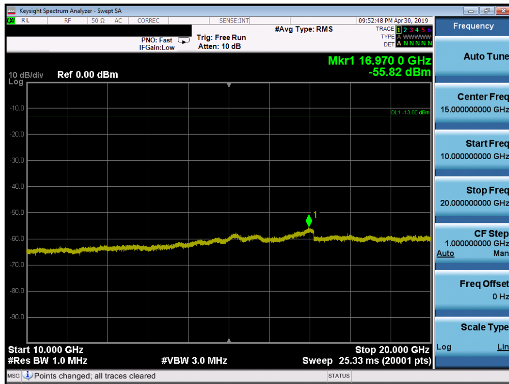
Plot 7-132. Conducted Spurious Plot (Band 2 - 15.0MHz QPSK - RB Size 1, RB Offset 0 - High Channel)
