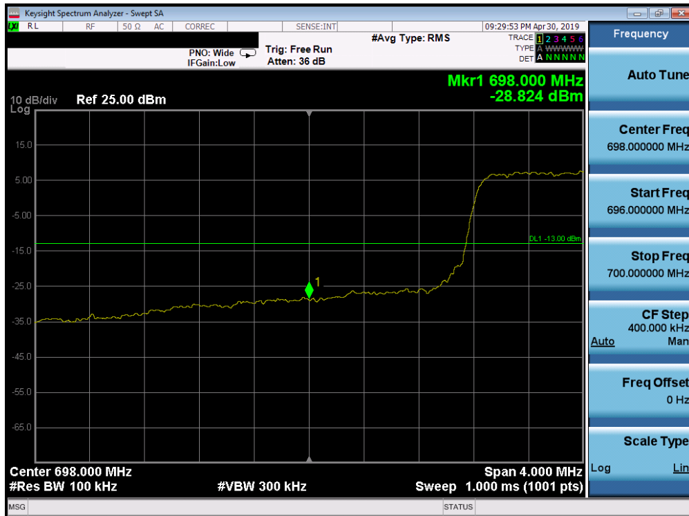
Plot 7-145. Lower Band Edge Plot (Band 12 - 5.0MHz QPSK - Full RB Configuration)
