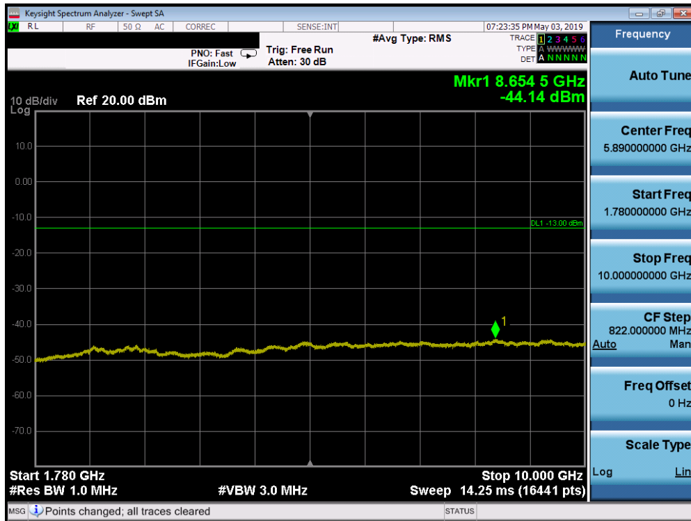
Plot 7-119. Conducted Spurious Plot (Band 66/4 - 20.0MHz QPSK - RB Size 1, RB Offset 0 - Mid Channel)
