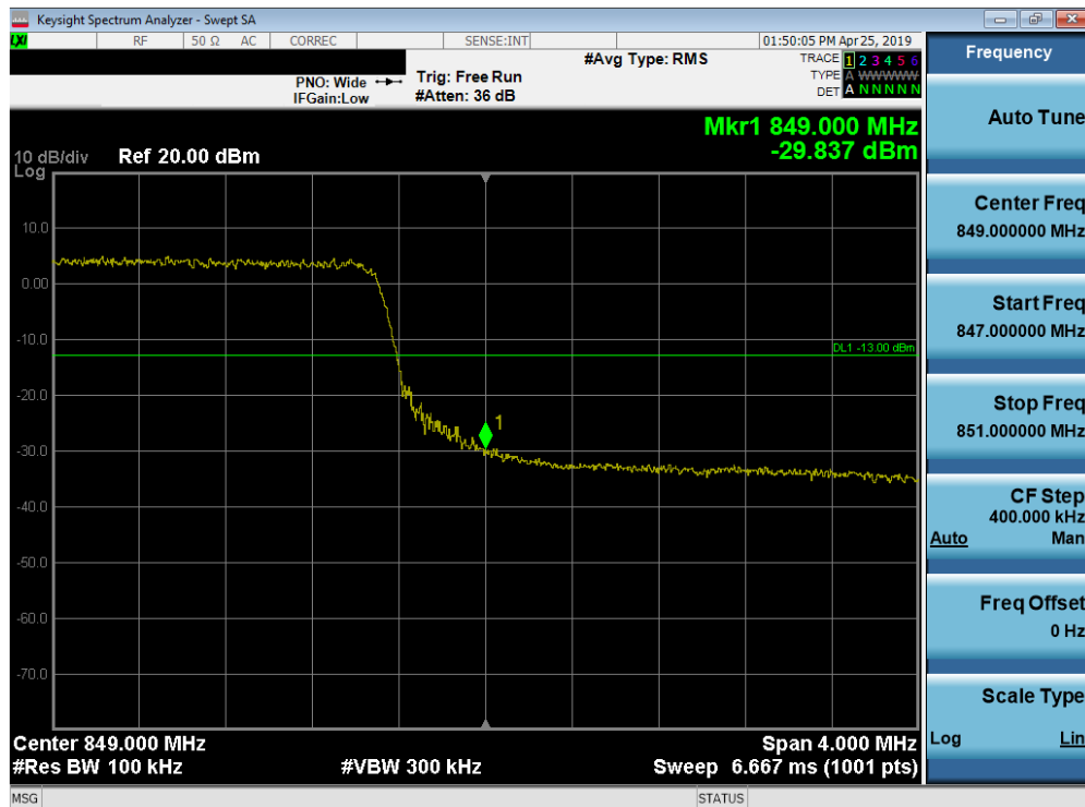
Plot 7-164. Upper Band Edge Plot (Band 5 - 10.0MHz QPSK - Full RB Configuration)
