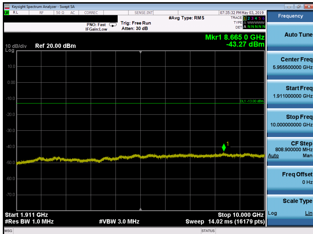
Plot 7-131. Conducted Spurious Plot (Band 2 - 15.0MHz QPSK - RB Size 1, RB Offset 0 - High Channel)
