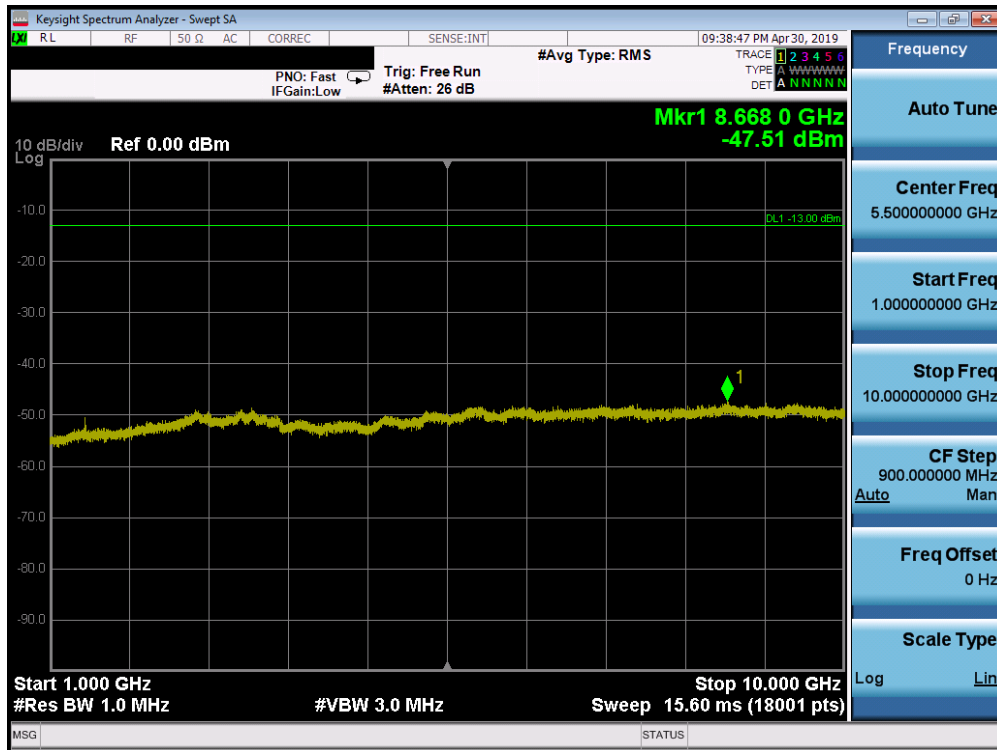
Plot 7-90. Conducted Spurious Plot (Band 12 - 3.0MHz QPSK - RB Size 1, RB Offset 0 - Low Channel)
