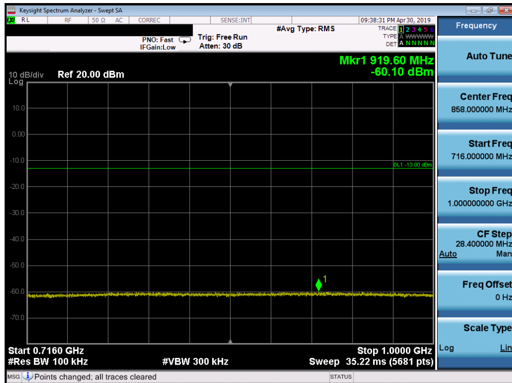
Plot 7-89. Conducted Spurious Plot (Band 12 - 3.0MHz QPSK - RB Size 1, RB Offset 0 - Low Channel)
