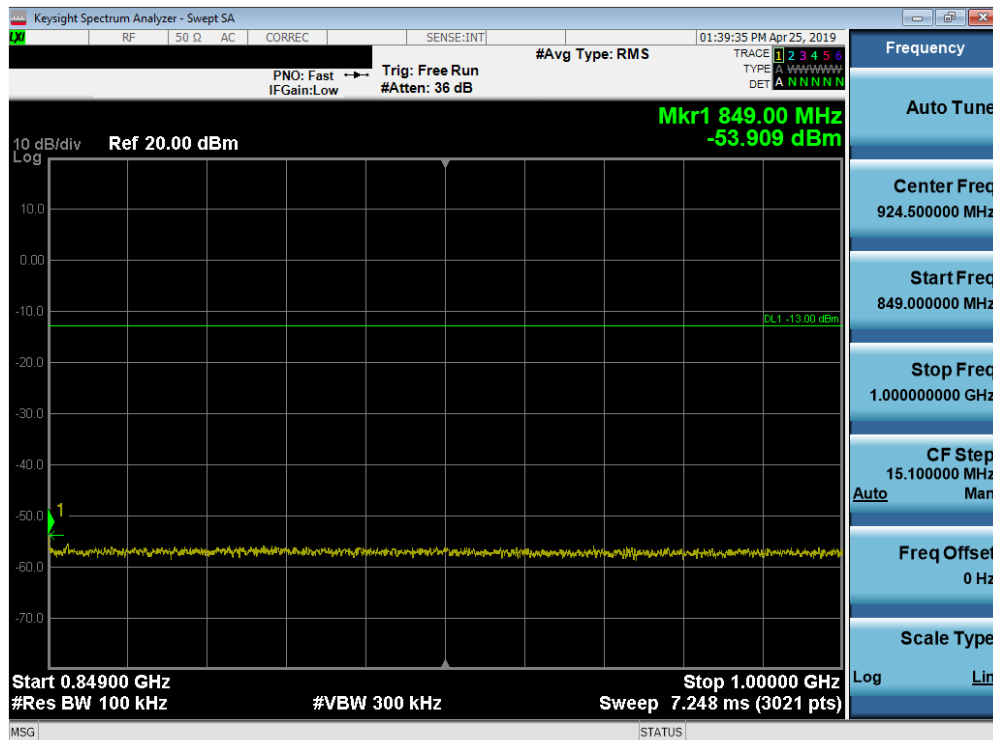
Plot 7-113. Conducted Spurious Plot (Band 5 - 10.0MHz QPSK - RB Size 1, RB Offset 0 - High Channel)
