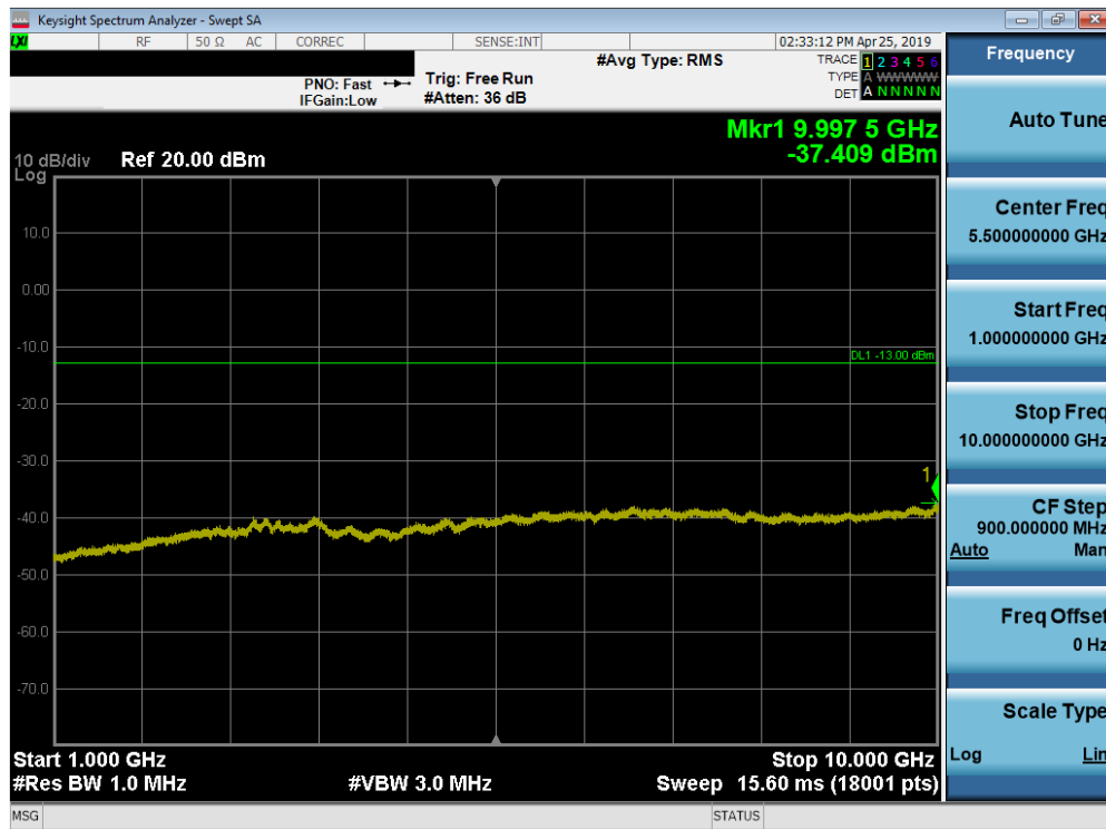
Plot 7-81. Conducted Spurious Plot (Band 71 - 15.0MHz QPSK - RB Size 1, RB Offset 0 - Low Channel)
