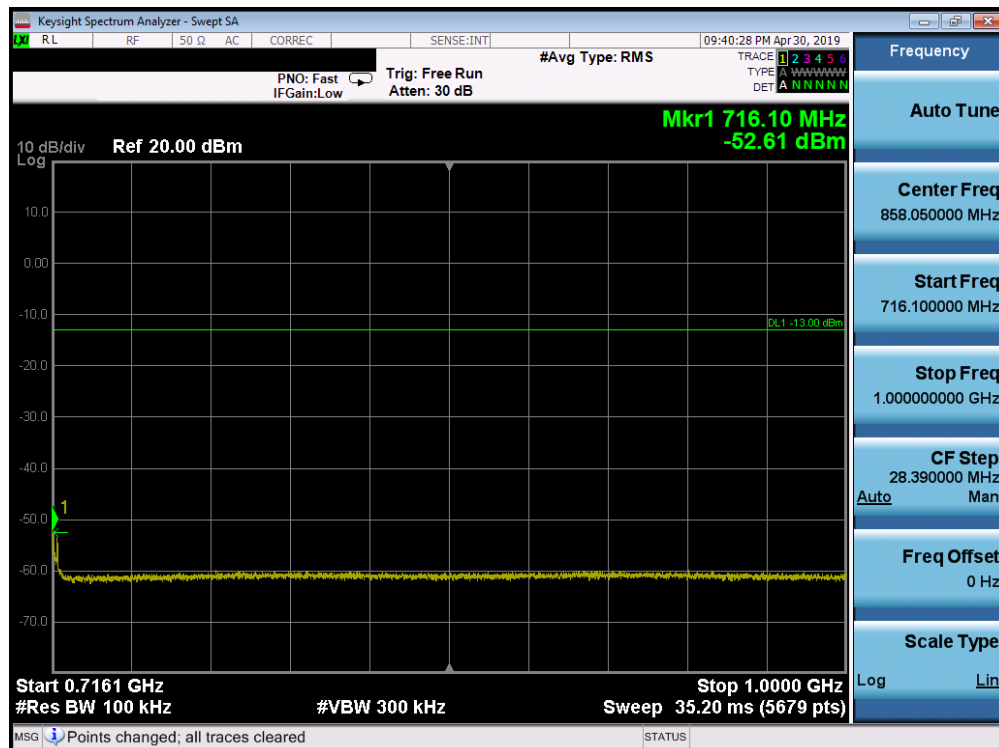
Plot 7-95. Conducted Spurious Plot (Band 12 - 3.0MHz QPSK - RB Size 1, RB Offset 0 - High Channel)
