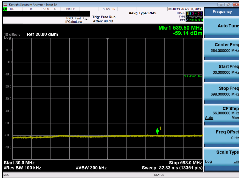
Plot 7-94. Conducted Spurious Plot (Band 12 - 3.0MHz QPSK - RB Size 1, RB Offset 0 - High Channel)
