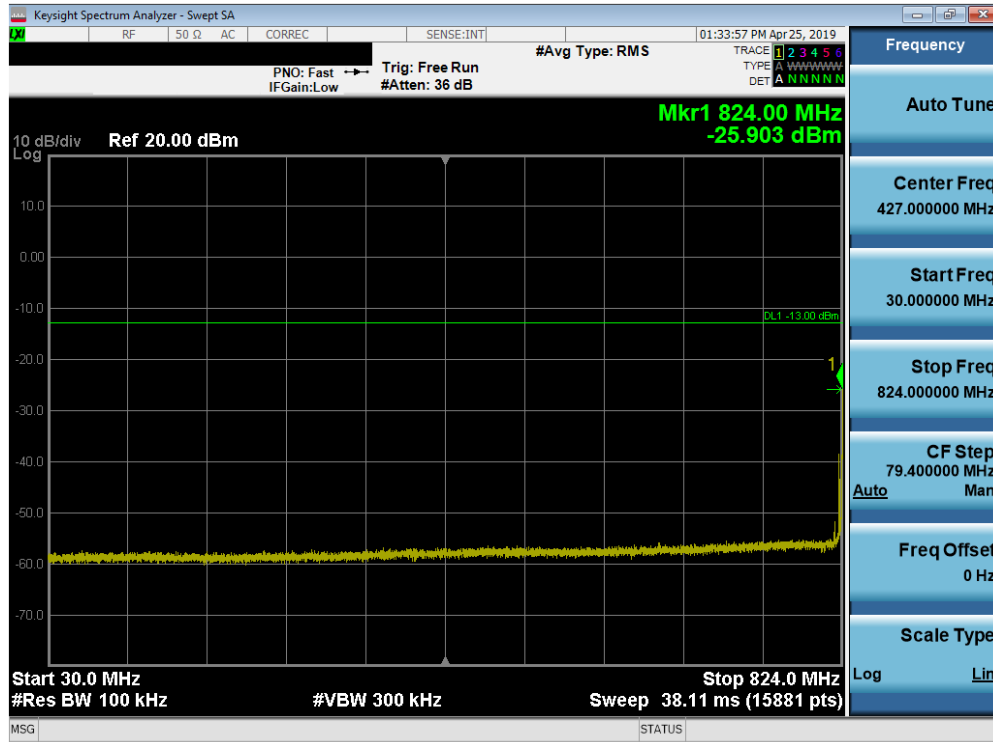
Plot 7-106. Conducted Spurious Plot (Band 5 - 10.0MHz QPSK - RB Size 1, RB Offset 0 - Low Channel)
