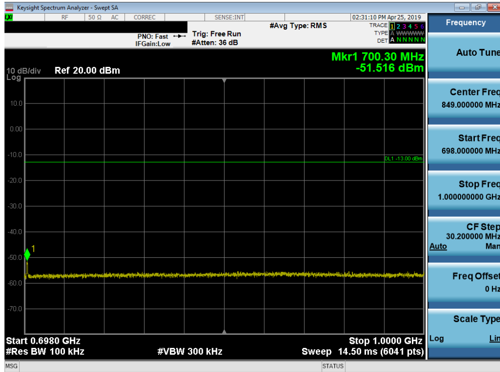
Plot 7-83. Conducted Spurious Plot (Band 71 - 15.0MHz QPSK - RB Size 1, RB Offset 0 - Mid Channel)
