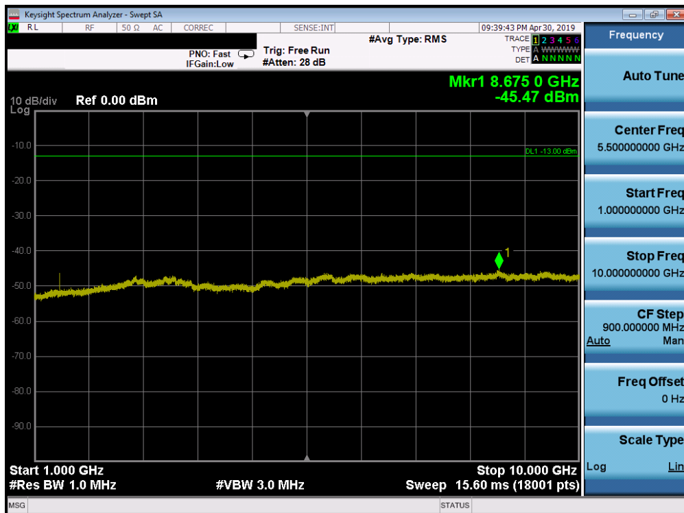
Plot 7-93. Conducted Spurious Plot (Band 12 - 3.0MHz QPSK - RB Size 1, RB Offset 0 - Mid Channel)
