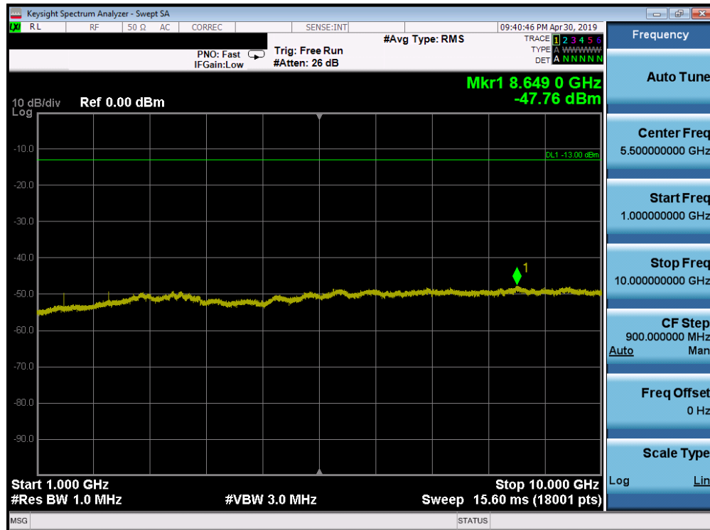
Plot 7-96. Conducted Spurious Plot (Band 12 - 3.0MHz QPSK - RB Size 1, RB Offset 0 - High Channel)
