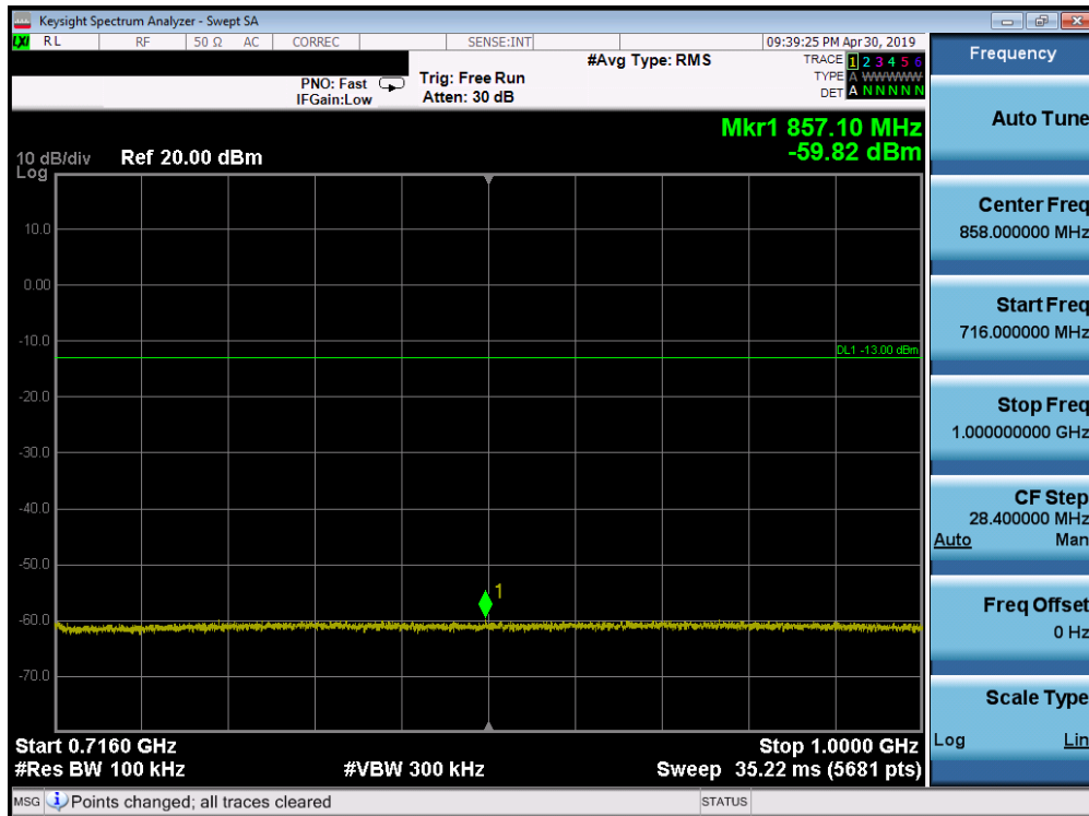
Plot 7-92. Conducted Spurious Plot (Band 12 - 3.0MHz QPSK - RB Size 1, RB Offset 0 - Mid Channel)
