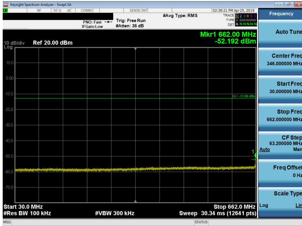
Plot 7-79. Conducted Spurious Plot (Band 71 - 15.0MHz QPSK - RB Size 1, RB Offset 0 - Low Channel)
