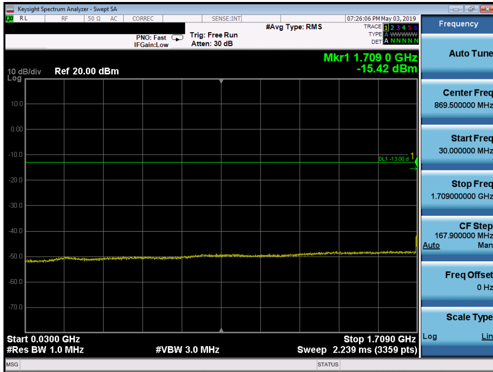
Plot 7-115. Conducted Spurious Plot (Band 66/4 - 20.0MHz QPSK - RB Size 1, RB Offset 0 - Low Channel)
