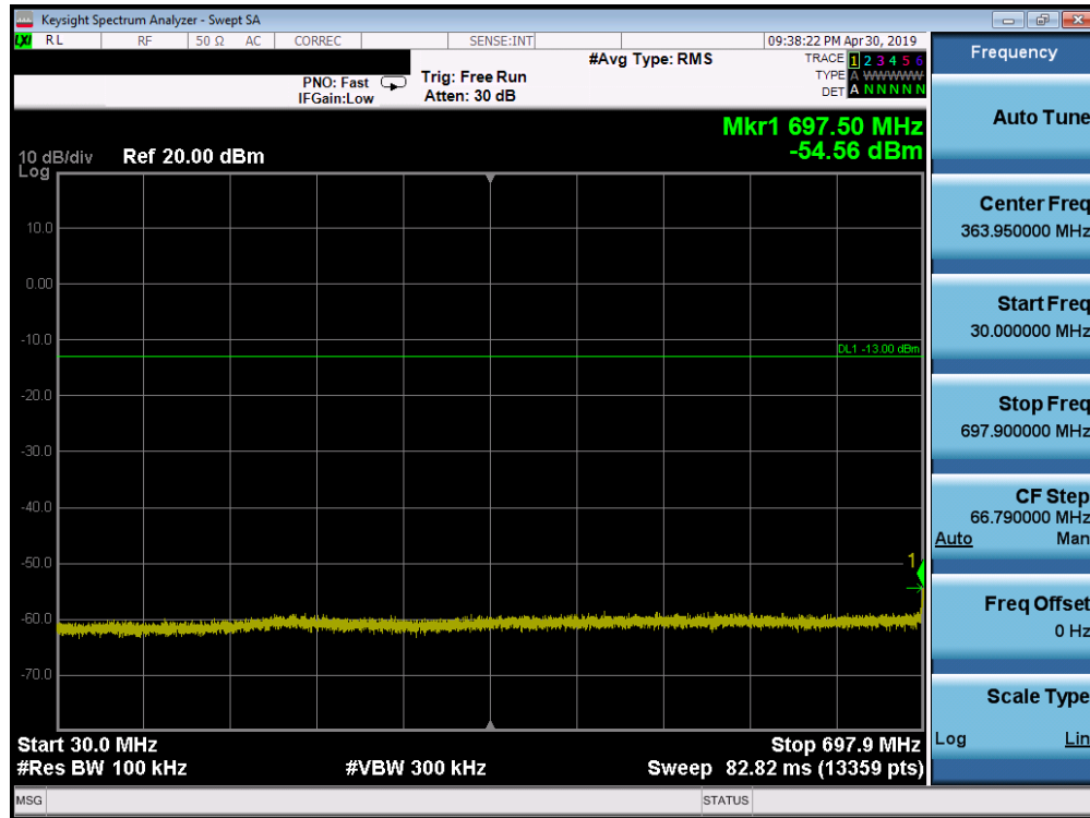
Plot 7-88. Conducted Spurious Plot (Band 12 - 3.0MHz QPSK - RB Size 1, RB Offset 0 - Low Channel)
