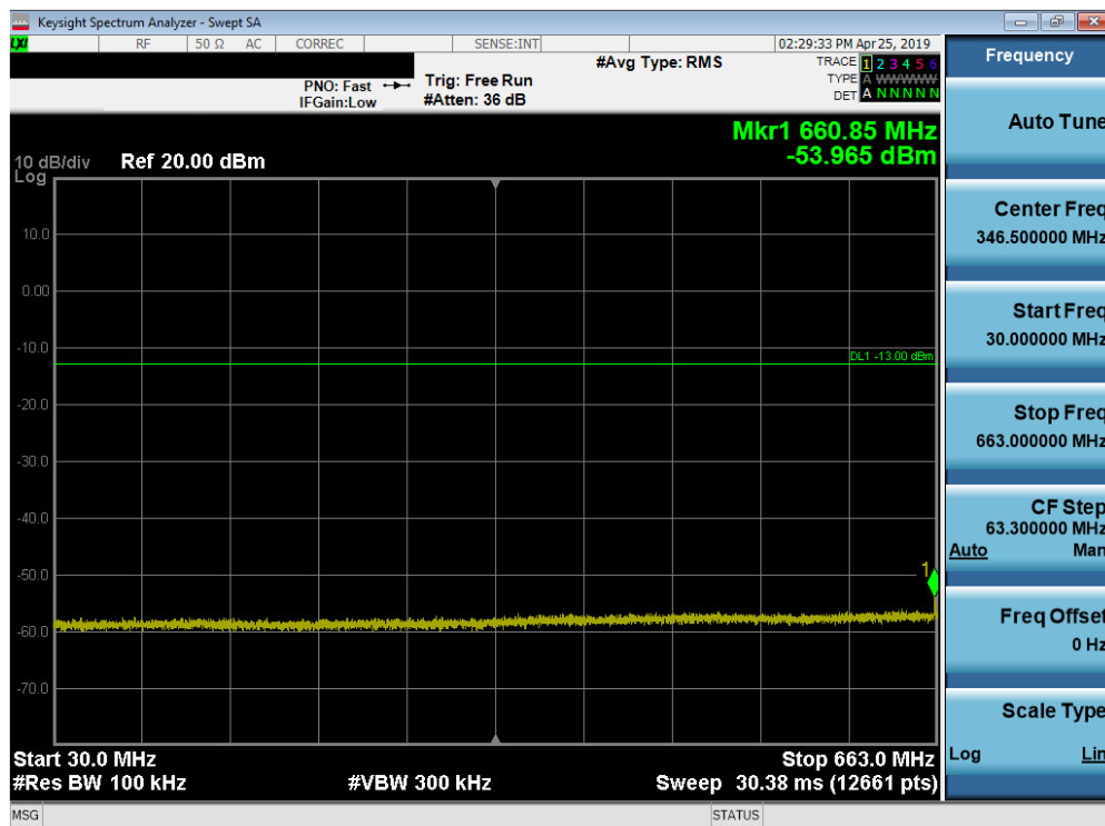
Plot 7-82. Conducted Spurious Plot (Band 71 - 15.0MHz QPSK - RB Size 1, RB Offset 0 - Mid Channel)
