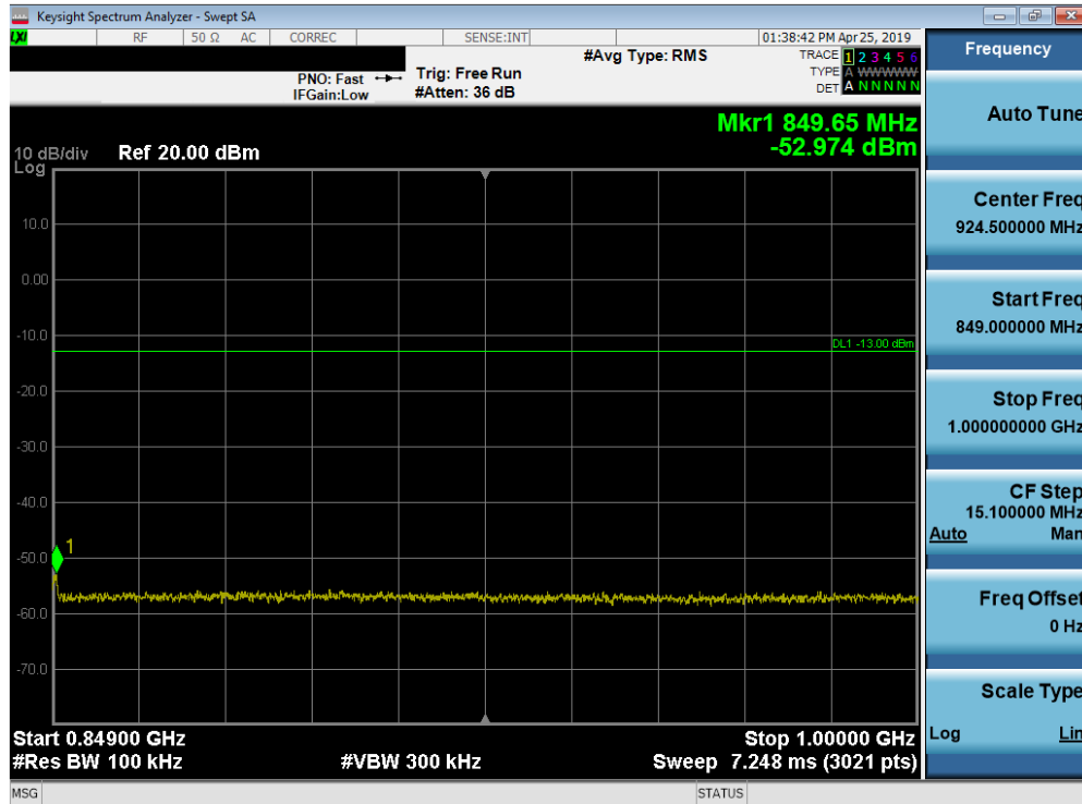
Plot 7-110. Conducted Spurious Plot (Band 5 - 10.0MHz QPSK - RB Size 1, RB Offset 0 - Mid Channel)
