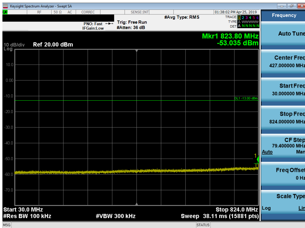
Plot 7-109. Conducted Spurious Plot (Band 5 - 10.0MHz QPSK - RB Size 1, RB Offset 0 - Mid Channel)
