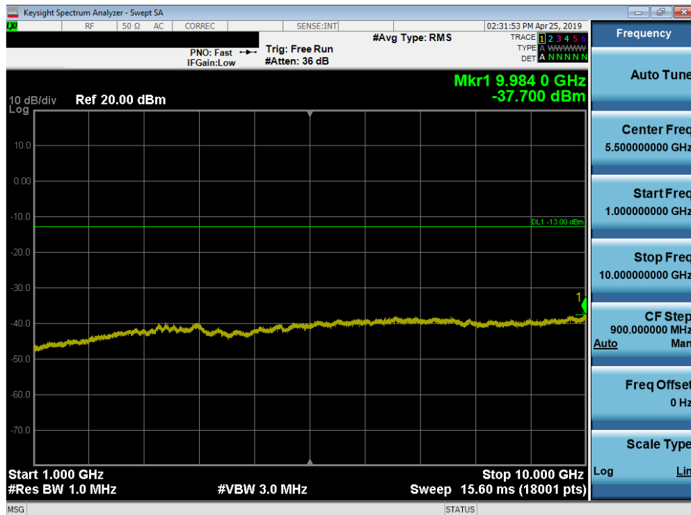
Plot 7-84. Conducted Spurious Plot (Band 71 - 15.0MHz QPSK - RB Size 1, RB Offset 0 - Mid Channel)
