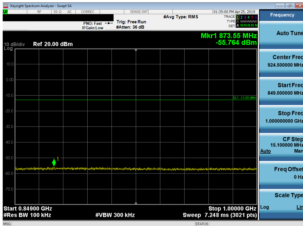
Plot 7-107. Conducted Spurious Plot (Band 5 - 10.0MHz QPSK - RB Size 1, RB Offset 0 - Low Channel)
