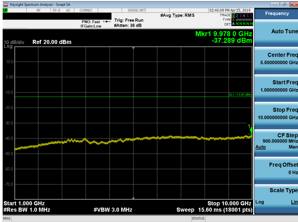
Plot 7-87. Conducted Spurious Plot (Band 71 - 15.0MHz QPSK - RB Size 1, RB Offset 0 - High Channel)
