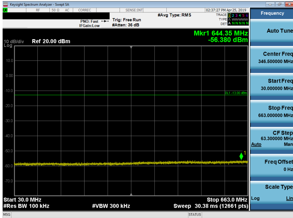
Plot 7-85. Conducted Spurious Plot (Band 71 - 15.0MHz QPSK - RB Size 1, RB Offset 0 - High Channel)
