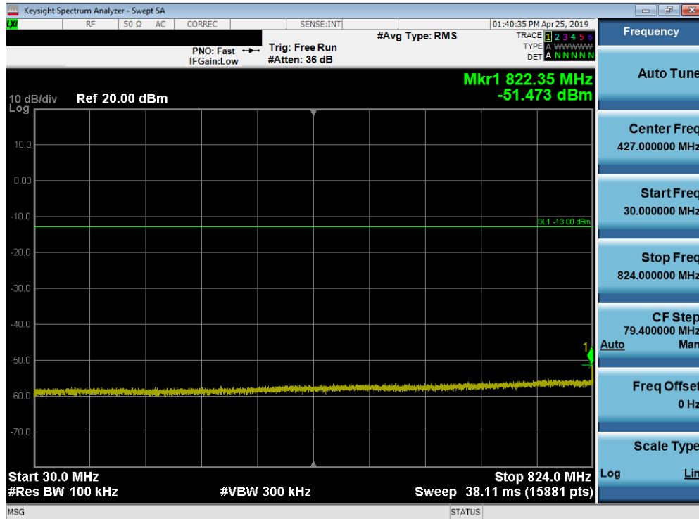
Plot 7-112. Conducted Spurious Plot (Band 5 - 10.0MHz QPSK - RB Size 1, RB Offset 0 - High Channel)
