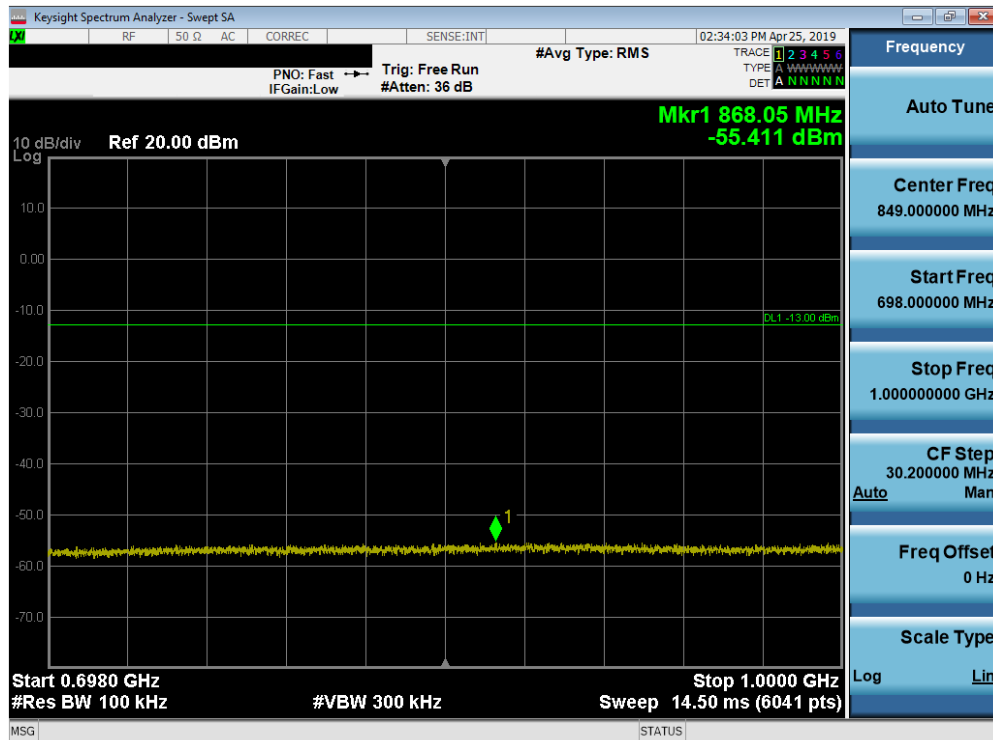
Plot 7-80. Conducted Spurious Plot (Band 71 - 15.0MHz QPSK - RB Size 1, RB Offset 0 - Low Channel)
