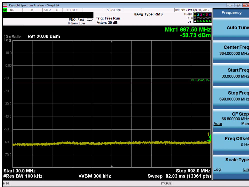
Plot 7-91. Conducted Spurious Plot (Band 12 - 3.0MHz QPSK - RB Size 1, RB Offset 0 - Mid Channel)
