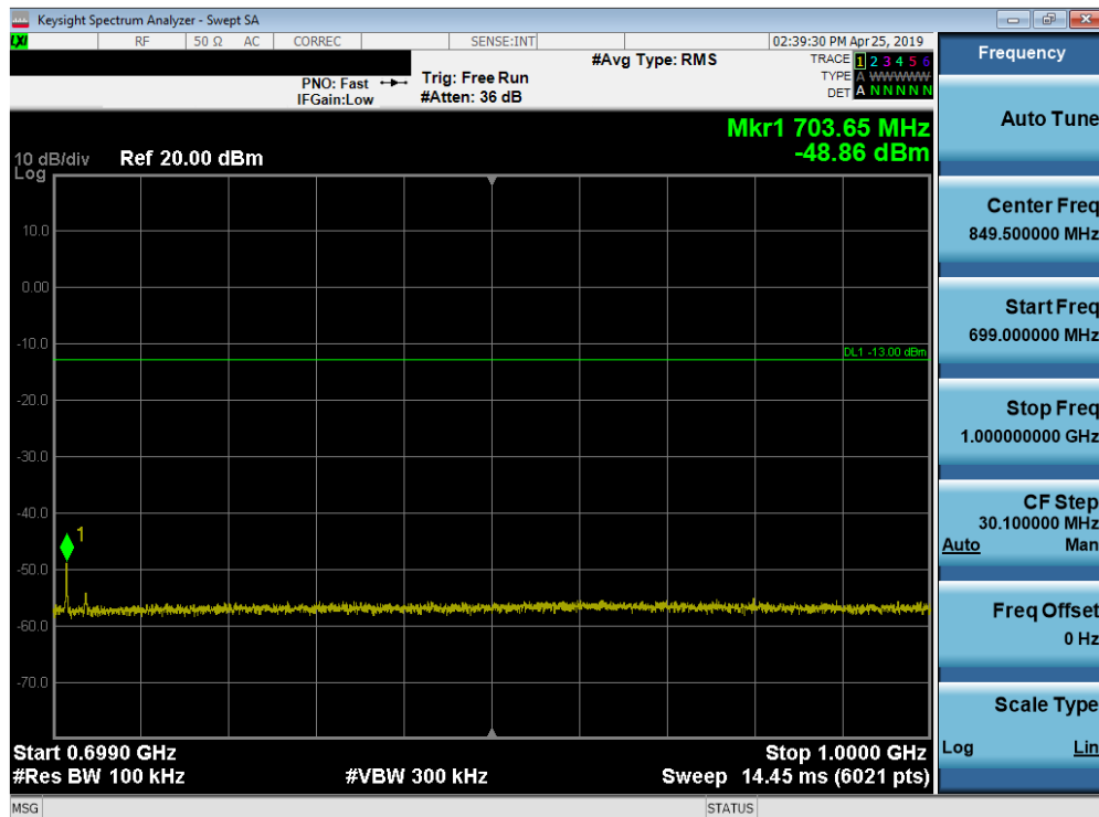
Plot 7-86. Conducted Spurious Plot (Band 71 - 15.0MHz QPSK - RB Size 1, RB Offset 0 - High Channel)
