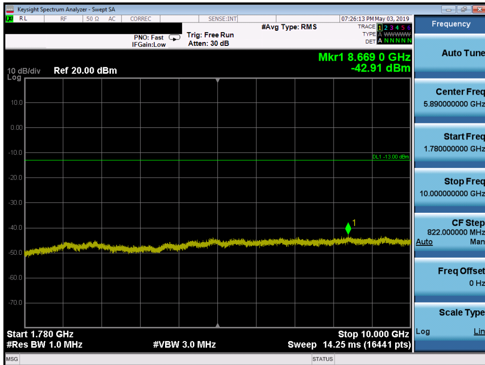
Plot 7-116. Conducted Spurious Plot (Band 66/4 - 20.0MHz QPSK - RB Size 1, RB Offset 0 - Low Channel)
