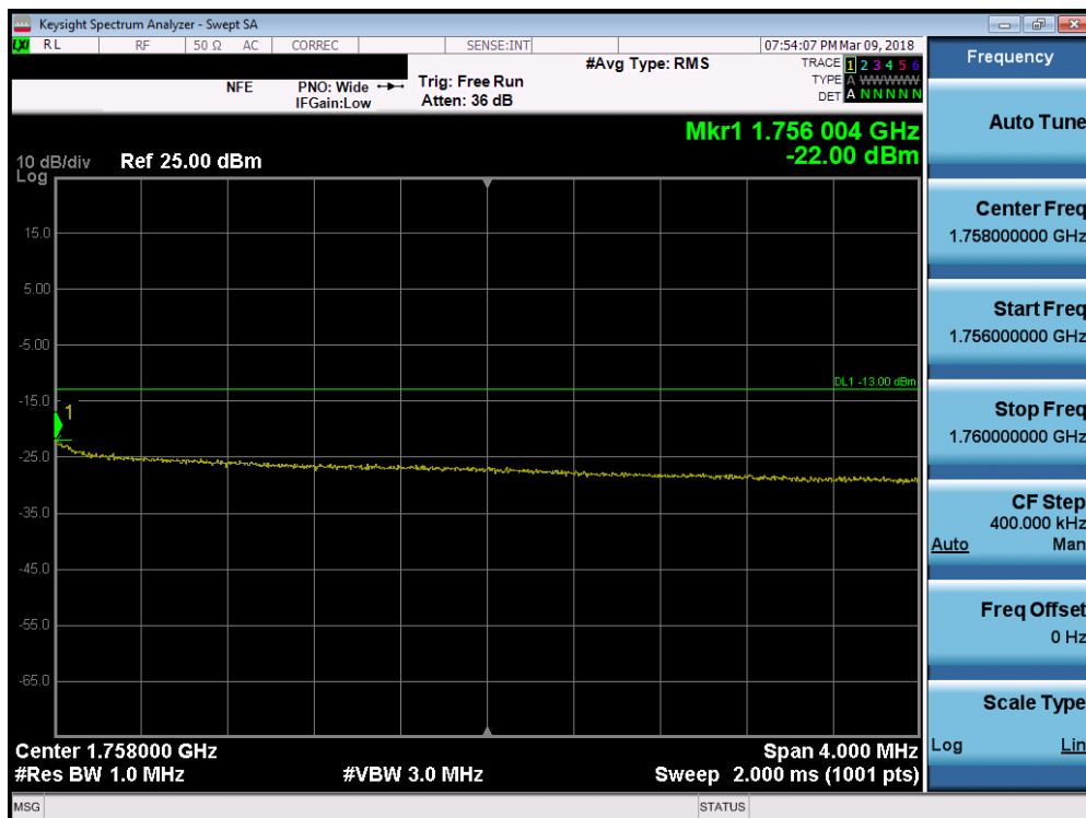
Plot 7-189. Upper Extended Band Edge Plot (Band 4 - 10.0MHz QPSK - Full RB Configuration)
