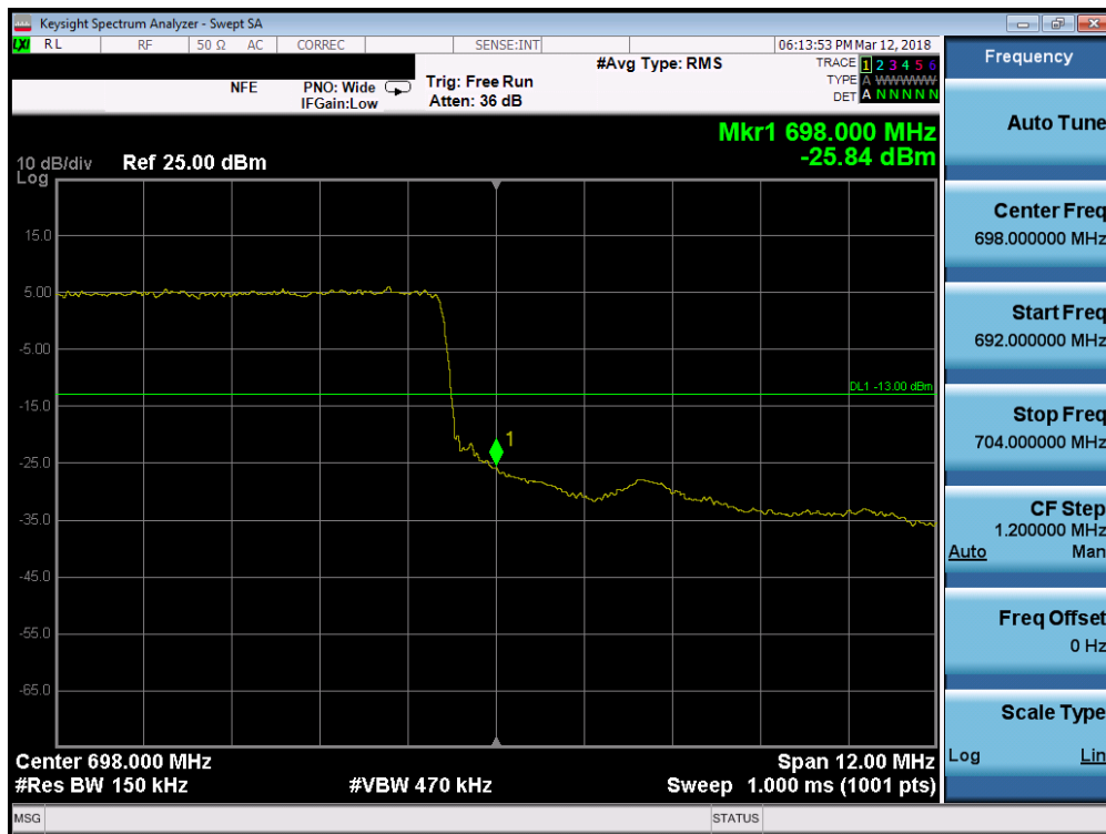
Plot 7-141. Upper Band Edge Plot (Band 71 - 15.0MHz QPSK - Full RB Configuration)
