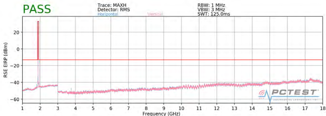
Plot 7-110. Radiated Spurious Plot above 1GHz (PCS GRPS Mode)
