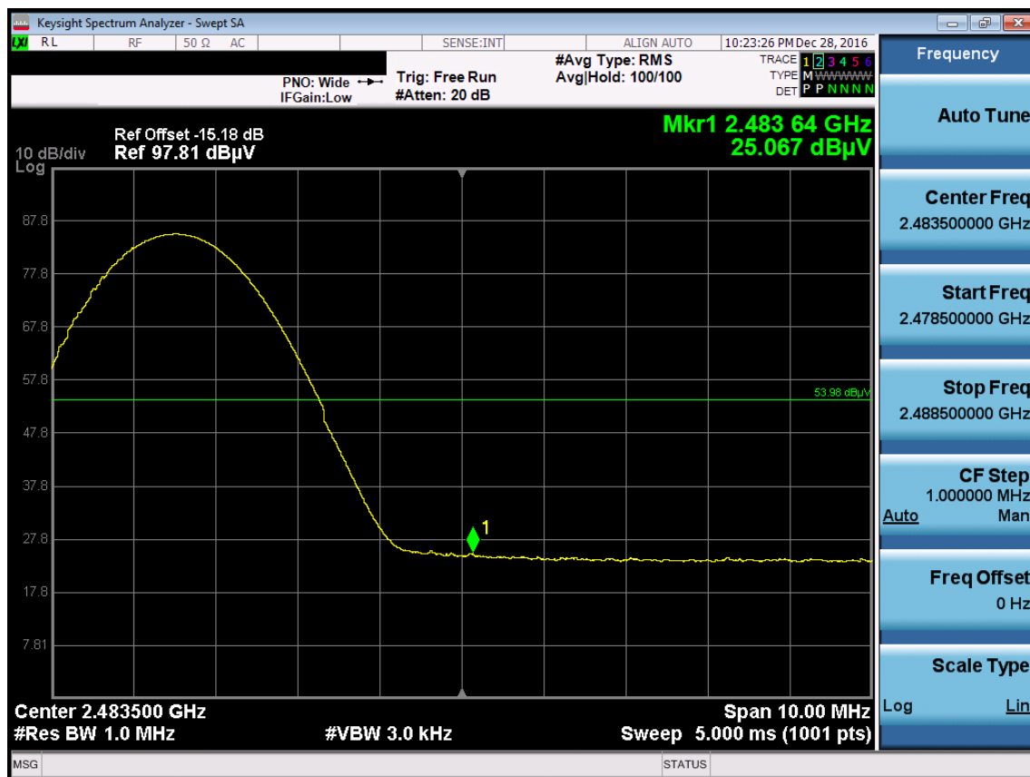
Plot 7-9. Radiated Restricted Upper Band Edge Measurement (Average)
