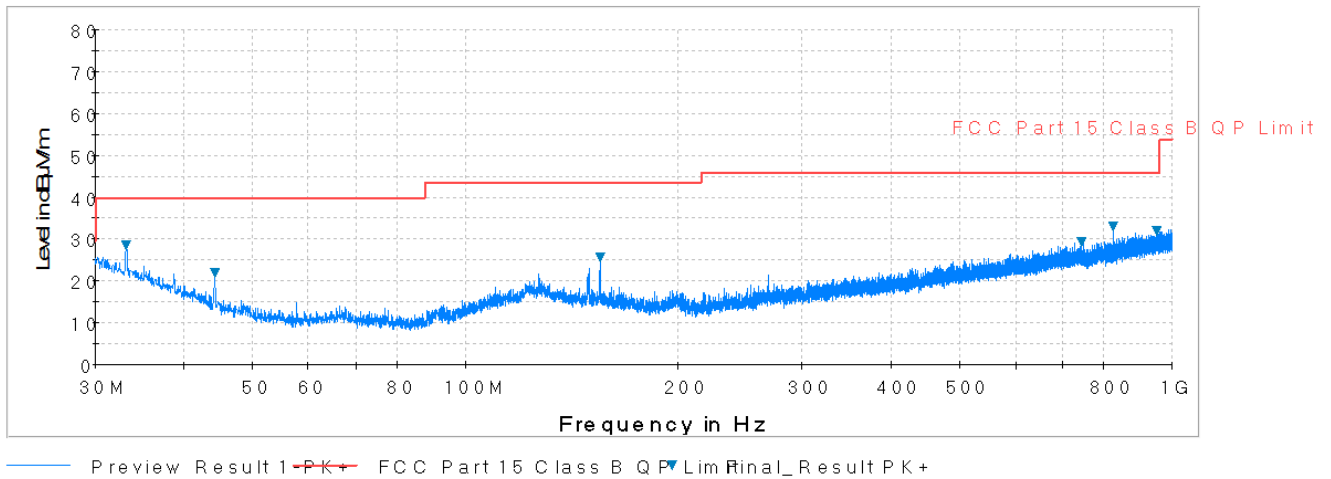
Plot 7-12. Radiated Spurious Plot below 1GHz (Pol. V)
