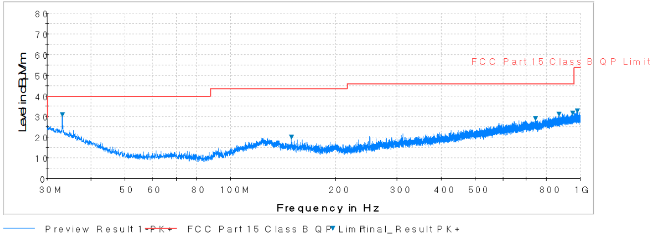
Plot 7-11. Radiated Spurious Plot below 1GHz (Pol. H)
