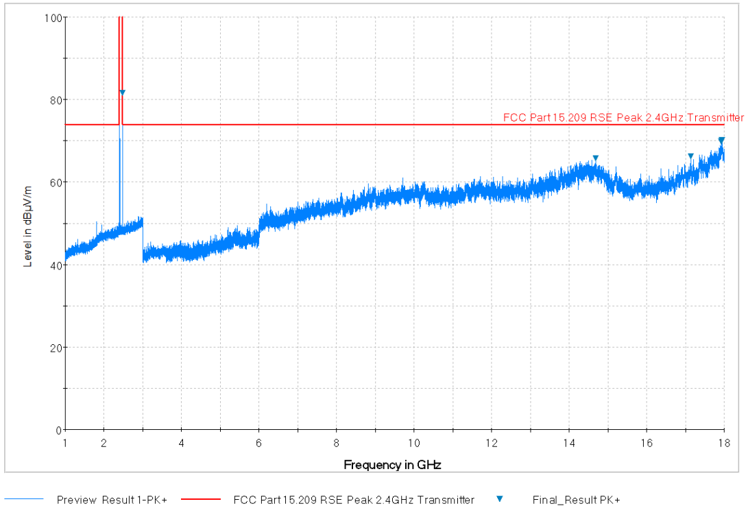
Plot 7-42. Radiated Spurious Plot above 1GHz (BT – Ch. 0, Ant. Pol. H)
