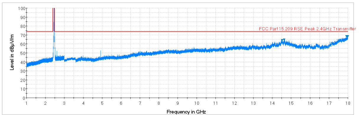
Plot 7-5. Radiated Spurious Plot above 1GHz (802.11b – Ch. 11, Ant. Pol. H)
