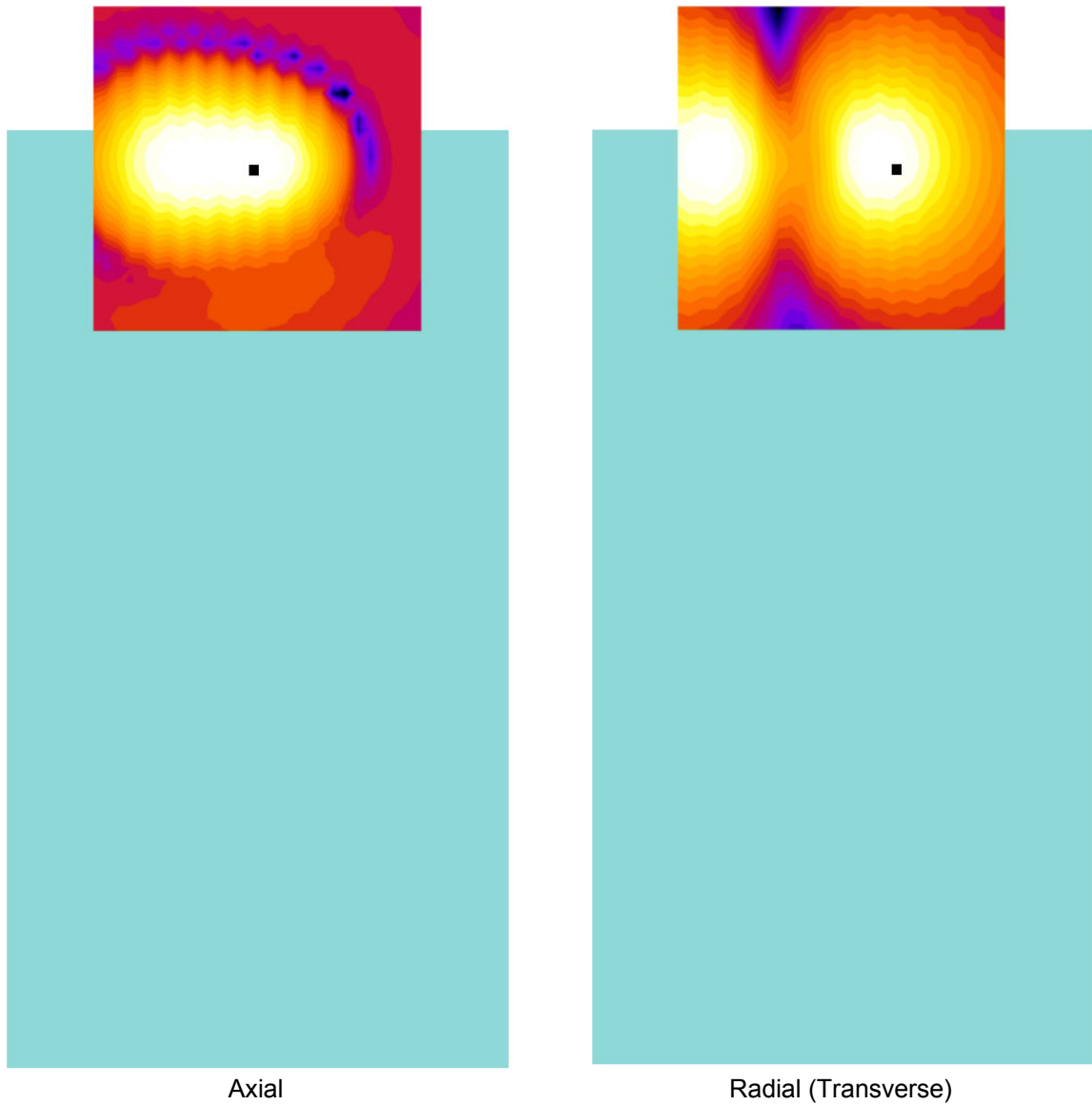
Figure 6-1 T-Coil Scan Overlay Magnetic Field Distributions
