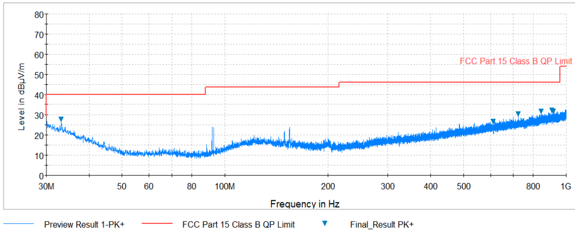
Plot 7-16. Radiated Spurious Plot below 1GHz (Pol. V)
