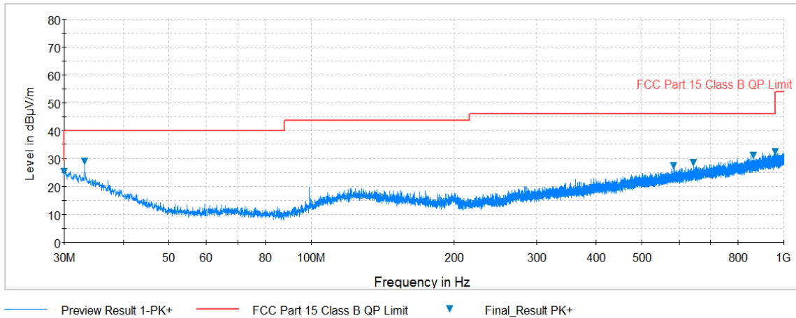
Plot 7-15. Radiated Spurious Plot below 1GHz (Pol. H)
