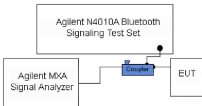
Figure 9-3 Power Measurement Setup
