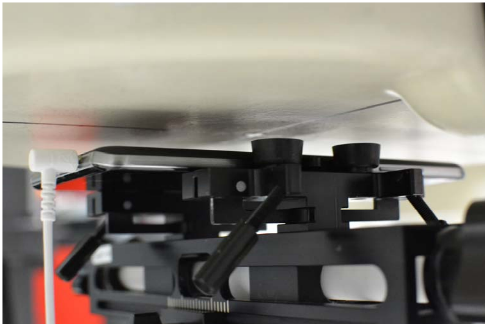
SAR Test Setup Photo 6 – Back Side with Headphones at 1.0 cm
