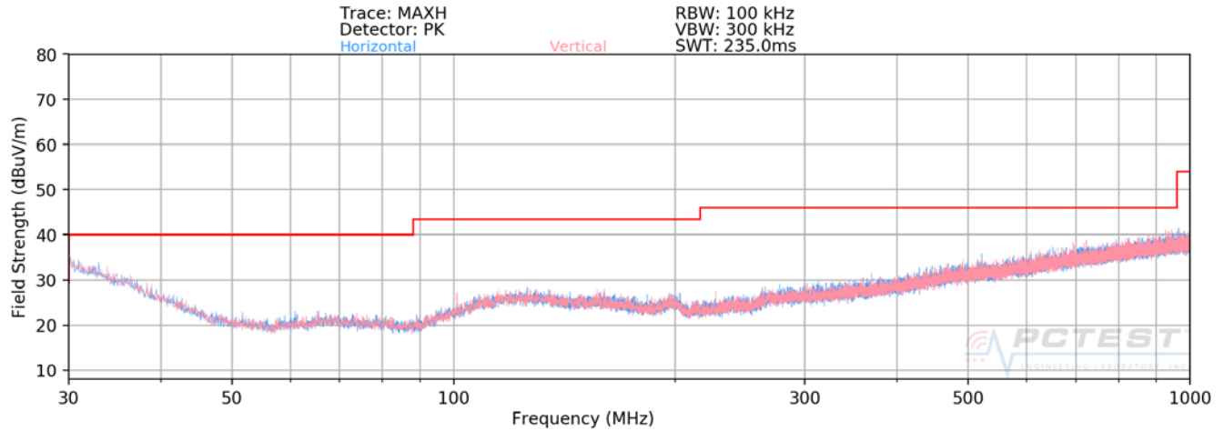
Plot 7-3. Radiated Spurious Plot below 1GHz
