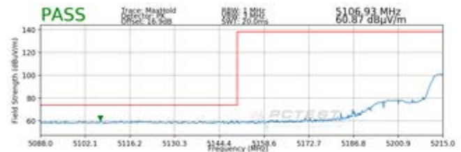
Plot 7-24. Radiated Lower Band Edge Plot (Peak – UNII Band 1)
