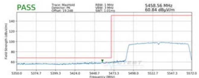
Plot 7-40. Radiated Lower Band Edge Plot (Peak – UNII Band 2C)
