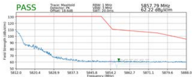
Plot 7-19. Radiated Upper Band Edge Plot (Peak – UNII Band 3)
