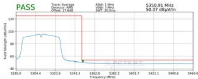
Plot 7-27. Radiated Upper Band Edge Plot (Average – UNII Band 2A)
