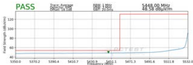
Plot 7-31. Radiated Lower Band Edge Plot (Average – UNII Band 2C)
