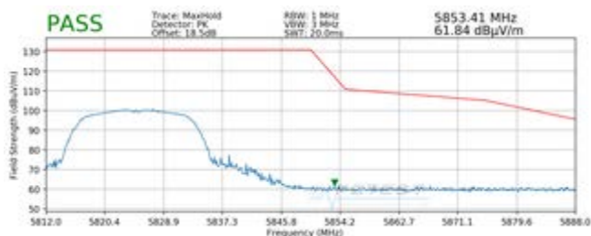
Plot 7-20. Radiated Upper Band Edge Plot (Peak – UNII Band 3)
