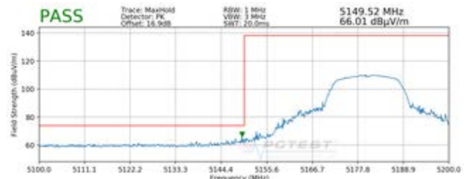
Plot 7-8. Radiated Lower Band Edge Plot (Peak – UNII Band 1)
