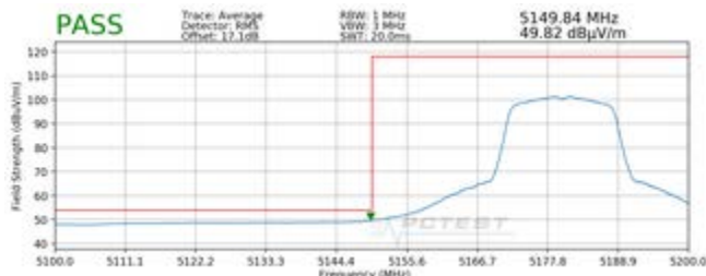
Plot 7-7. Radiated Lower Band Edge Plot (Average – UNII Band 1)
