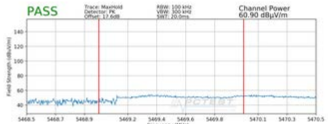
Plot 7-30. Radiated Lower Band Edge Plot (Peak – UNII Band 2C)
