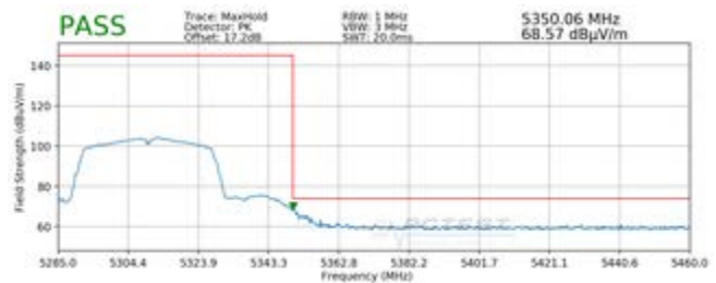
Plot 7-28. Radiated Upper Band Edge Plot (Peak – UNII Band 2A)
