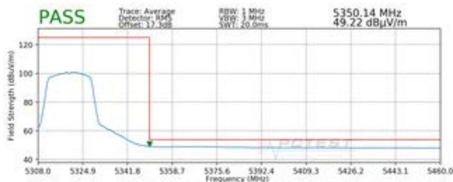
Plot 7-13. Radiated Upper Band Edge Plot (Average – UNII Band 2A)
