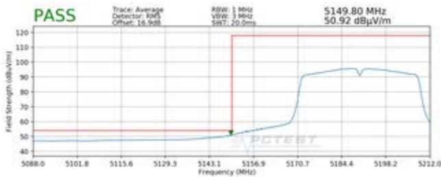
Plot 7-21. Radiated Lower Band Edge Plot (Average – UNII Band 1)
