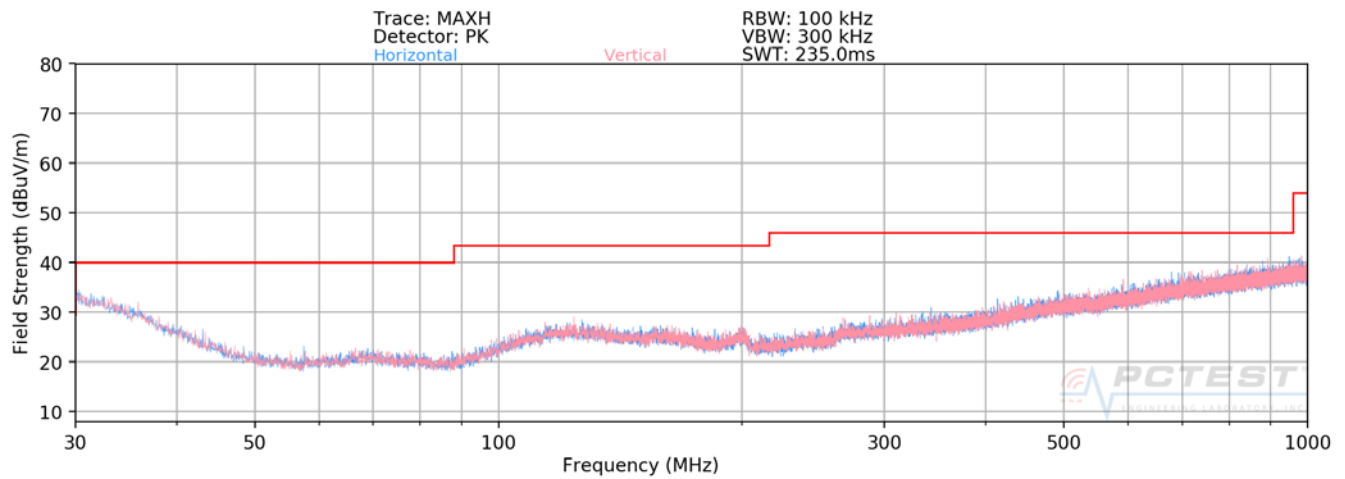
Plot 7-42. Radiated Spurious Plot below 1GHz (802.11a – U3 Ch. 157)
