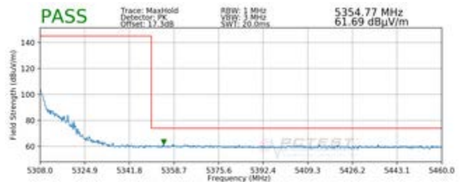
Plot 7-12. Radiated Upper Band Edge Plot (Peak – UNII Band 2A)
