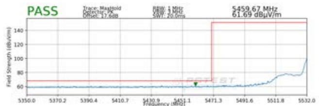
Plot 7-32. Radiated Lower Band Edge Plot (Peak – UNII Band 2C)
