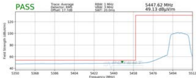
Plot 7-15. Radiated Lower Band Edge Plot (Average – UNII Band 2C)
