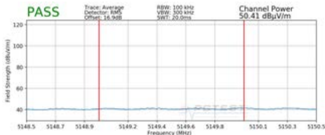
Plot 7-35. Radiated Lower Band Edge Plot (Average – UNII Band 1)
