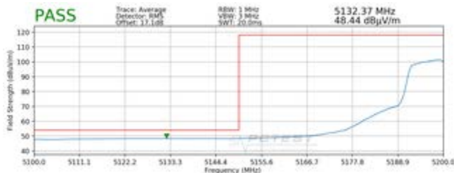
Plot 7-9. Radiated Lower Band Edge Plot (Average – UNII Band 1)
