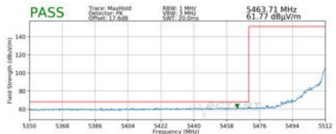
Plot 7-18. Radiated Lower Band Edge Plot (Peak – UNII Band 2C)
