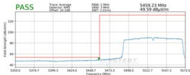
Plot 7-39. Radiated Lower Band Edge Plot (Average – UNII Band 2C)
