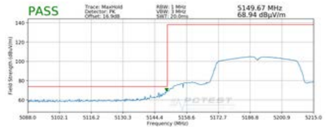
Plot 7-22. Radiated Lower Band Edge Plot (Peak – UNII Band 1)
