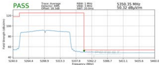
Plot 7-37. Radiated Upper Band Edge Plot (Average – UNII Band 2A)
