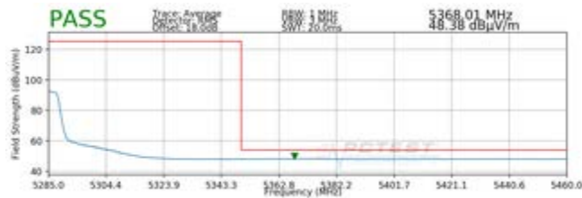
Plot 7-25. Radiated Upper Band Edge Plot (Average – UNII Band 2A)
