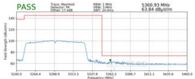
Plot 7-38. Radiated Upper Band Edge Plot (Peak – UNII Band 2A)
