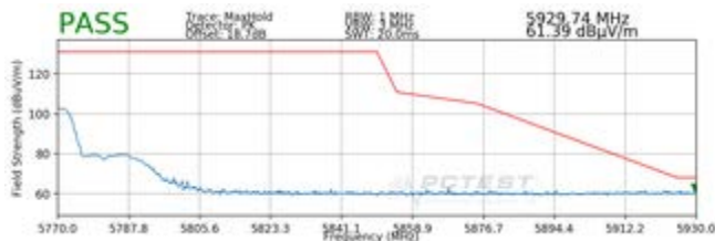
Plot 7-33. Radiated Upper Band Edge Plot (Peak – UNII Band 3)
