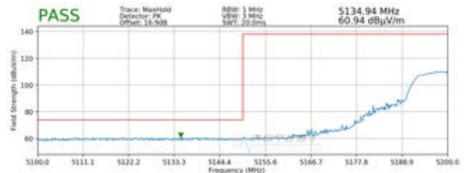
Plot 7-10. Radiated Lower Band Edge Plot (Peak – UNII Band 1)
