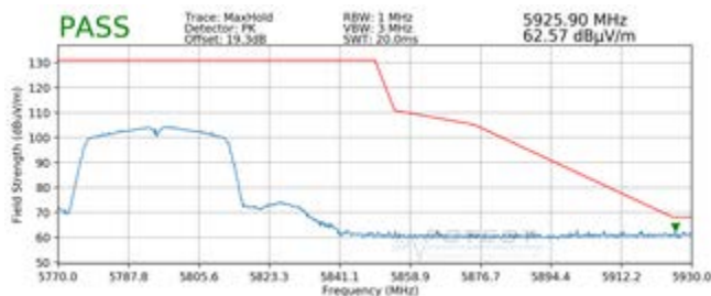
Plot 7-34. Radiated Upper Band Edge Plot (Peak – UNII Band 3)
