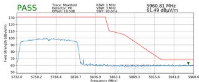
Plot 7-41. Radiated Upper Band Edge Plot (Peak – UNII Band 3)
