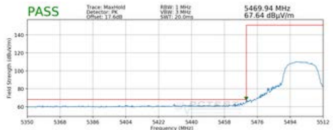
Plot 7-16. Radiated Lower Band Edge Plot (Peak – UNII Band 2C)
