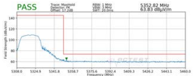
Plot 7-14. Radiated Upper Band Edge Plot (Peak – UNII Band 2A)
