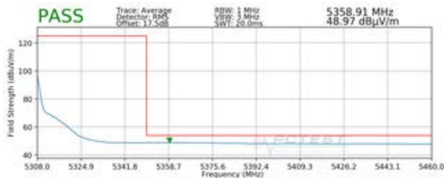
Plot 7-11. Radiated Upper Band Edge Plot (Average – UNII Band 2A)
