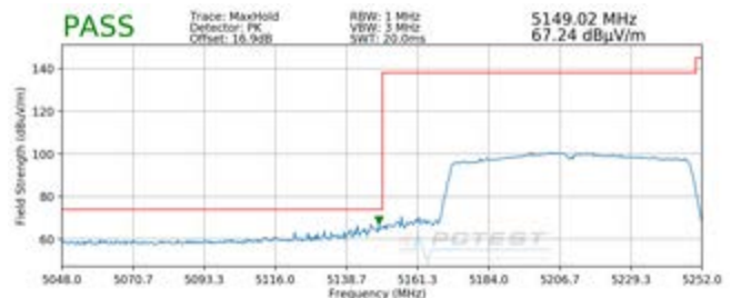
Plot 7-36. Radiated Lower Band Edge Plot (Peak – UNII Band 1)
