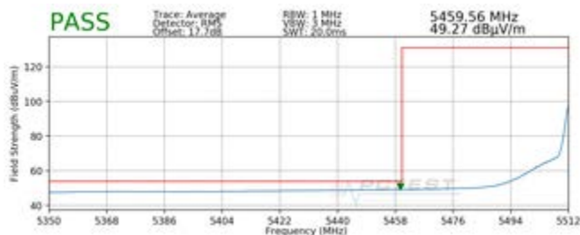
Plot 7-17. Radiated Lower Band Edge Plot (Average – UNII Band 2C)
