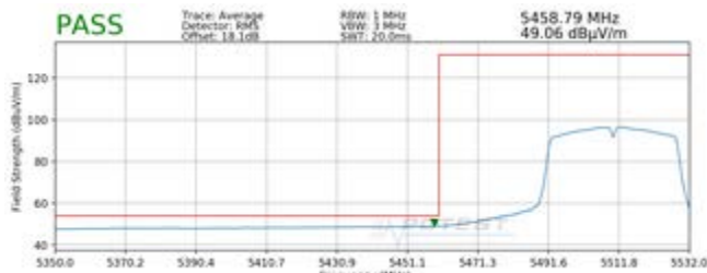
Plot 7-29. Radiated Lower Band Edge Plot (Average – UNII Band 2C)
