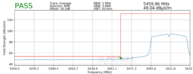
Plot 7-96. Radiated Lower Band Edge Plot (Average - UNII Band 2C)
