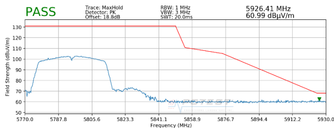
Plot 7-98. Radiated Upper Band Edge Plot (Peak - UNII Band 3)
