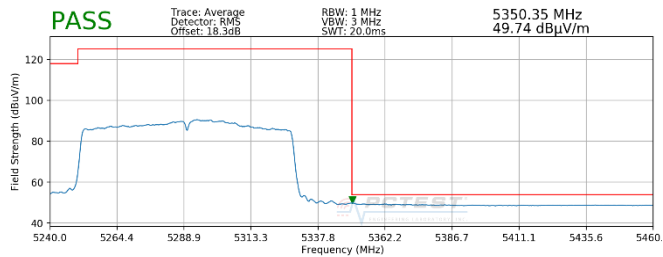
Plot 7-101. Radiated Upper Band Edge Plot (Average – UNII Band 2A)
