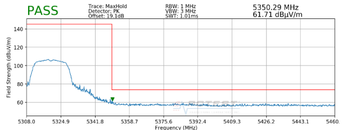
Plot 7-88. Radiated Upper Band Edge Plot (Peak – UNII Band 2A)
