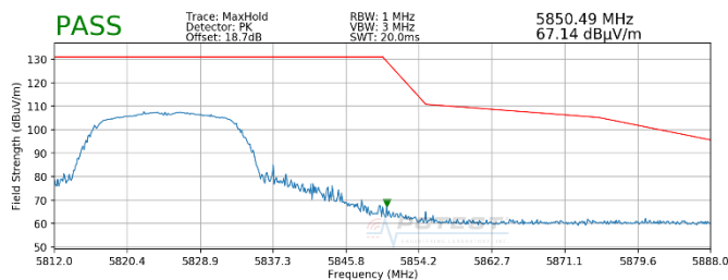
Plot 7-91. Radiated Upper Band Edge Plot (Peak - UNII Band 3)
