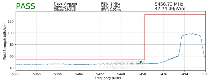
Plot 7-89. Radiated Lower Band Edge Plot (Average - UNII Band 2C)
