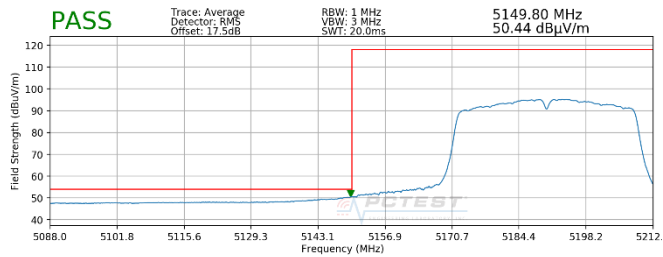
Plot 7-92. Radiated Lower Band Edge Plot (Average – UNII Band 1)
