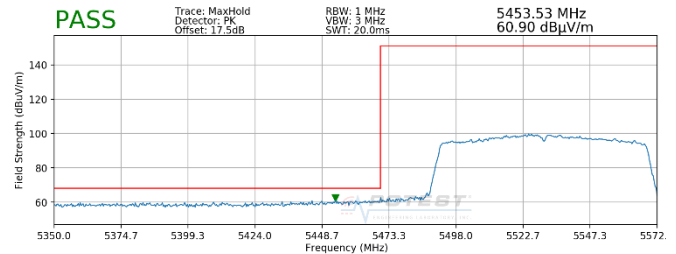
Plot 7-104. Radiated Lower Band Edge Plot (Peak – UNII Band 2C)
