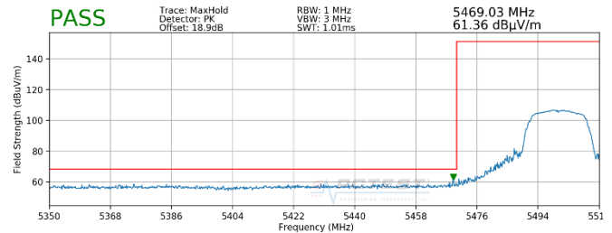
Plot 7-90. Radiated Lower Band Edge Plot (Peak - UNII Band 2C)
