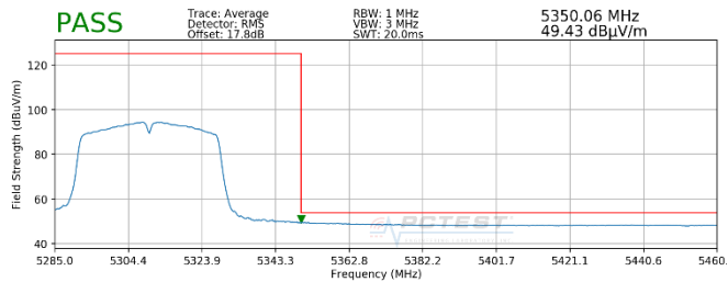
Plot 7-94. Radiated Upper Band Edge Plot (Average – UNII Band 2A)
