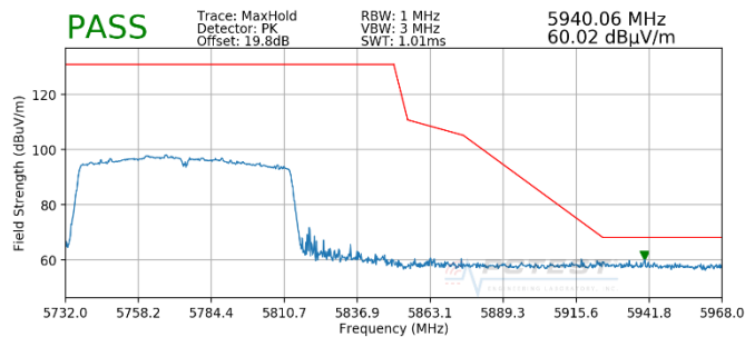
Plot 7-105. Radiated Upper Band Edge Plot (Peak – UNII Band 3)
