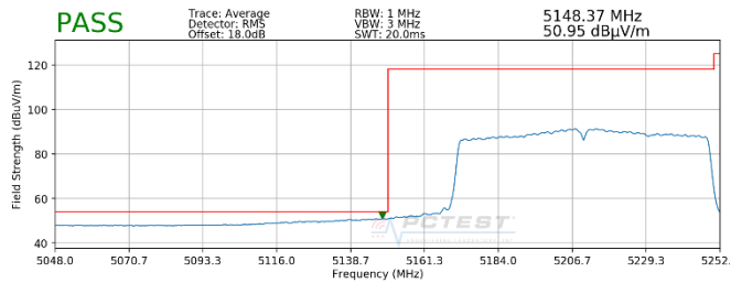
Plot 7-99. Radiated Lower Band Edge Plot (Average – UNII Band 1)
