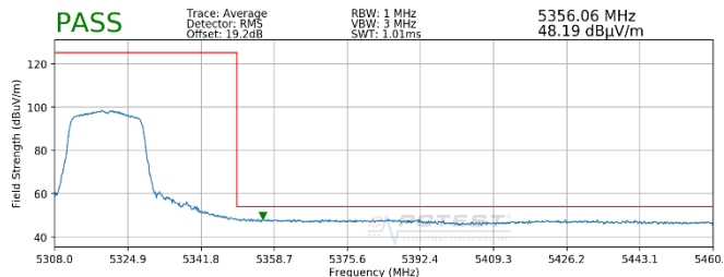
Plot 7-87. Radiated Upper Band Edge Plot (Average – UNII Band 2A)
