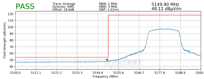
Plot 7-85. Radiated Lower Band Edge Plot (Average – UNII Band 1)
