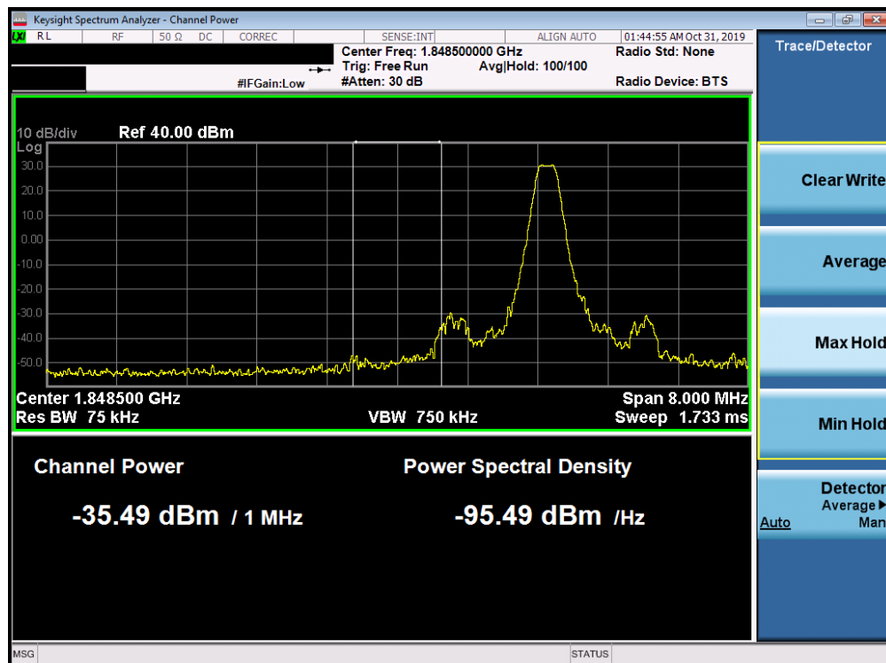
Plot 7-76. Lower Extended Band Edge Plot (PCS GPRS Mode - Low Channel)
