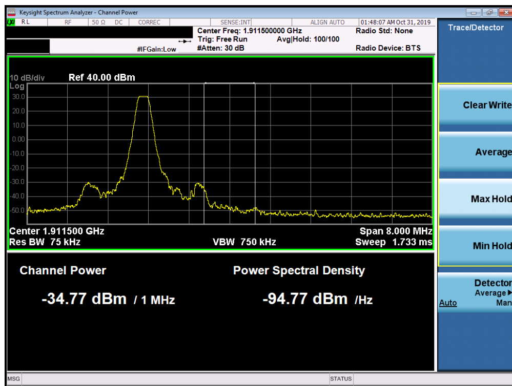
Plot 7-78. Upper Extended Band Edge Plot (PCS GPRS Mode - High Channel)
