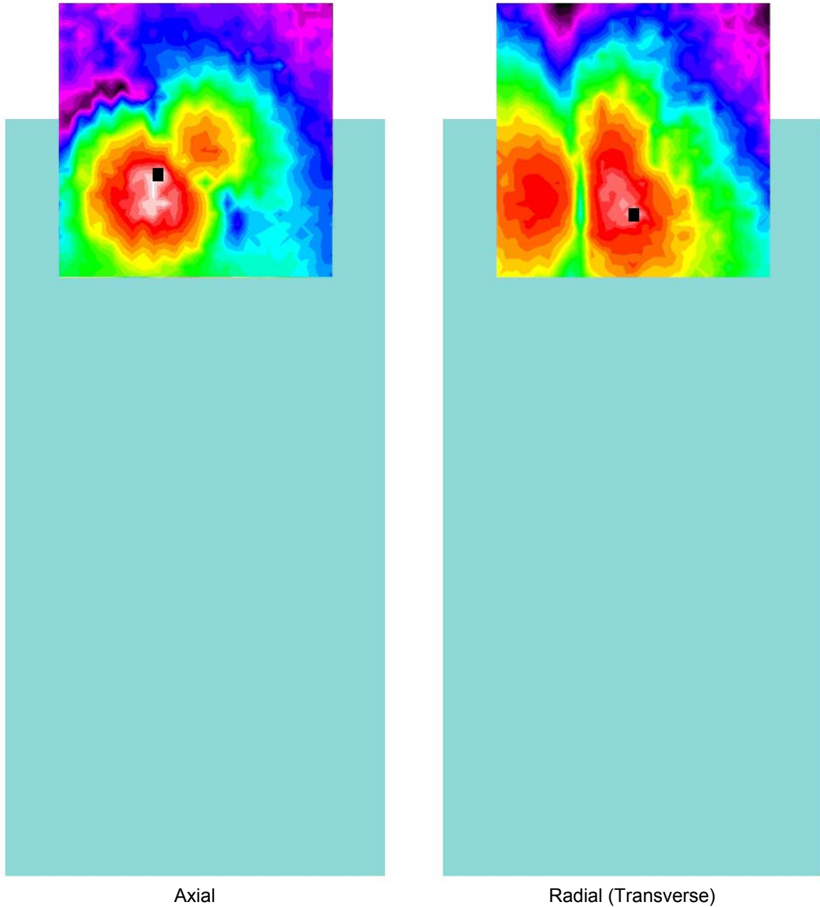
Figure 7-3 T-Coil Scan Overlay Magnetic Field Distributions
