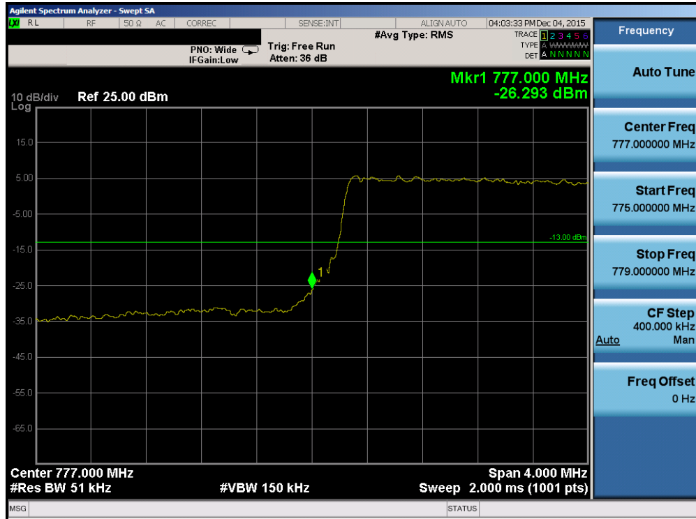
Plot 7-57. Lower Band Edge Plot (Band 13 – 5.0MHz QPSK – RB Size 25)
