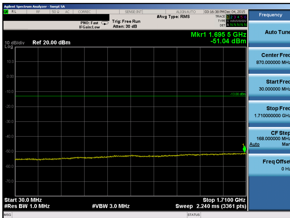
Plot 7-44. Conducted Spurious Plot (Band 4 – 15.0MHz QPSK – RB Size 1, RB Offset 0 – High Channel)
