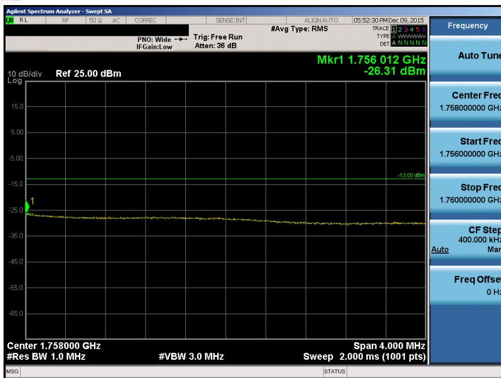
Plot 7-84. Upper Extended Band Edge Plot (Band 4 – 15.0MHz QPSK – RB Size 75)
