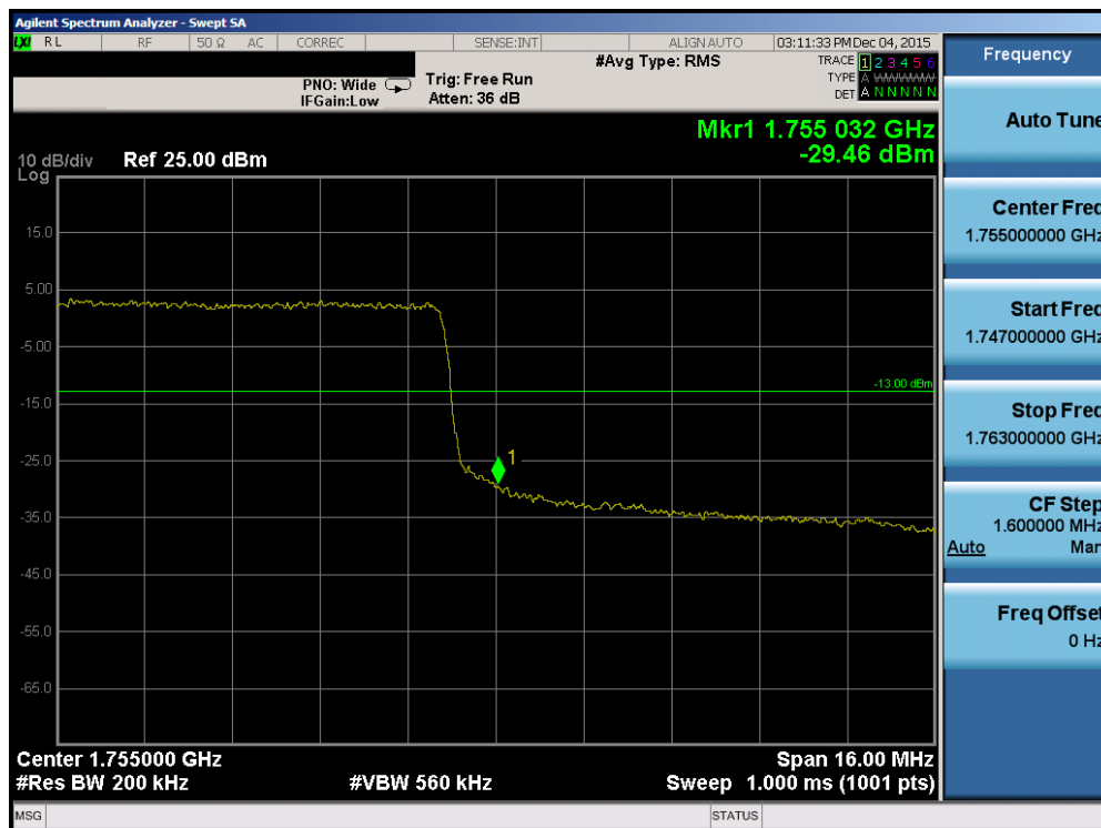
Plot 7-87. Upper Band Edge Plot (Band 4 – 20.0MHz QPSK – RB Size 100)
