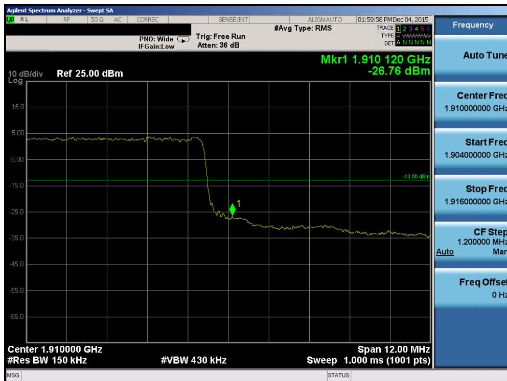
Plot 7-107. Upper Band Edge Plot (Band 2 – 15.0MHz QPSK – RB Size 75)
