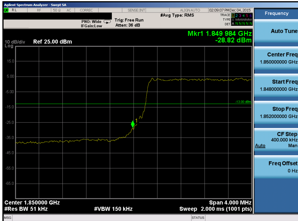
Plot 7-97. Lower Band Edge Plot (Band 2 - 5.0MHz QPSK - RB Size 25)
