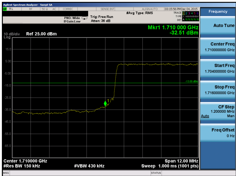
Plot 7-81. Lower Band Edge Plot (Band 4 – 15.0MHz QPSK – RB Size 75)
