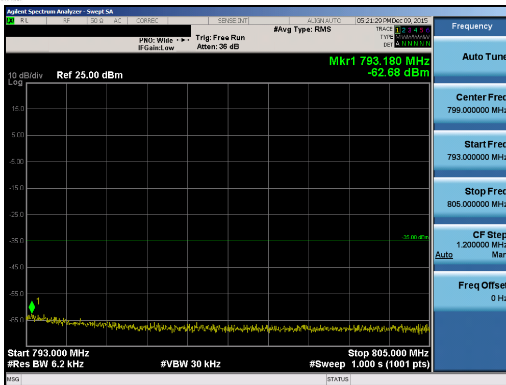
Plot 7-64. Upper Emission Mask Edge Plot (Band 13 – 10.0MHz QPSK – RB Size 50)
