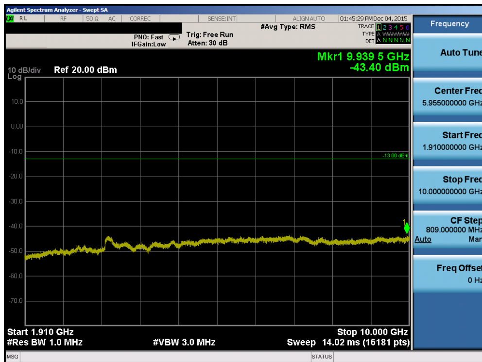
Plot 7-49. Conducted Spurious Plot (Band 2 – 20.0MHz QPSK – RB Size 1, RB Offset 0 – Low Channel)
