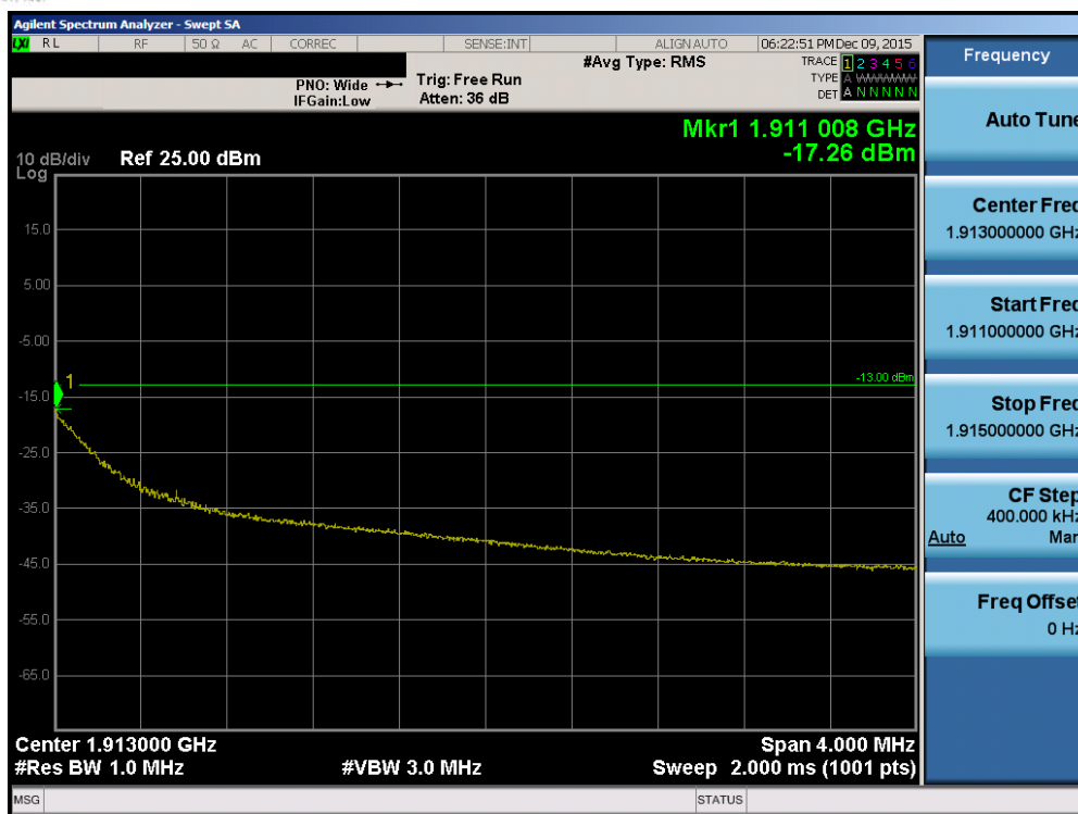
Plot 7-92. Upper Extended Band Edge Plot (Band 2 - 1.4MHz QPSK - RB Size 6)
