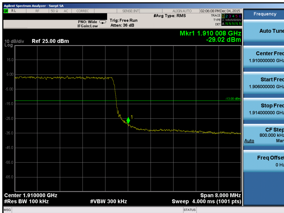
Plot 7-103. Upper Band Edge Plot (Band 2 – 10.0MHz QPSK – RB Size 50)
