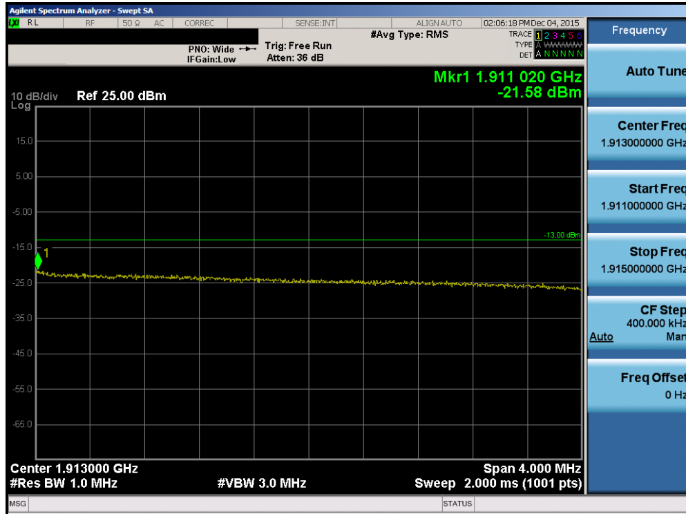
Plot 7-104. Upper Extended Band Edge Plot (Band 2 - 10.0MHz QPSK - RB Size 50)
