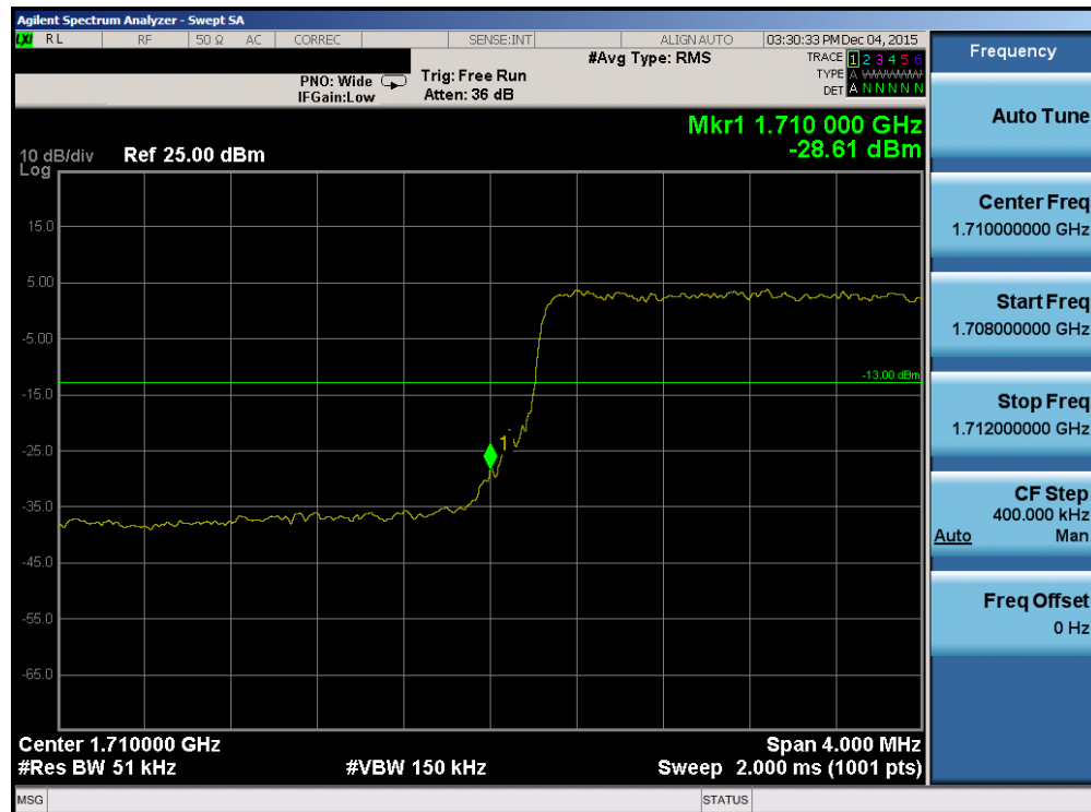
Plot 7-73. Lower Band Edge Plot (Band 4 – 5.0MHz QPSK – RB Size 25)
