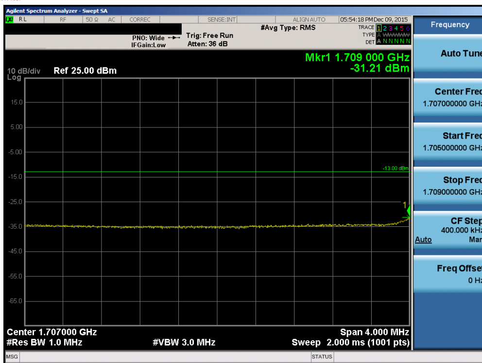
Plot 7-78. Lower Extended Band Edge Plot (Band 4 – 10.0MHz QPSK – RB Size 50)
