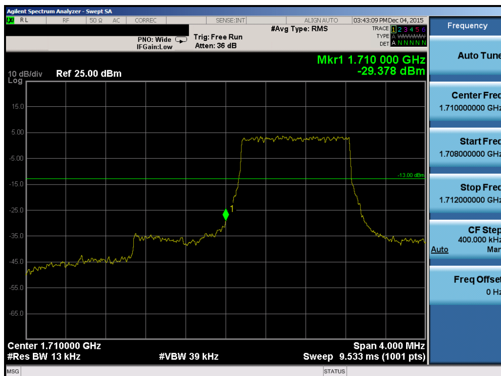
Plot 7-65. Lower Band Edge Plot (Band 4 – 1.4MHz QPSK – RB Size 6)
