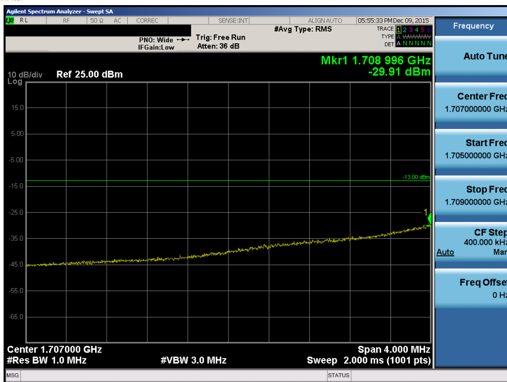
Plot 7-74. Lower Extended Band Edge Plot (Band 4 – 5.0MHz QPSK – RB Size 25)
