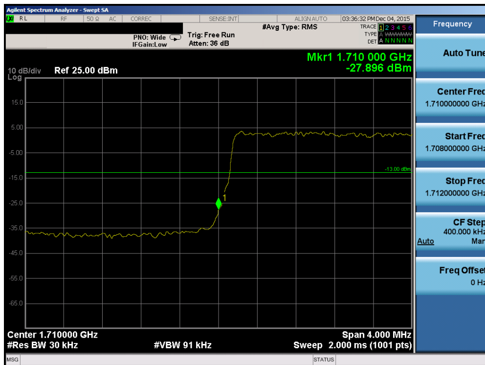
Plot 7-69. Lower Band Edge Plot (Band 4 – 3.0MHz QPSK – RB Size 15)
