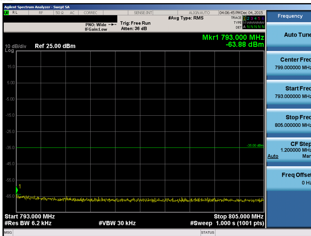
Plot 7-60. Upper Emission Mask Edge Plot (Band 13 – 5.0MHz QPSK – RB Size 25)
