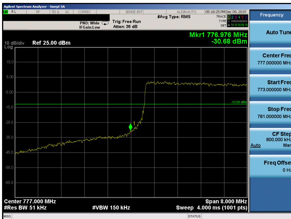
Plot 7-61. Lower Band Edge Plot (Band 13 – 10.0MHz QPSK – RB Size 50)
