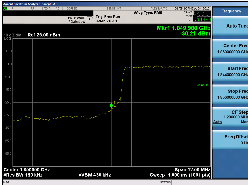
Plot 7-105. Lower Band Edge Plot (Band 2 - 15.0MHz QPSK - RB Size 75)
