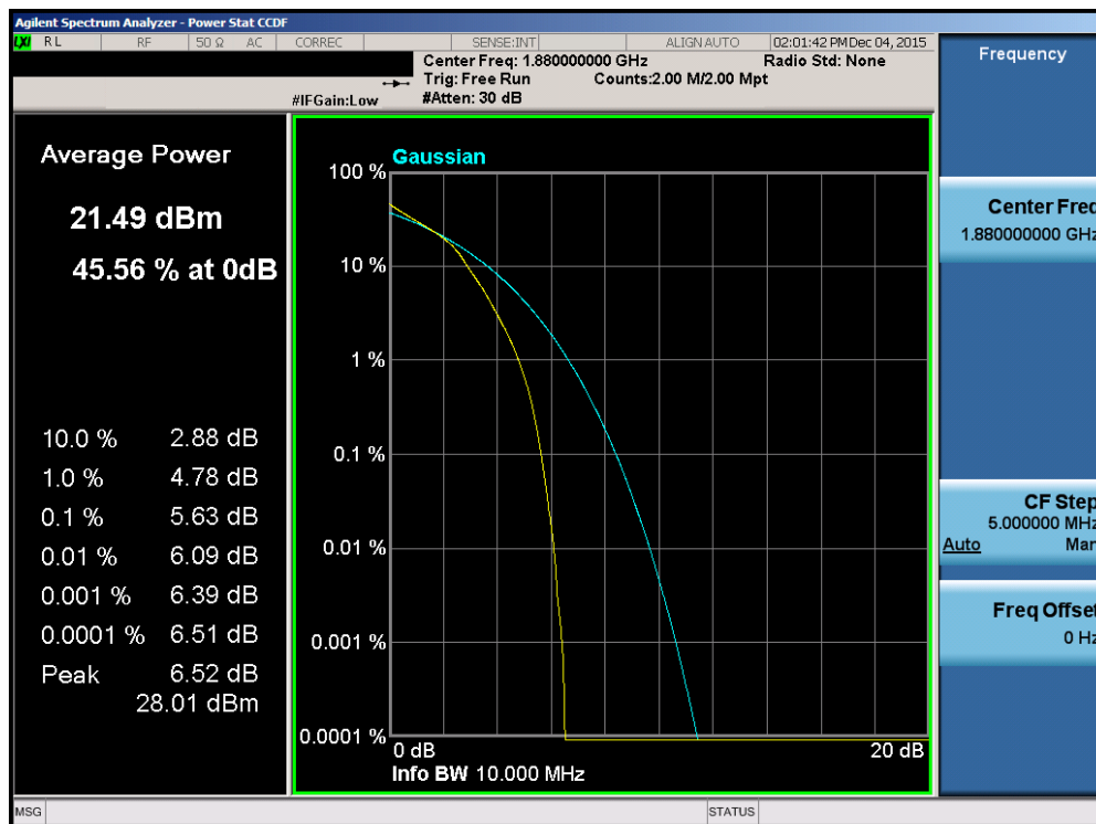
Plot 7-120. PAR Plot (Band 2 – 10.0MHz 16-QAM – RB Size 50)
