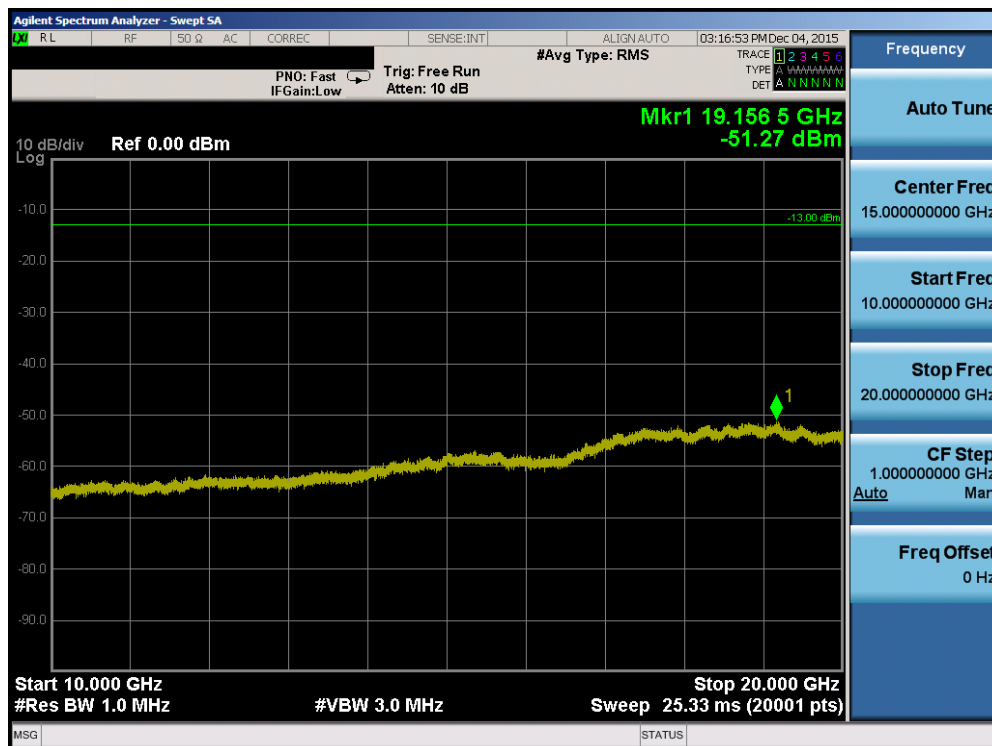
Plot 7-46. Conducted Spurious Plot (Band 4 – 15.0MHz QPSK – RB Size 1, RB Offset 0 – High Channel)
