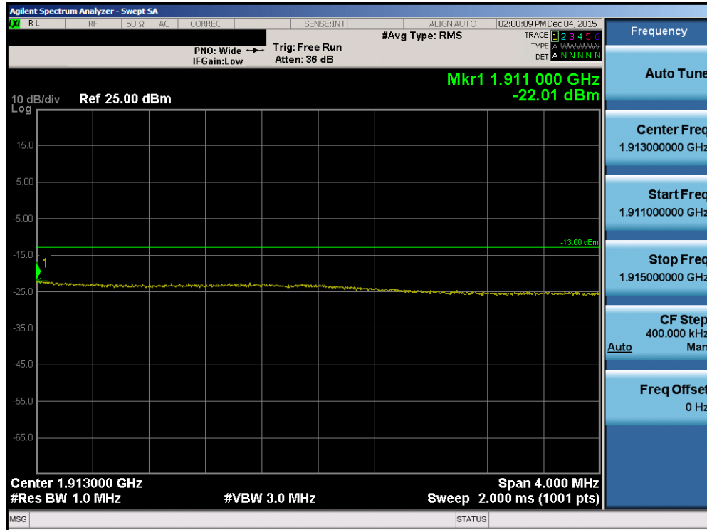
Plot 7-108. Upper Extended Band Edge Plot (Band 2 – 15.0MHz QPSK – RB Size 75)
