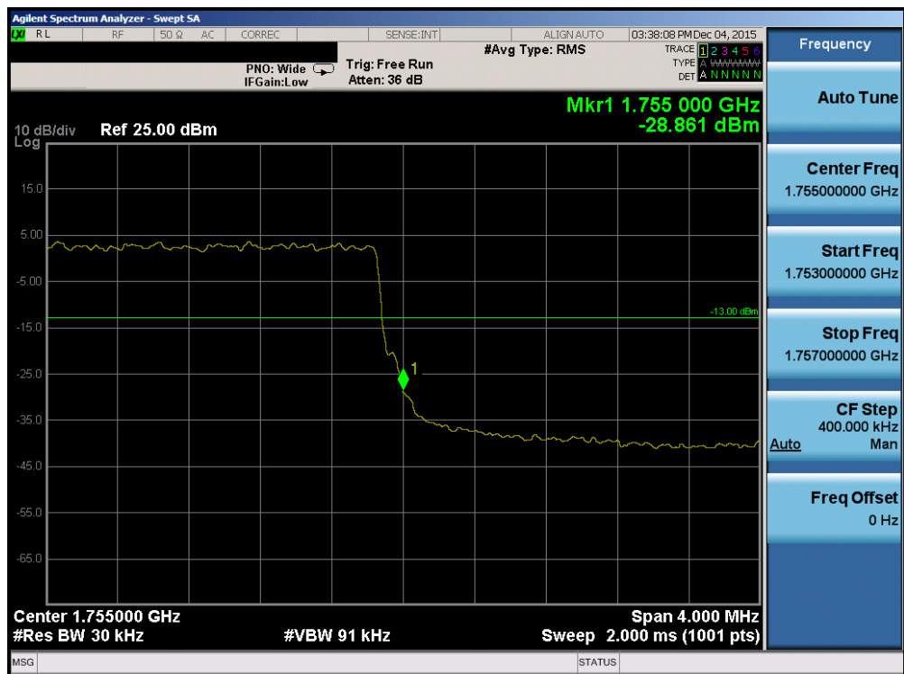
Plot 7-71. Upper Band Edge Plot (Band 4 – 3.0MHz QPSK – RB Size 15)
