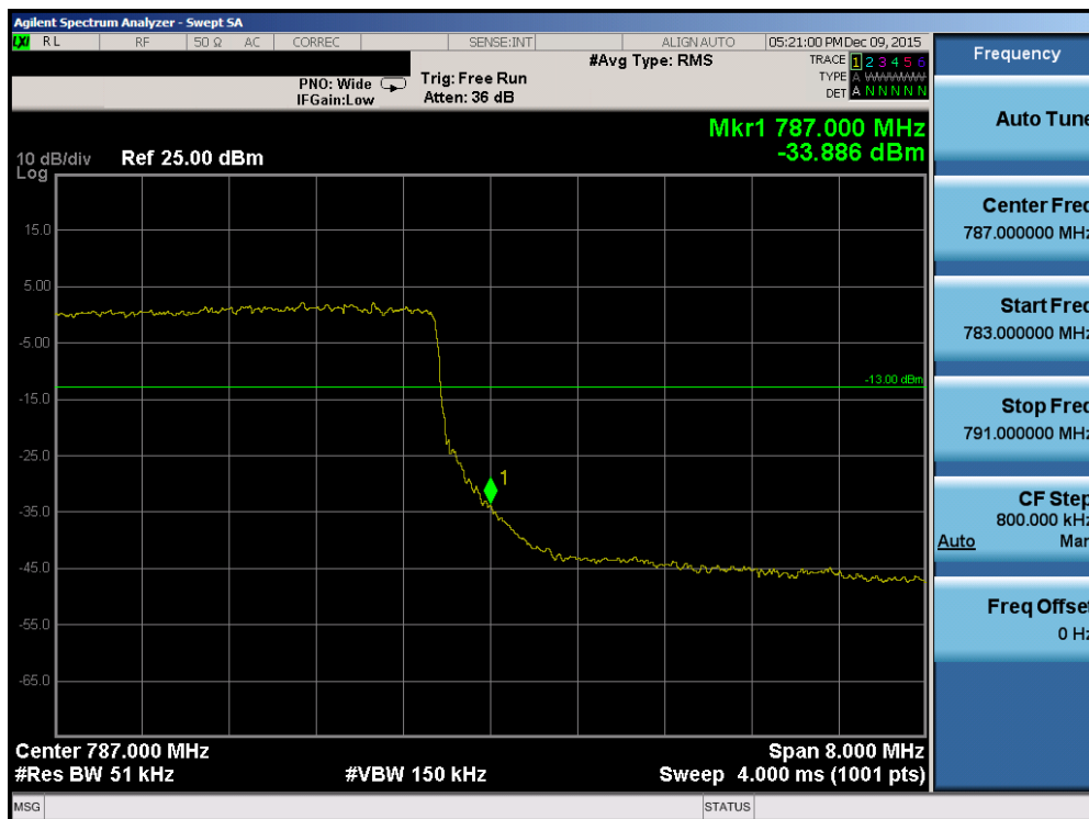
Plot 7-63. Upper Band Edge Plot (Band 13 – 10.0MHz QPSK – RB Size 50)
