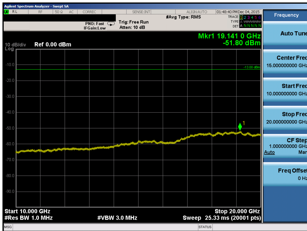
Plot 7-56. Conducted Spurious Plot (Band 2 – 20.0MHz QPSK – RB Size 1, RB Offset 0 – High Channel)
