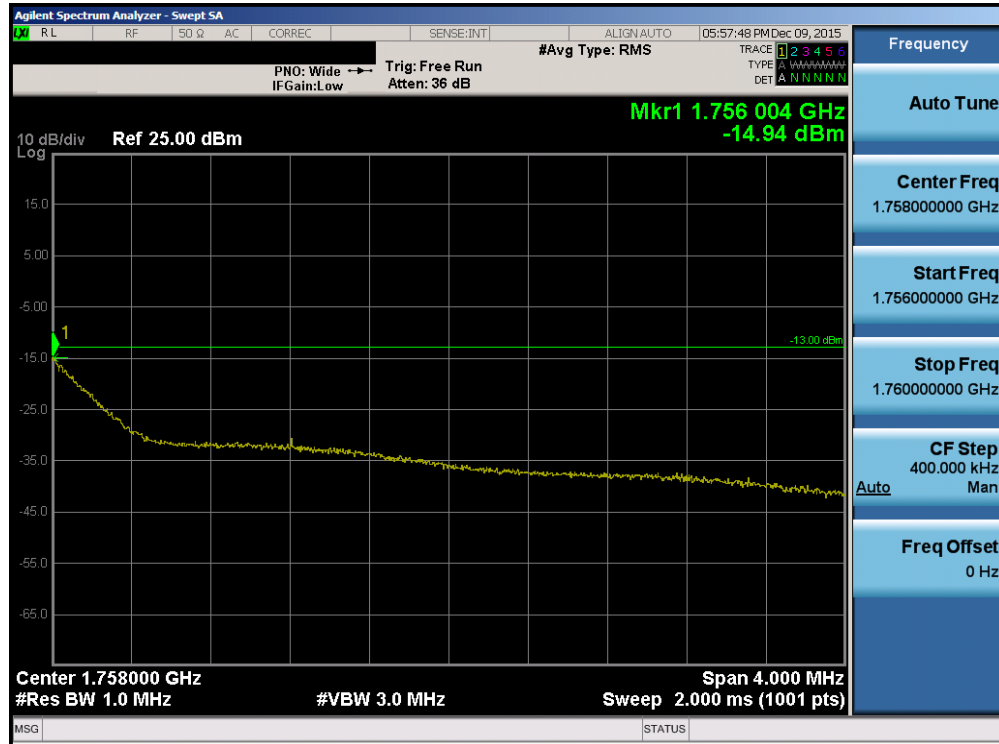
Plot 7-72. Upper Extended Band Edge Plot (Band 4 – 3.0MHz QPSK – RB Size 15)
