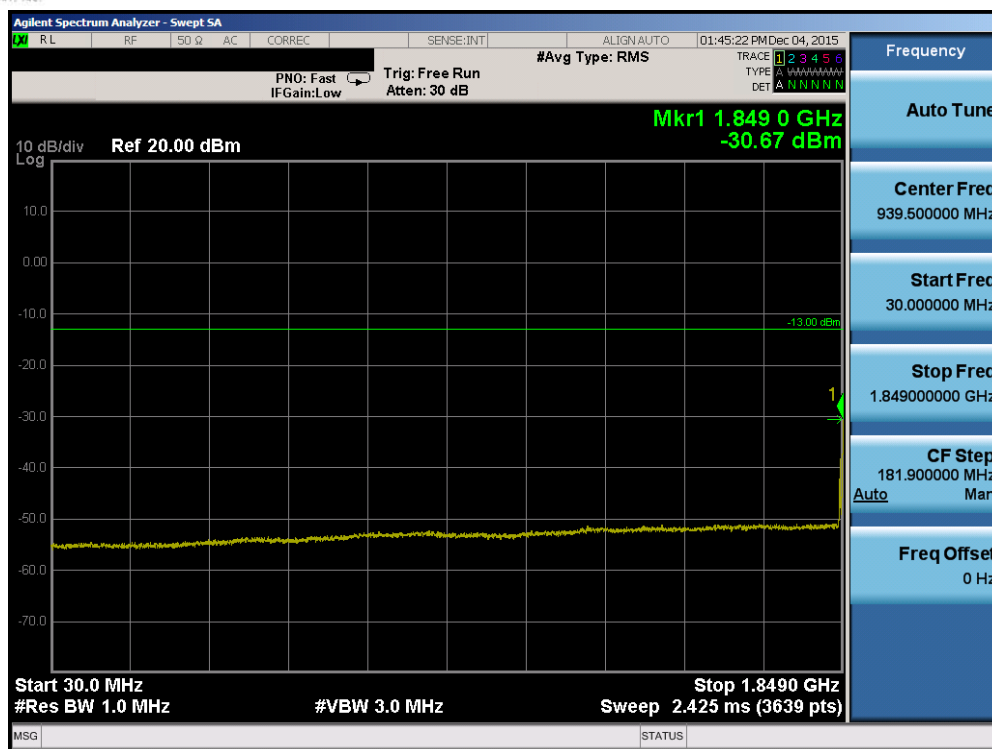
Plot 7-48. Conducted Spurious Plot (Band 2 – 20.0MHz QPSK – RB Size 1, RB Offset 0– Low Channel)
