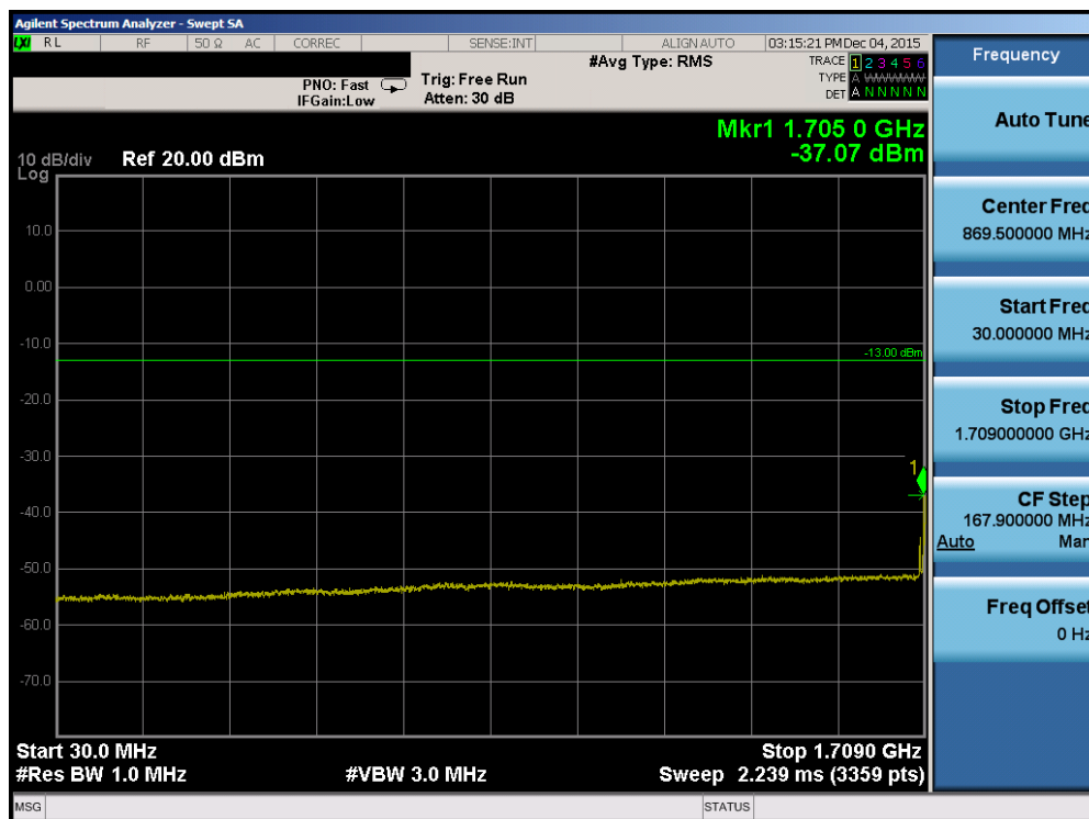
Plot 7-38. Conducted Spurious Plot (Band 4 – 15.0MHz QPSK – RB Size 1, RB Offset 0 – Low Channel)
