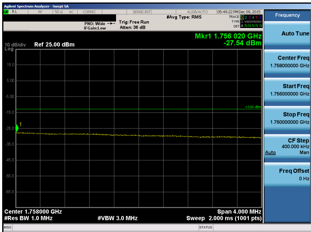
Plot 7-88. Upper Extended Band Edge Plot (Band 4 – 20.0MHz QPSK – RB Size 100)
