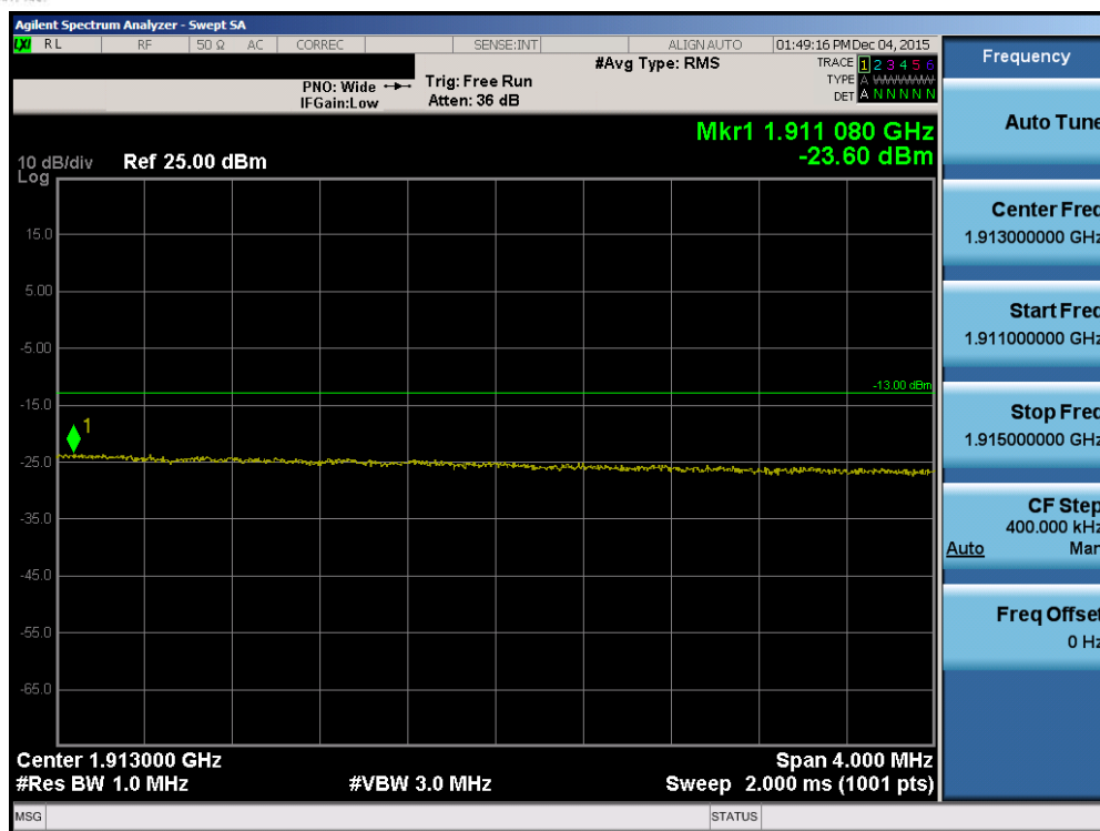
Plot 7-112. Upper Extended Band Edge Plot (Band 2 – 20.0MHz QPSK – RB Size 100)
