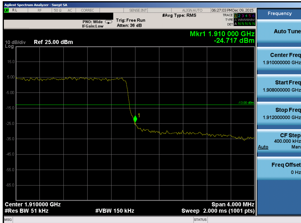
Plot 7-95. Upper Band Edge Plot (Band 2 – 3.0MHz QPSK – RB Size 15)
