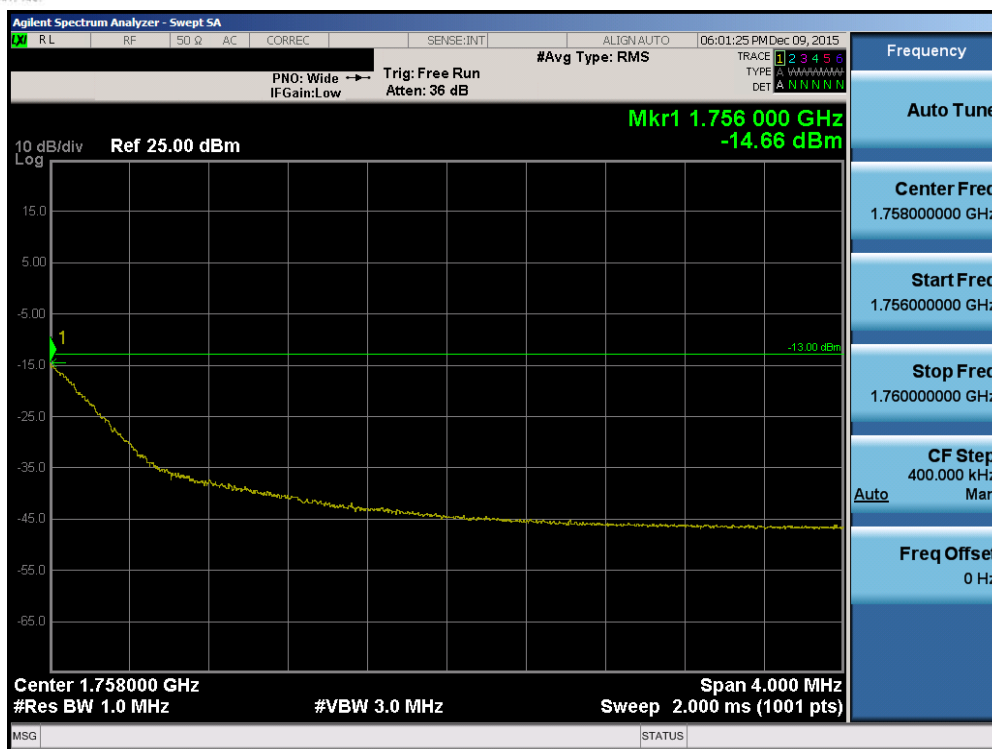
Plot 7-68. Upper Extended Band Edge Plot (Band 4 – 1.4MHz QPSK – RB Size 6)
