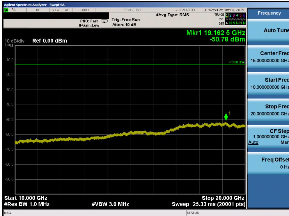
Plot 7-53. Conducted Spurious Plot (Band 2 – 20.0MHz QPSK – RB Size 1, RB Offset 0 – Mid Channel)
