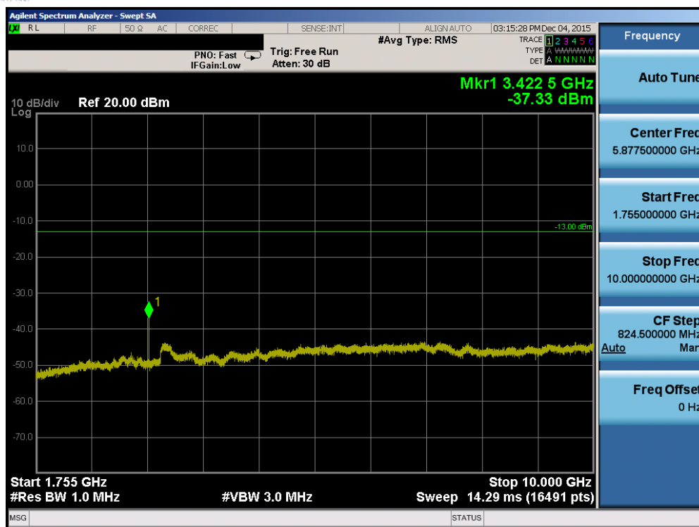
Plot 7-39. Conducted Spurious Plot (Band 4 – 15.0MHz QPSK – RB Size 1, RB Offset 0 – Low Channel)
