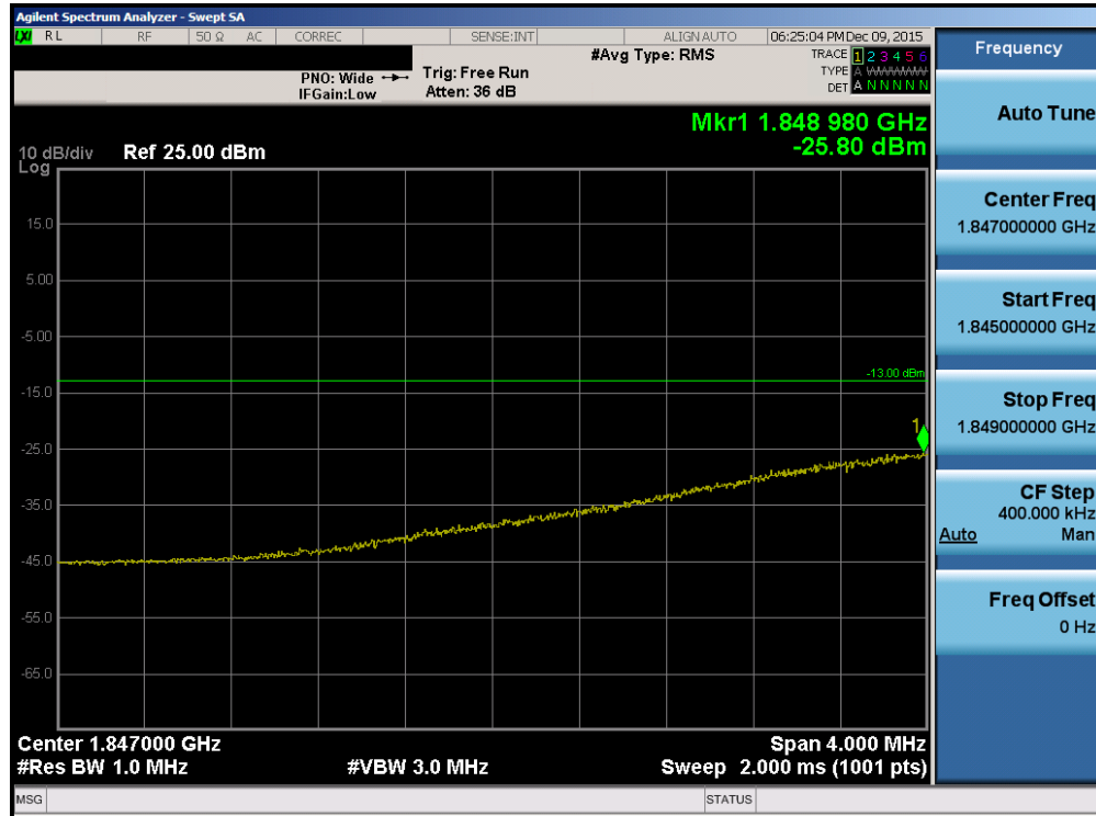
Plot 7-94. Lower Extended Band Edge Plot (Band 2 – 3.0MHz QPSK – RB Size 15)
