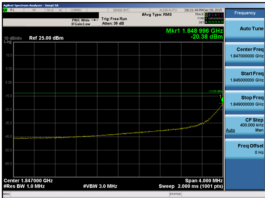
Plot 7-90. Lower Extended Band Edge Plot (Band 2 – 1.4MHz QPSK – RB Size 6)
