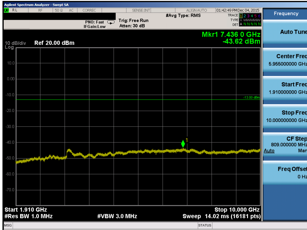
Plot 7-52. Conducted Spurious Plot (Band 2 – 20.0MHz QPSK – RB Size 1, RB Offset 0 – Mid Channel)
