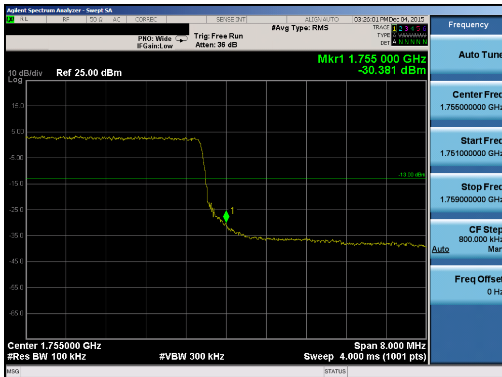
Plot 7-79. Upper Band Edge Plot (Band 4 – 10.0MHz QPSK – RB Size 50)
