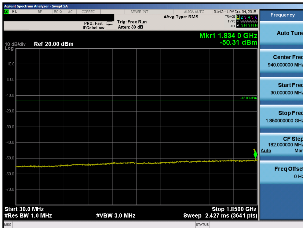
Plot 7-51. Conducted Spurious Plot (Band 2 – 20.0MHz QPSK – RB Size 1, RB Offset 0 – Mid Channel)
