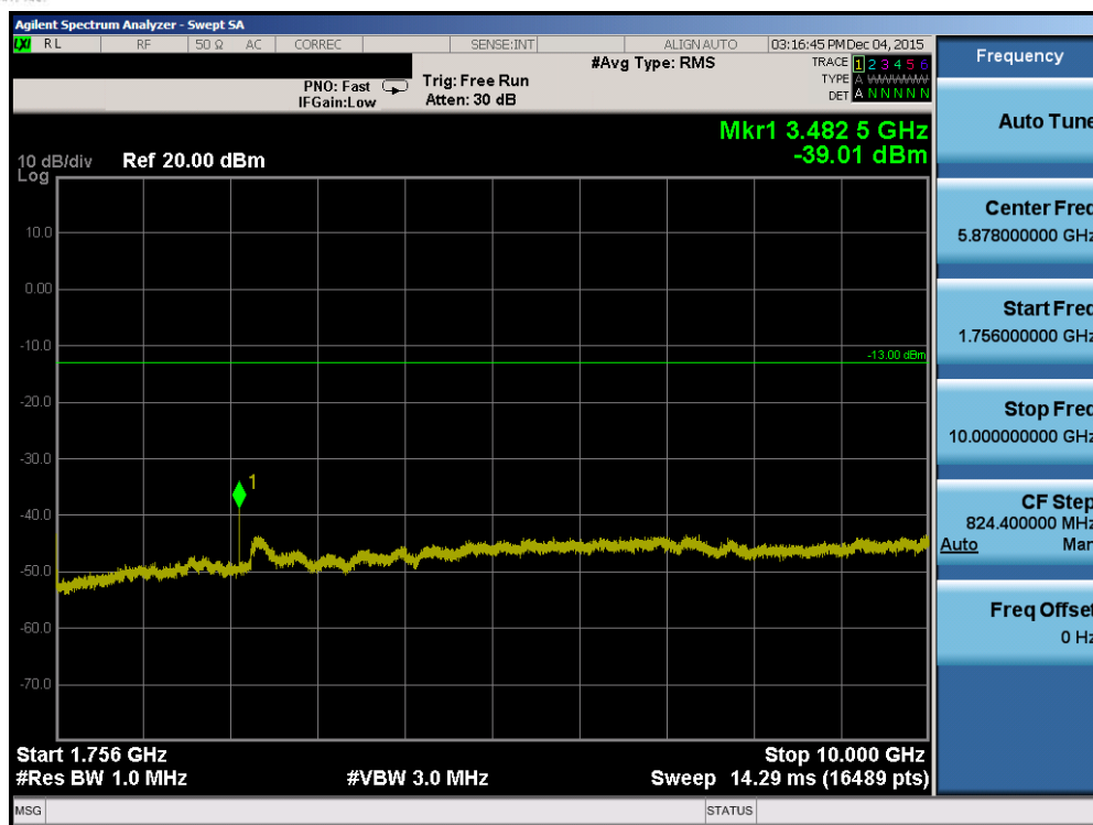
Plot 7-45. Conducted Spurious Plot (Band 4 – 15.0MHz QPSK – RB Size 1, RB Offset 0 – High Channel)
