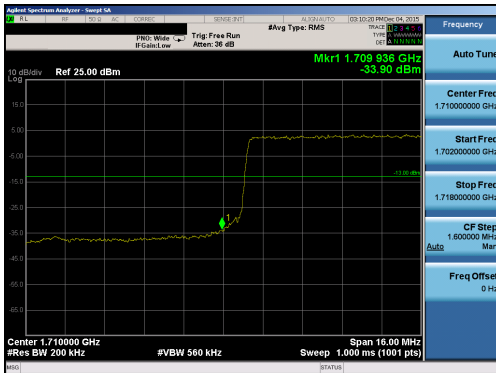
Plot 7-85. Lower Band Edge Plot (Band 4 – 20.0MHz QPSK – RB Size 100)
