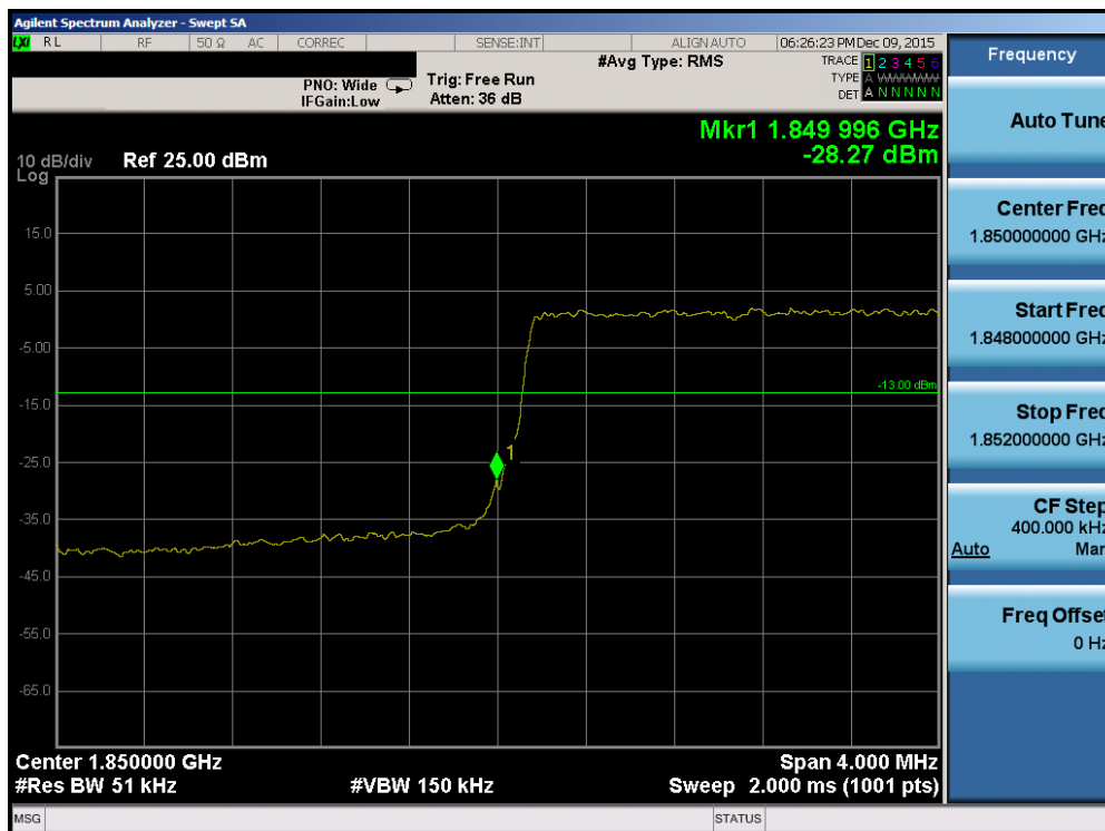
Plot 7-93. Lower Band Edge Plot (Band 2 - 3.0MHz QPSK - RB Size 15)
