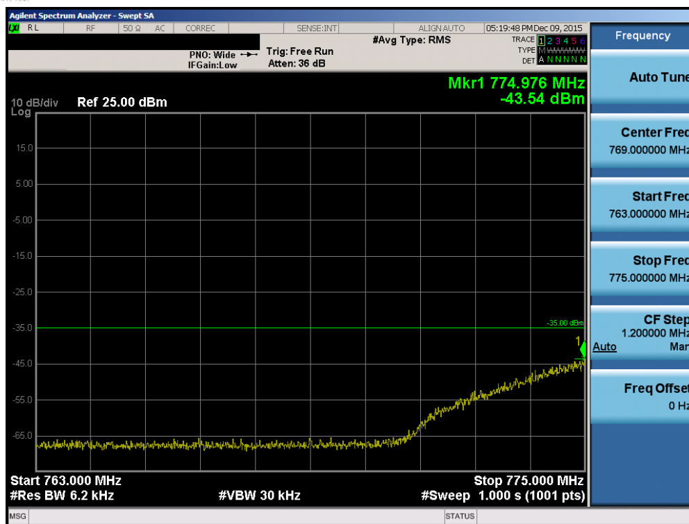
Plot 7-62. Lower Emission Mask Edge Plot (Band 13 – 10.0MHz QPSK – RB Size 50)
