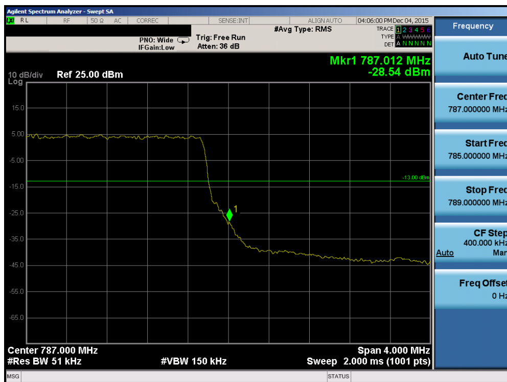
Plot 7-59. Upper Band Edge Plot (Band 13 – 5.0MHz QPSK – RB Size 25)
