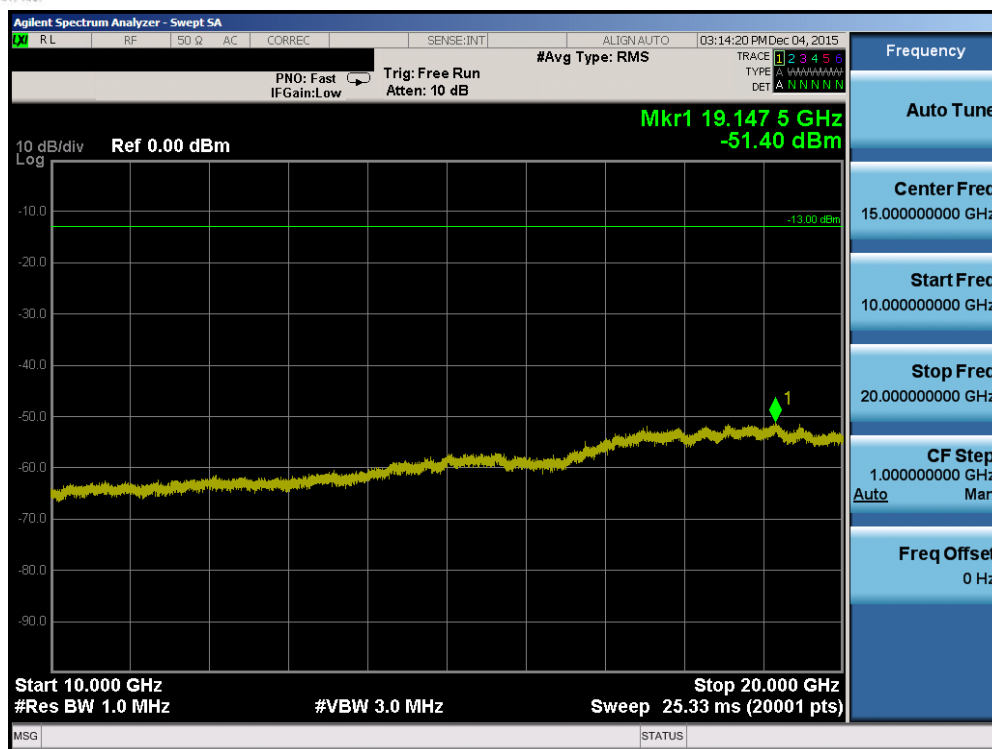
Plot 7-43. Conducted Spurious Plot (Band 4 – 15.0MHz QPSK – RB Size 1, RB Offset 0 – Mid Channel)
