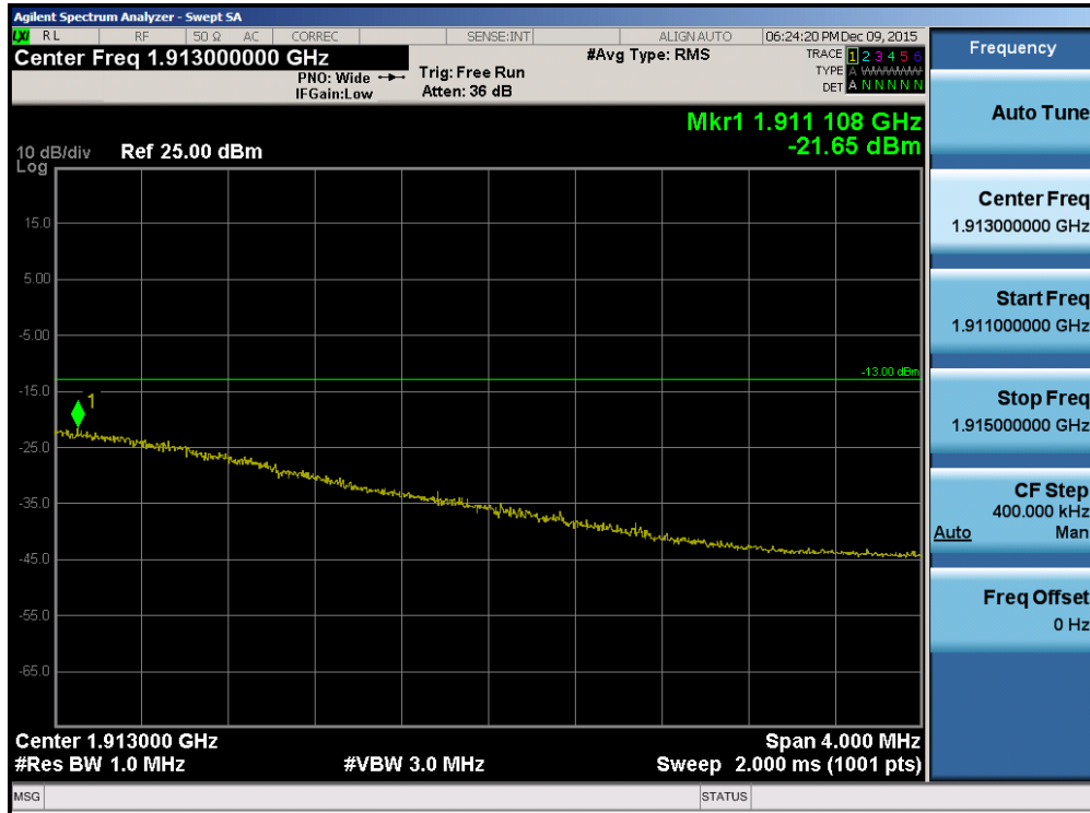
Plot 7-96. Upper Extended Band Edge Plot (Band 2 - 3.0MHz QPSK - RB Size 15)
