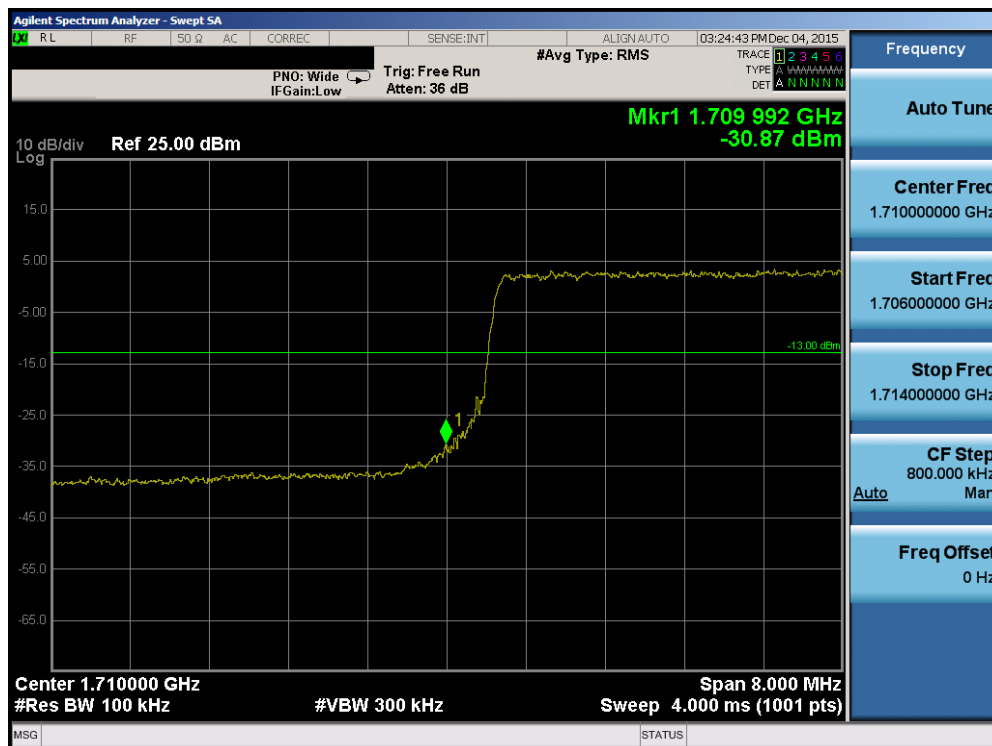
Plot 7-77. Lower Band Edge Plot (Band 4 – 10.0MHz QPSK – RB Size 50)
