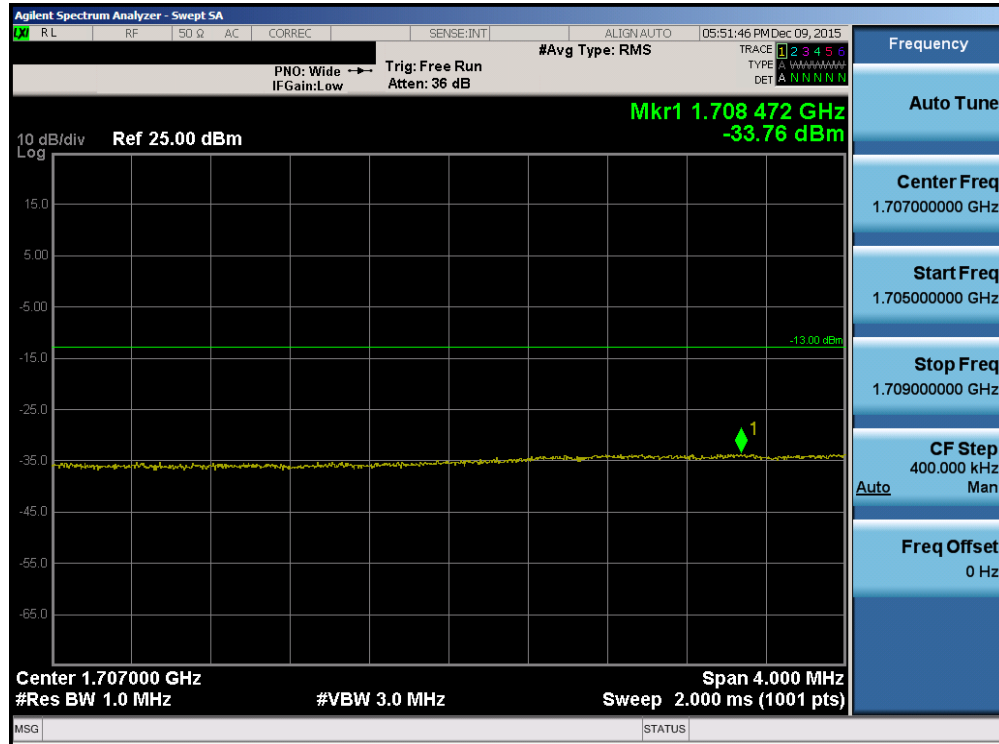
Plot 7-82. Lower Extended Band Edge Plot (Band 4 – 15.0MHz QPSK – RB Size 75)
