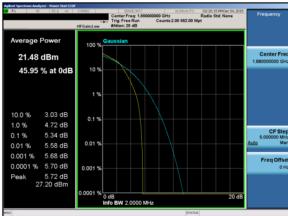
Plot 7-114. PAR Plot (Band 2 – 1.4MHz 16-QAM – RB Size 6)
