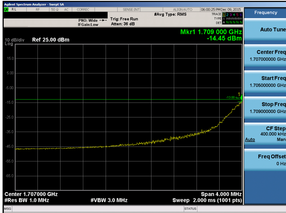
Plot 7-66. Lower Extended Band Edge Plot (Band 4 – 1.4MHz QPSK – RB Size 6)
