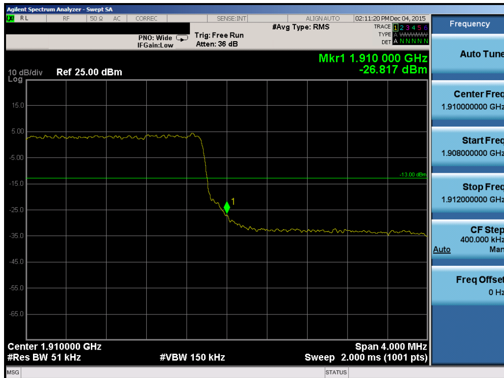
Plot 7-99. Upper Band Edge Plot (Band 2 – 5.0MHz QPSK – RB Size 25)
