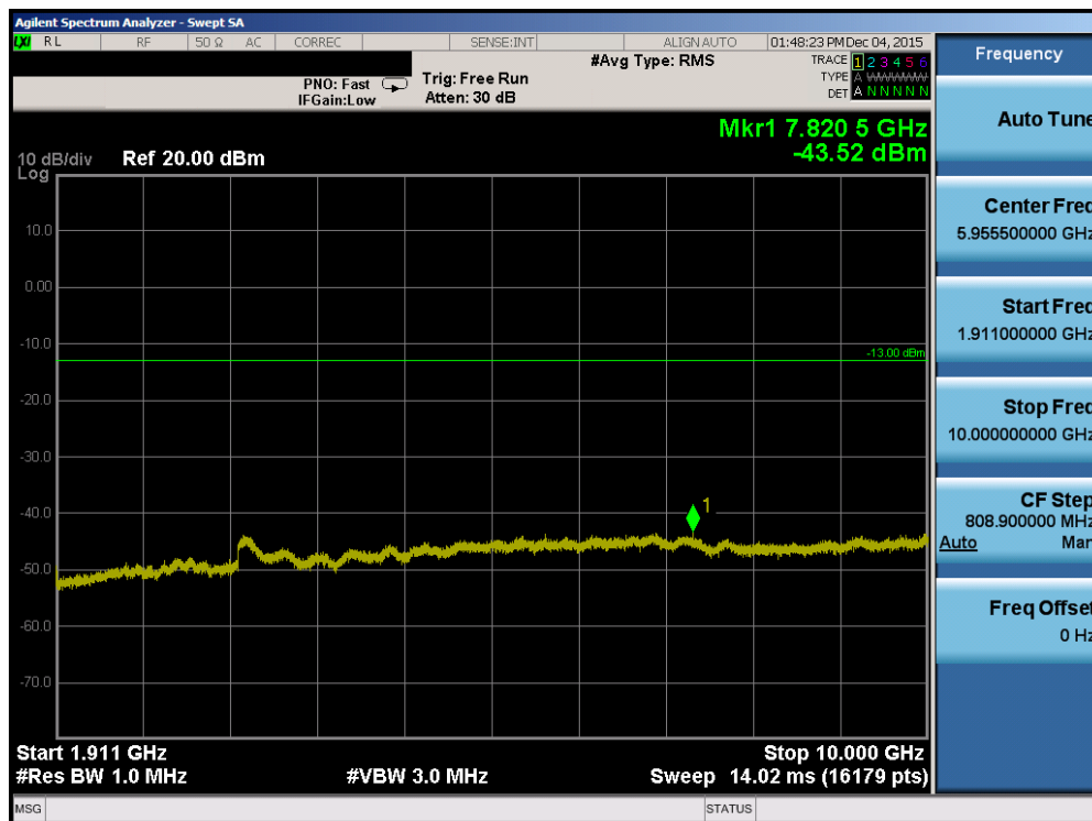
Plot 7-55. Conducted Spurious Plot (Band 2 – 20.0MHz QPSK – RB Size 1, RB Offset 0 – High Channel)
