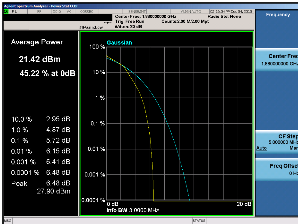
Plot 7-116. PAR Plot (Band 2 – 3.0MHz 16-QAM – RB Size 15)
