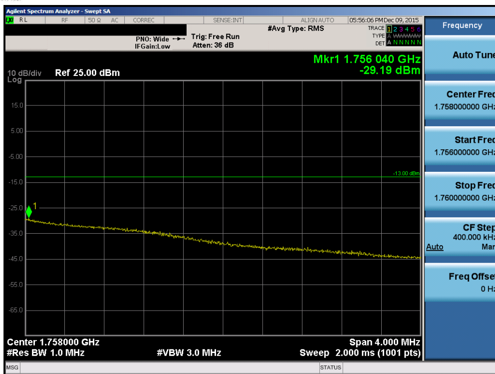
Plot 7-76. Upper Extended Band Edge Plot (Band 4 – 5.0MHz QPSK – RB Size 25)
