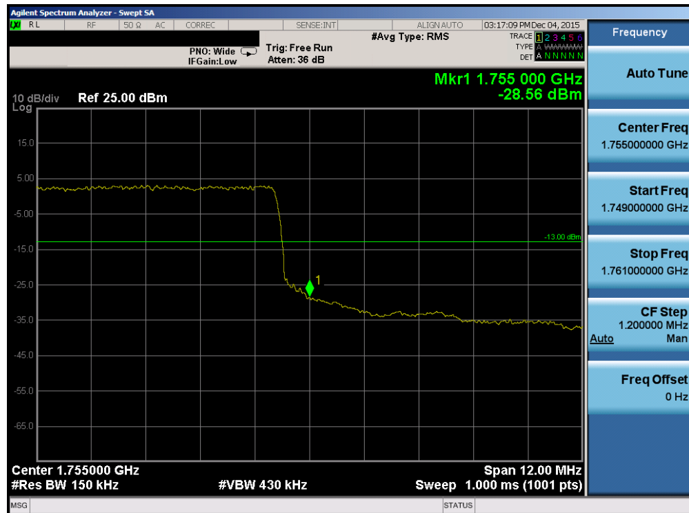
Plot 7-83. Upper Band Edge Plot (Band 4 – 15.0MHz QPSK – RB Size 75)
