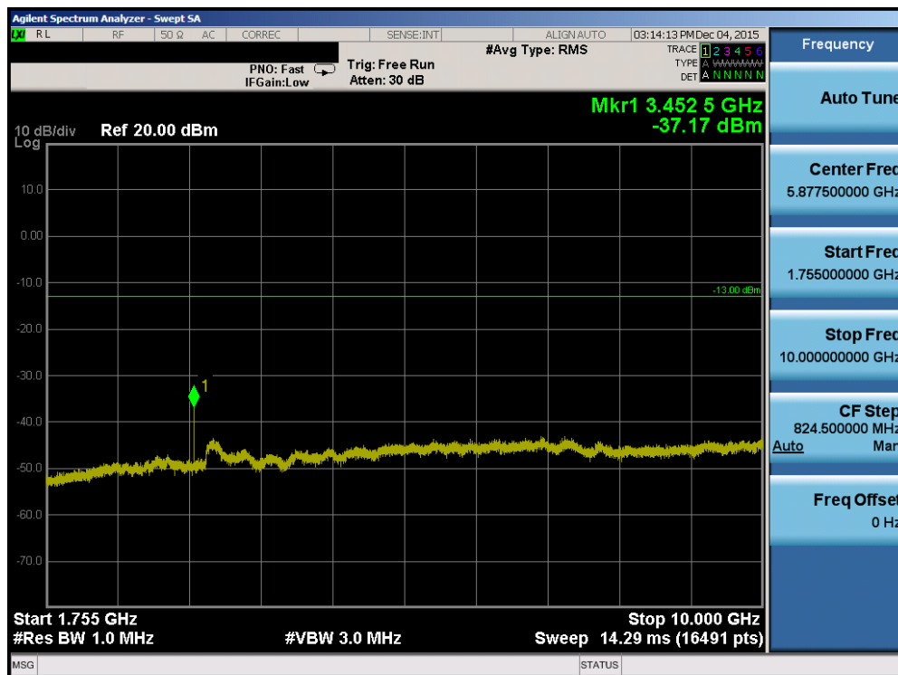
Plot 7-42. Conducted Spurious Plot (Band 4 – 15.0MHz QPSK – RB Size 1, RB Offset 0 – Mid Channel)
