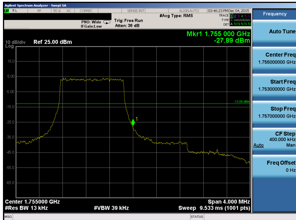
Plot 7-67. Upper Band Edge Plot (Band 4 – 1.4MHz QPSK – RB Size 6)
