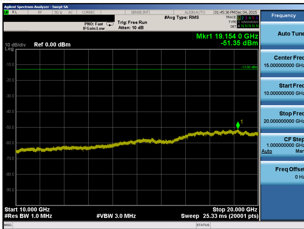
Plot 7-50. Conducted Spurious Plot (Band 2 – 20.0MHz QPSK – RB Size 1, RB Offset 0 – Low Channel)
