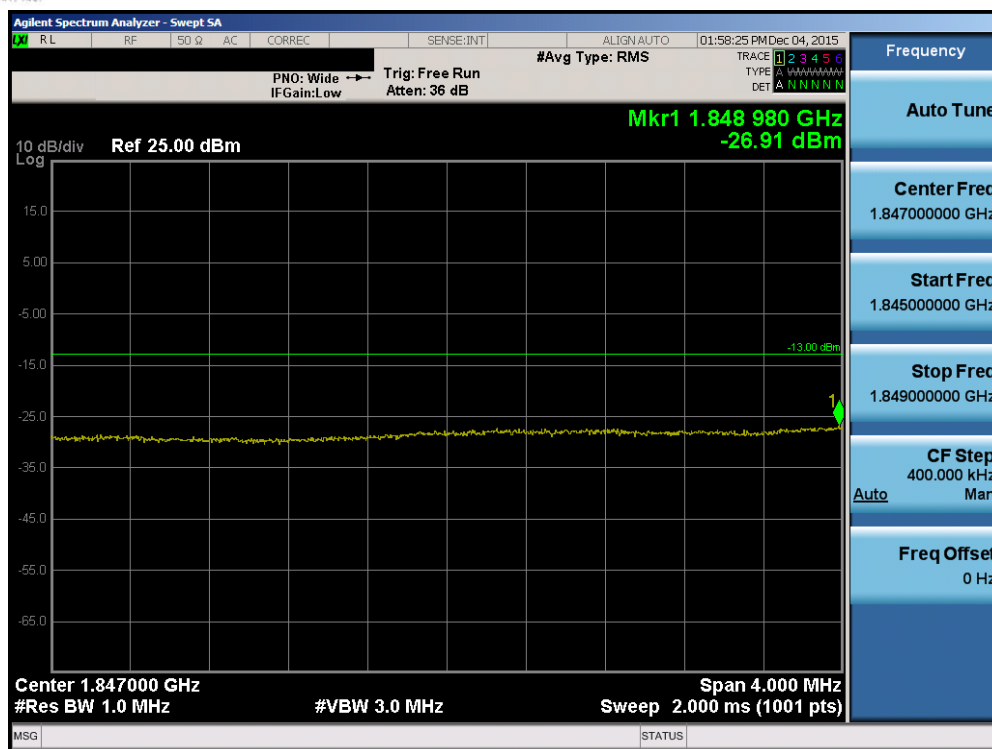
Plot 7-106. Lower Extended Band Edge Plot (Band 2 – 15.0MHz QPSK – RB Size 75)
