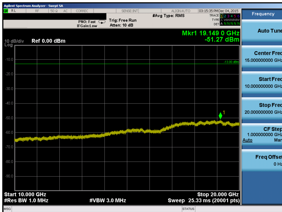
Plot 7-40. Conducted Spurious Plot (Band 4 – 15.0MHz QPSK – RB Size 1, RB Offset 0 – Low Channel)
