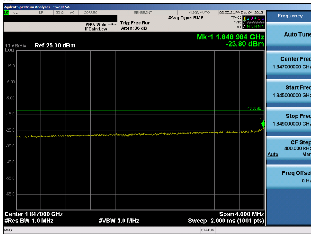
Plot 7-102. Lower Extended Band Edge Plot (Band 2 – 10.0MHz QPSK – RB Size 50)
