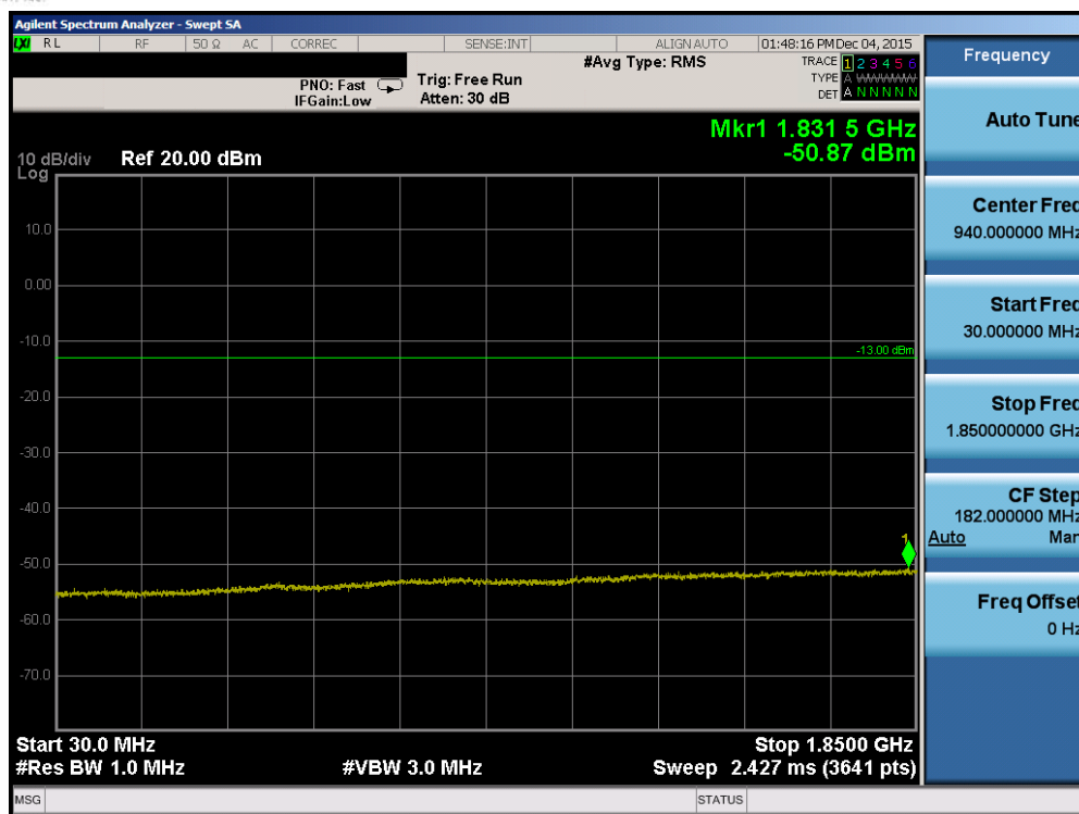
Plot 7-54. Conducted Spurious Plot (Band 2 – 20.0MHz QPSK – RB Size 1, RB Offset 0 – High Channel)
