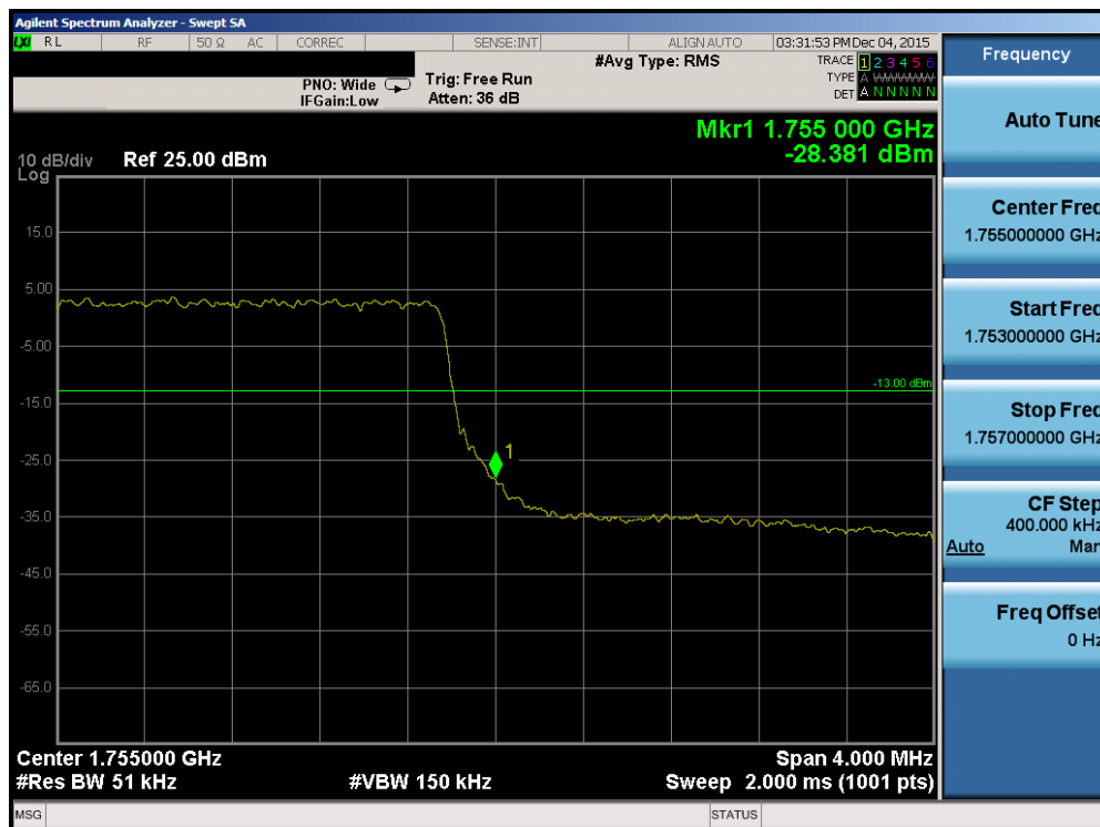
Plot 7-75. Upper Band Edge Plot (Band 4 – 5.0MHz QPSK – RB Size 25)
