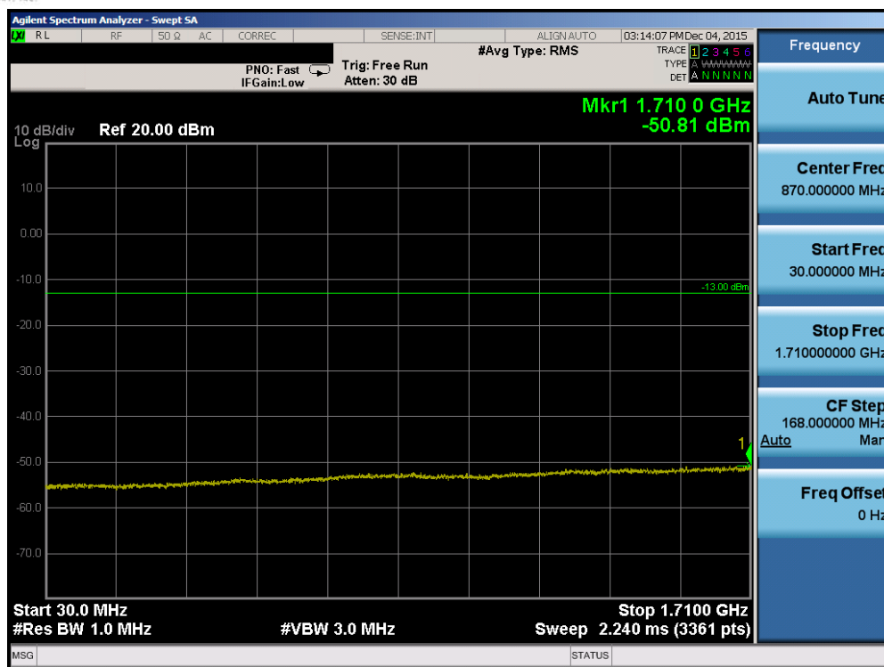
Plot 7-41. Conducted Spurious Plot (Band 4 – 15.0MHz QPSK – RB Size 1, RB Offset 0 – Mid Channel)
