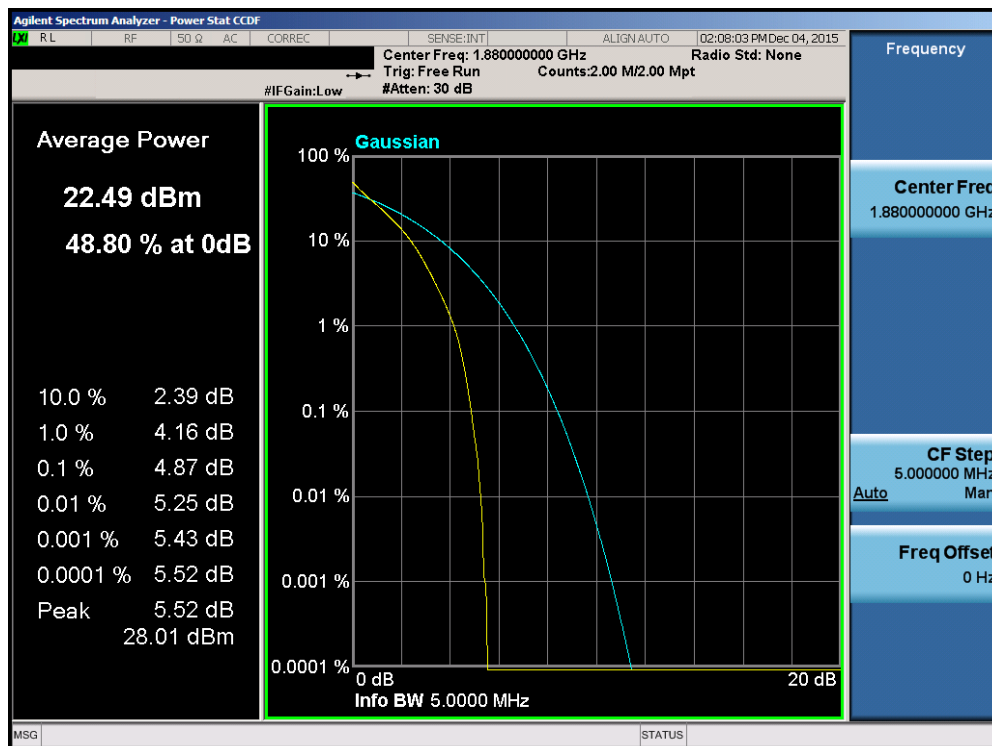
Plot 7-118. PAR Plot (Band 2 – 5.0MHz 16-QAM – RB Size 25)
