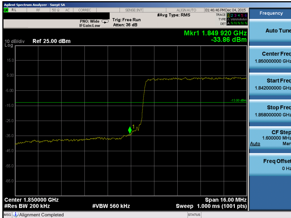
Plot 7-109. Lower Band Edge Plot (Band 2 – 20.0MHz QPSK – RB Size 100)
