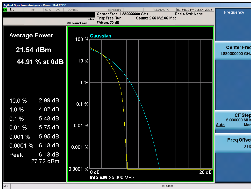
Plot 7-122. PAR Plot (Band 2 – 15.0MHz 16-QAM – RB Size 75)
