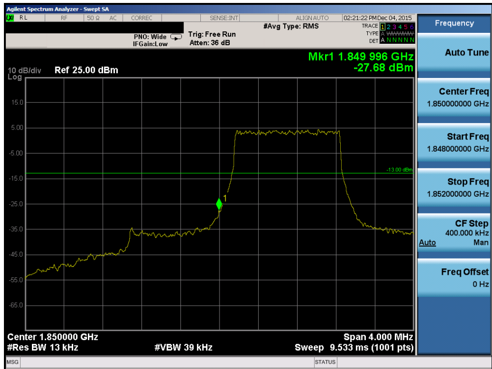
Plot 7-89. Lower Band Edge Plot (Band 2 – 1.4MHz QPSK – RB Size 6)
