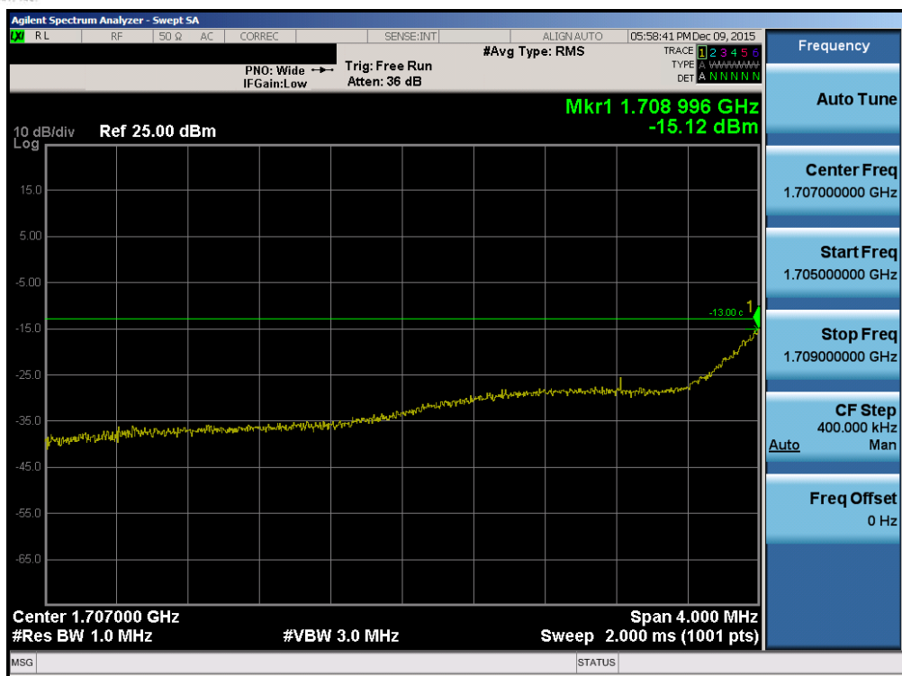
Plot 7-70. Lower Extended Band Edge Plot (Band 4 – 3.0MHz QPSK – RB Size 15)
