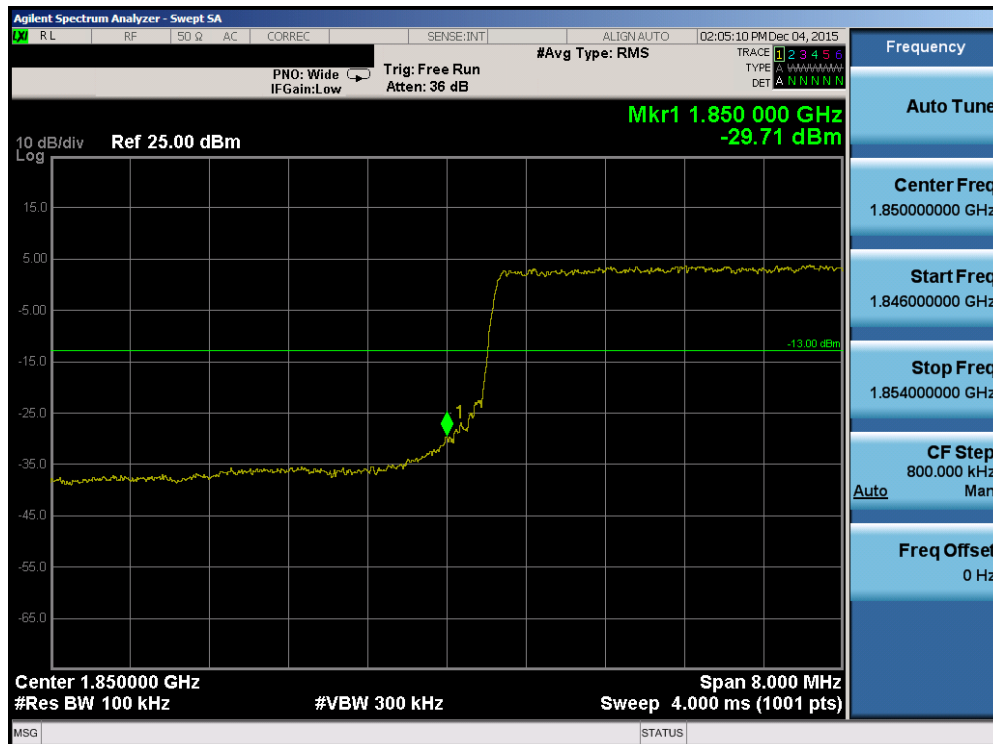
Plot 7-101. Lower Band Edge Plot (Band 2 – 10.0MHz QPSK – RB Size 50)
