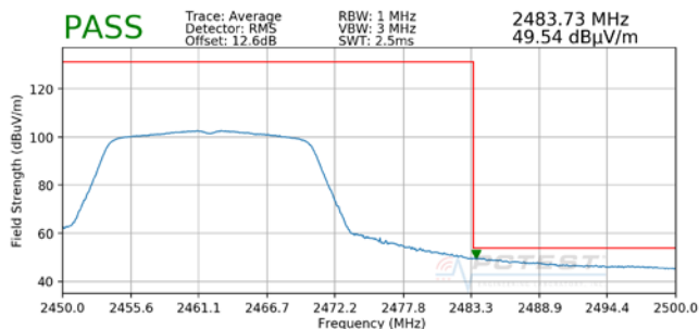
Plot 7-11. Radiated Restricted Upper Band Edge Measurement (Average)
