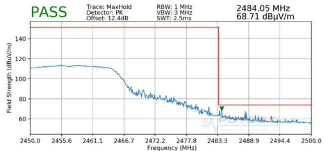
Plot 7-10. Radiated Restricted Upper Band Edge Measurement (Peak)
