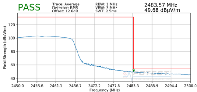
Plot 7-9. Radiated Restricted Upper Band Edge Measurement (Average)
