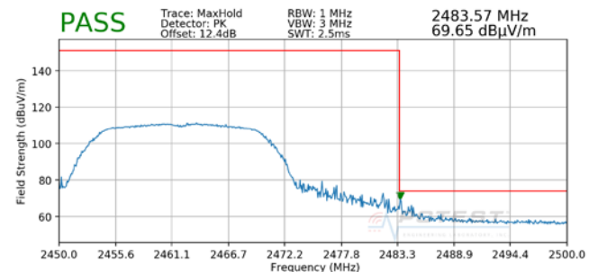
Plot 7-12. Radiated Restricted Upper Band Edge Measurement (Peak)
