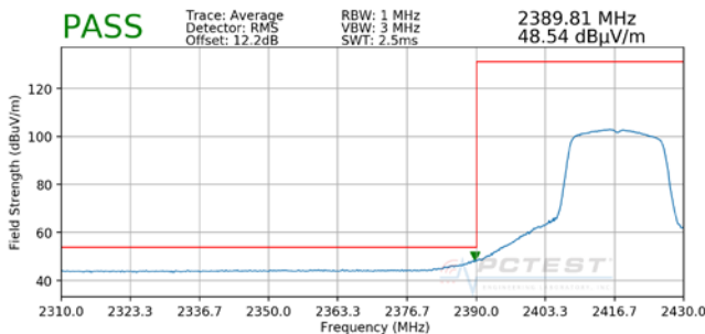
Plot 7-7. Radiated Restricted Lower Band Edge Measurement (Average)
