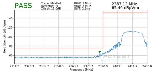
Plot 7-8. Radiated Restricted Lower Band Edge Measurement (Peak)
