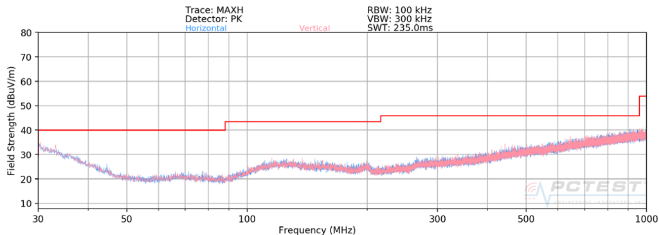
Plot 7-13. Radiated Spurious Plot below 1GHz
