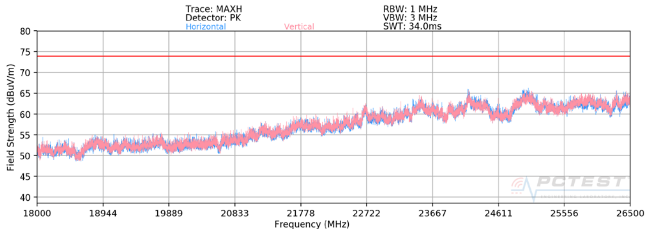
Plot 7-4. Radiated Spurious Plot above 18GHz
