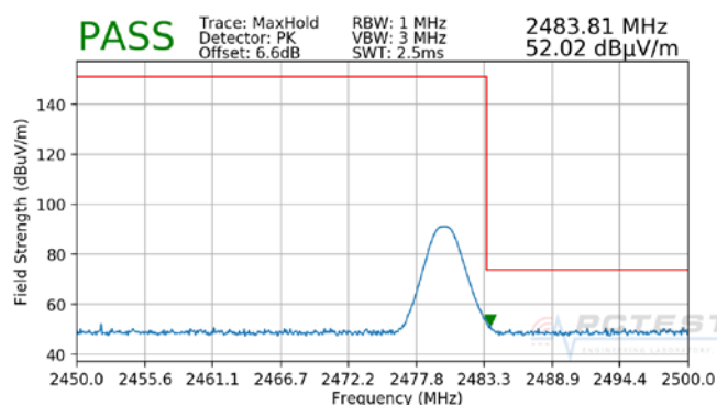
Plot 7-2. Radiated Restricted Upper Band Edge Measurement (Peak)
