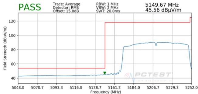
Plot 7-21. Radiated Lower Band Edge Plot (Average – UNII Band 1)
