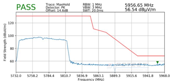
Plot 7-27. Radiated Upper Band Edge Plot (Peak – UNII Band 3)
