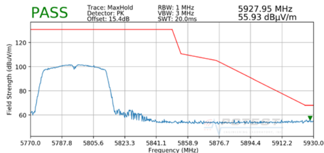
Plot 7-20. Radiated Upper Band Edge Plot (Peak – UNII Band 3)
