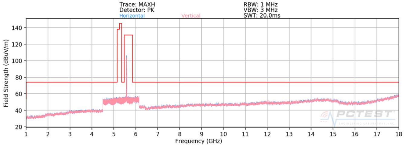
Plot 7-3. Radiated Spurious Plot above 1GHz (802.11a – U2C Ch. 116)
