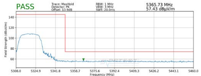
Plot 7-10. Radiated Upper Band Edge Plot (Peak – UNII Band 2A)
