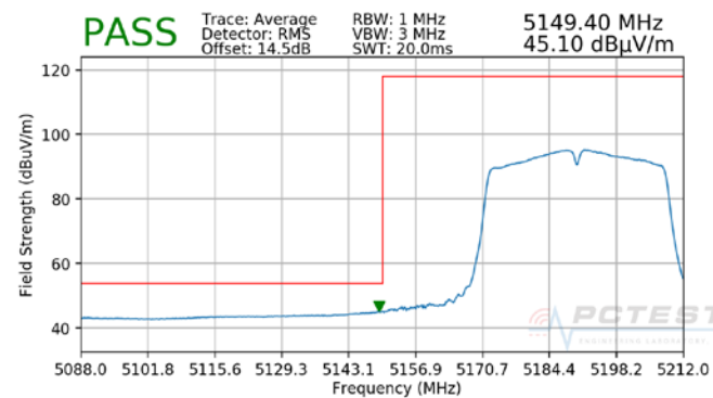
Plot 7-14. Radiated Lower Band Edge Plot (Average – UNII Band 1)
