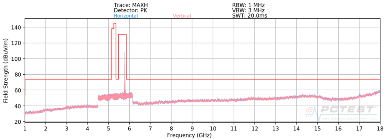
Plot 7-4. Radiated Spurious Plot above 1GHz (802.11a – U3 Ch. 157)
