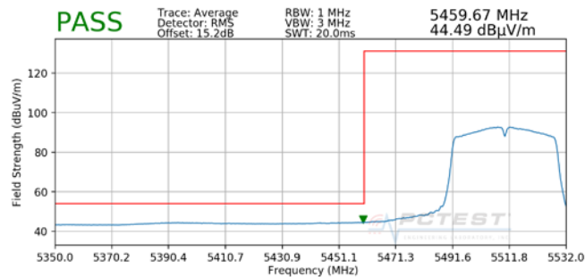
Plot 7-18. Radiated Lower Band Edge Plot (Average – UNII Band 2C)
