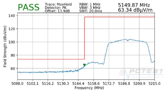
Plot 7-15. Radiated Lower Band Edge Plot (Peak – UNII Band 1)
