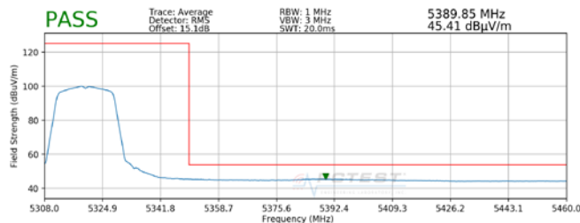
Plot 7-9. Radiated Upper Band Edge Plot (Average – UNII Band 2A)
