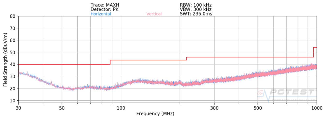
Plot 7-28. Radiated Spurious Plot below 1GHz (802.11a – U3 Ch. 157)
