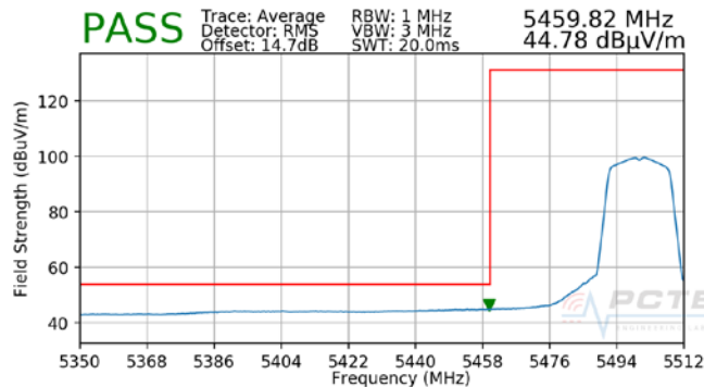
Plot 7-11. Radiated Lower Band Edge Plot (Average – UNII Band 2C)
