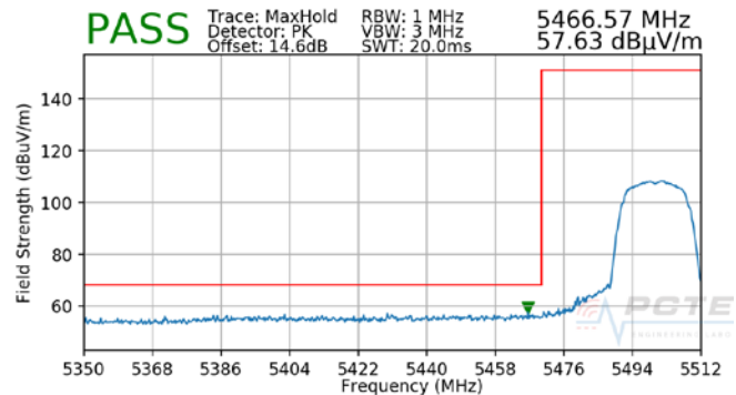
Plot 7-12. Radiated Lower Band Edge Plot (Peak – UNII Band 2C)
