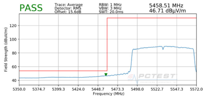
Plot 7-25. Radiated Lower Band Edge Plot (Average – UNII Band 2C)
