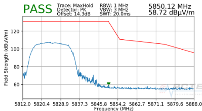
Plot 7-13. Radiated Upper Band Edge Plot (Peak – UNII Band 3)
