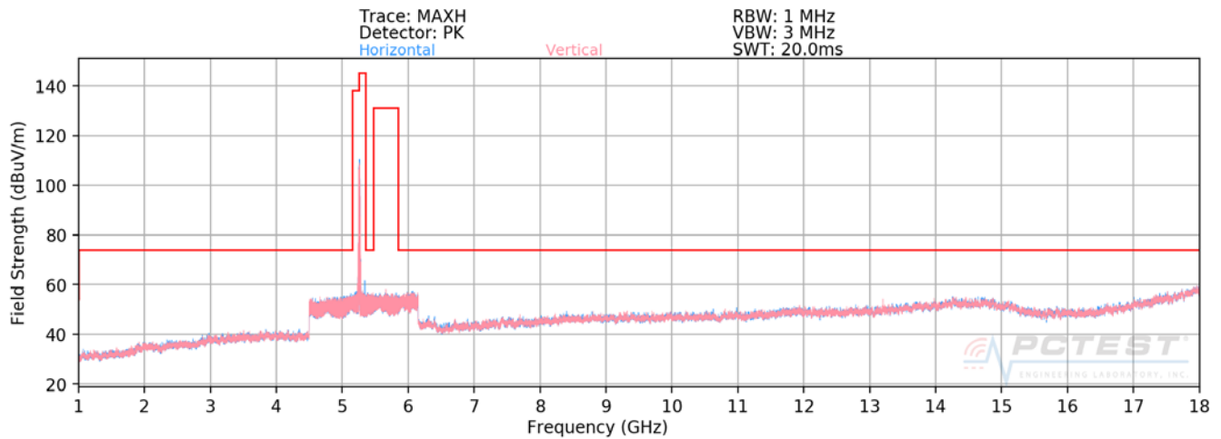
Plot 7-2. Radiated Spurious Plot above 1GHz (802.11a – U2A Ch. 56)
