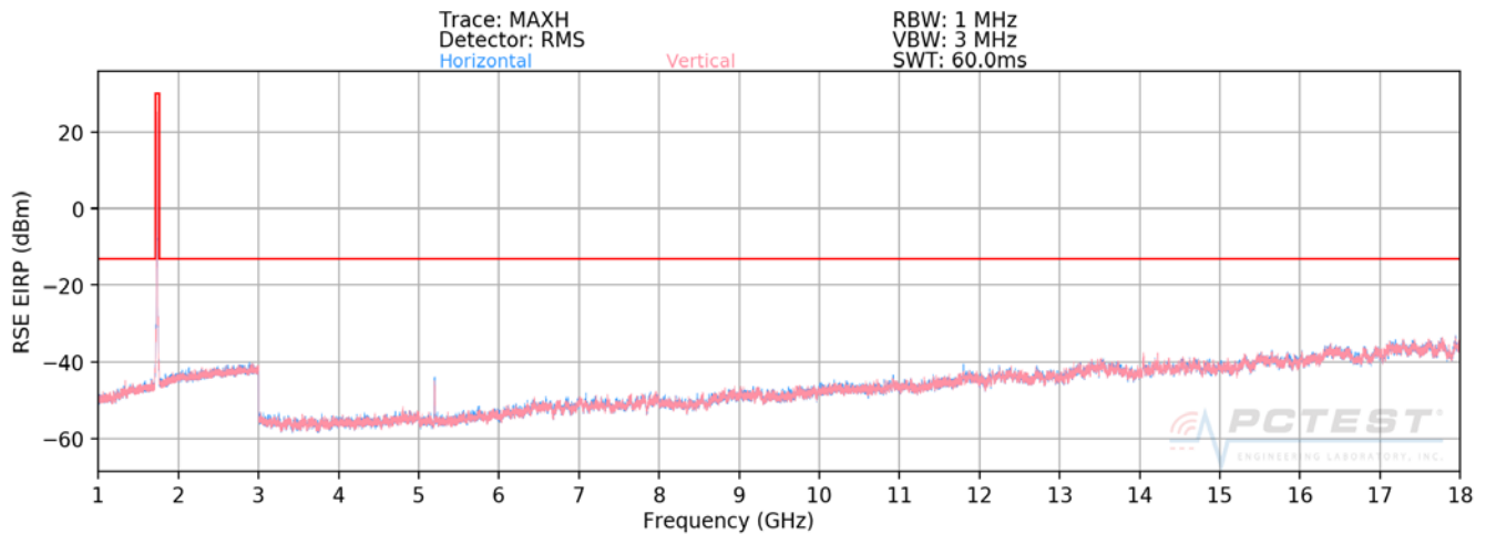
Plot 7-2. Radiated Spurious Plot above 1GHz (AWS WCDMA Mode)
