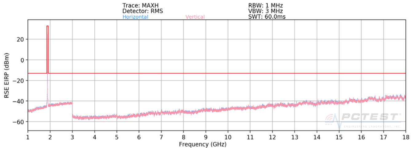
Plot 7-7. Radiated Spurious Plot above 1GHz (PCS WCDMA Mode)
