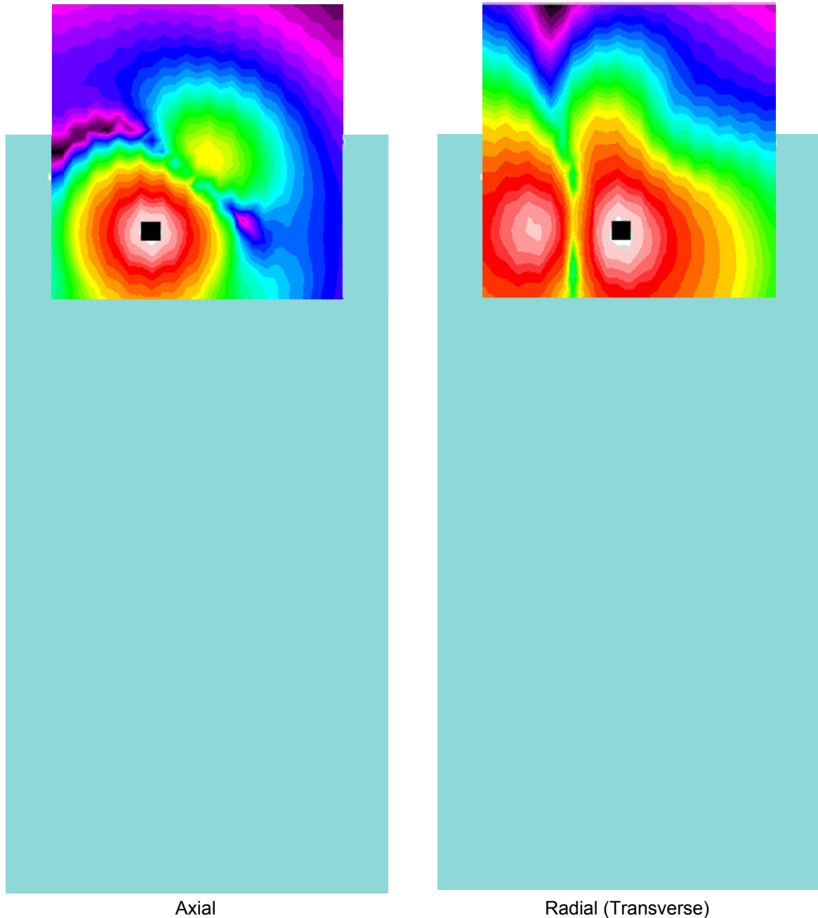
Figure 7-4 T-Coil Scan Overlay Magnetic Field Distributions
