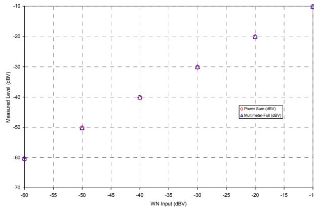
Figure 5-10 ABM2 Power Sum Validation
