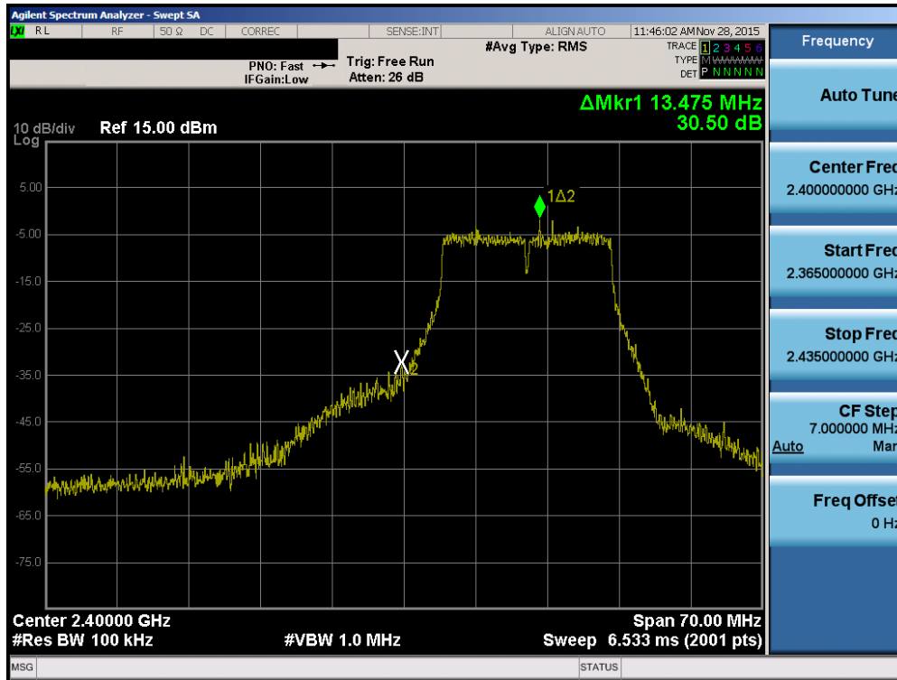
Plot 7-25. Band Edge Plot (802.11g– Ch. 2)
