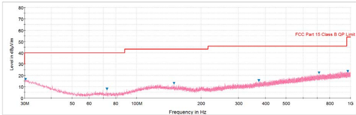
Plot 7-53. Radiated Spurious Plot below 1GHz (Pol. H)
