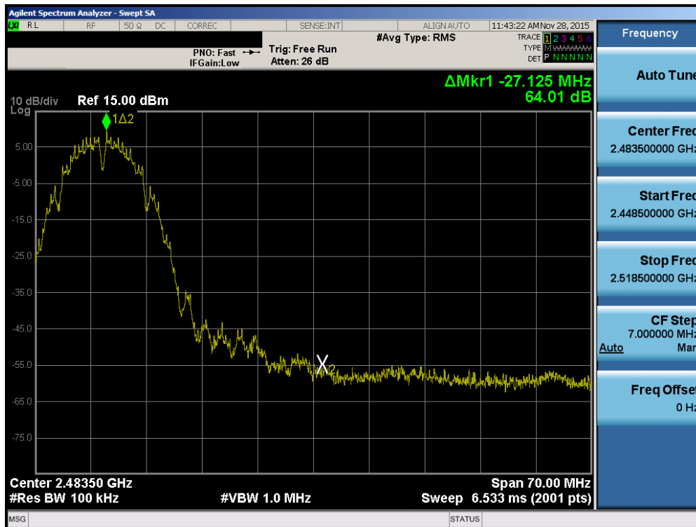
Plot 7-22. Band Edge Plot (802.11b – Ch. 10)
