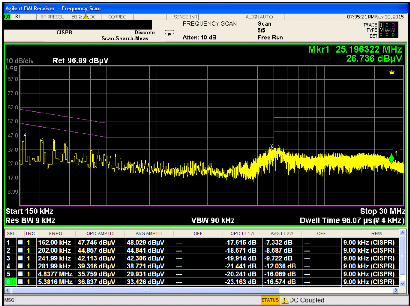
Plot 7-57. Line Conducted Plot with 802.11b (L1) – Travel Adapter S/N EAY64329102
