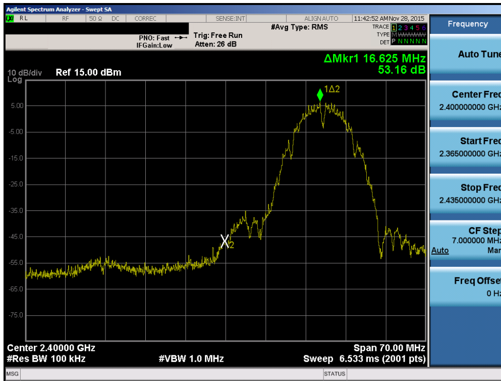
Plot 7-21. Band Edge Plot (802.11b – Ch. 2)
