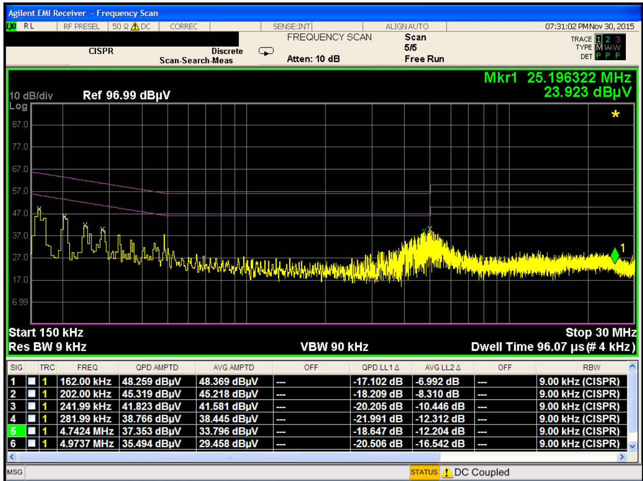
Plot 7-58. Line Conducted Plot with 802.11b (N) – Travel Adapter S/N EAY64329102
