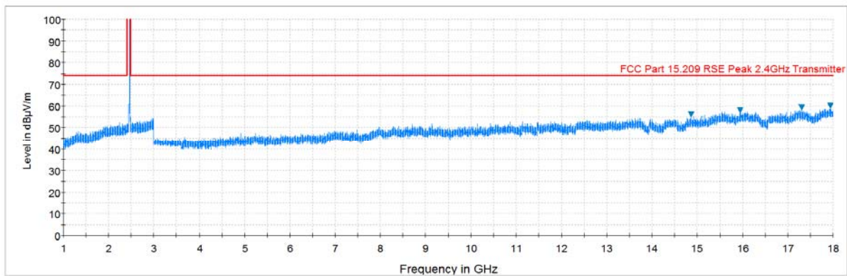
Plot 7-41. Radiated Spurious Plot above 1GHz (802.11b – Ch. 11, Ant. Pol. H)
