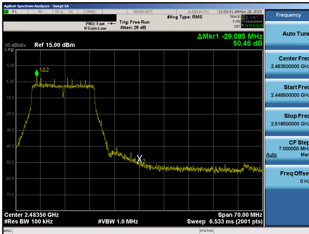
Plot 7-30. Band Edge Plot (802.11n (2.4GHz) – Ch. 10)
