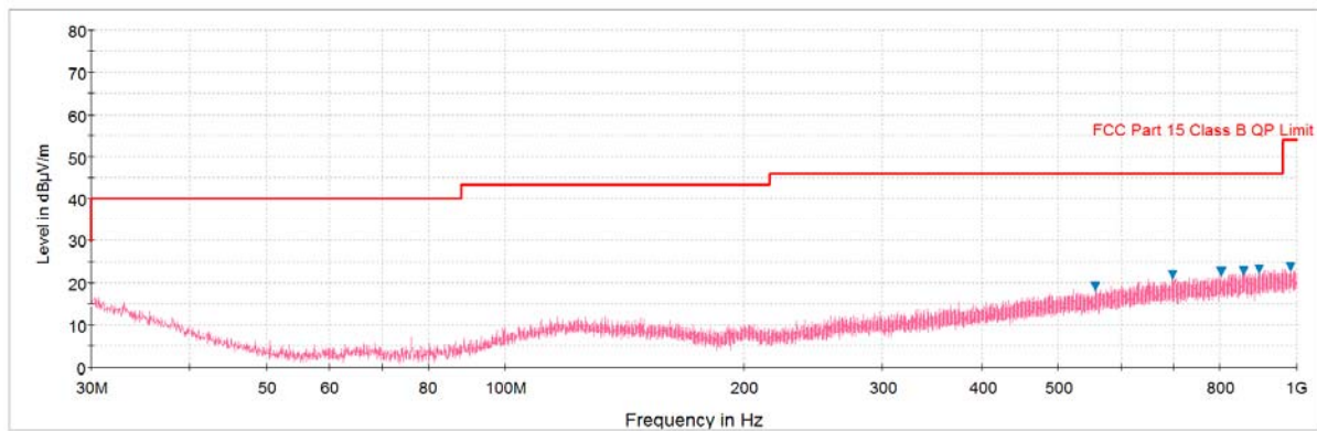
Plot 7-54. Radiated Spurious Plot below 1GHz (Pol. V)
