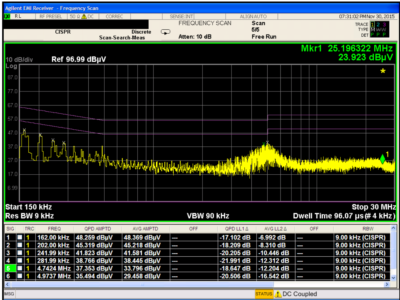
Plot 7-56. Line Conducted Plot with 802.11b (N)
