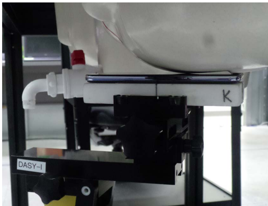
SAR Test Setup Photo 1: Left Cheek
