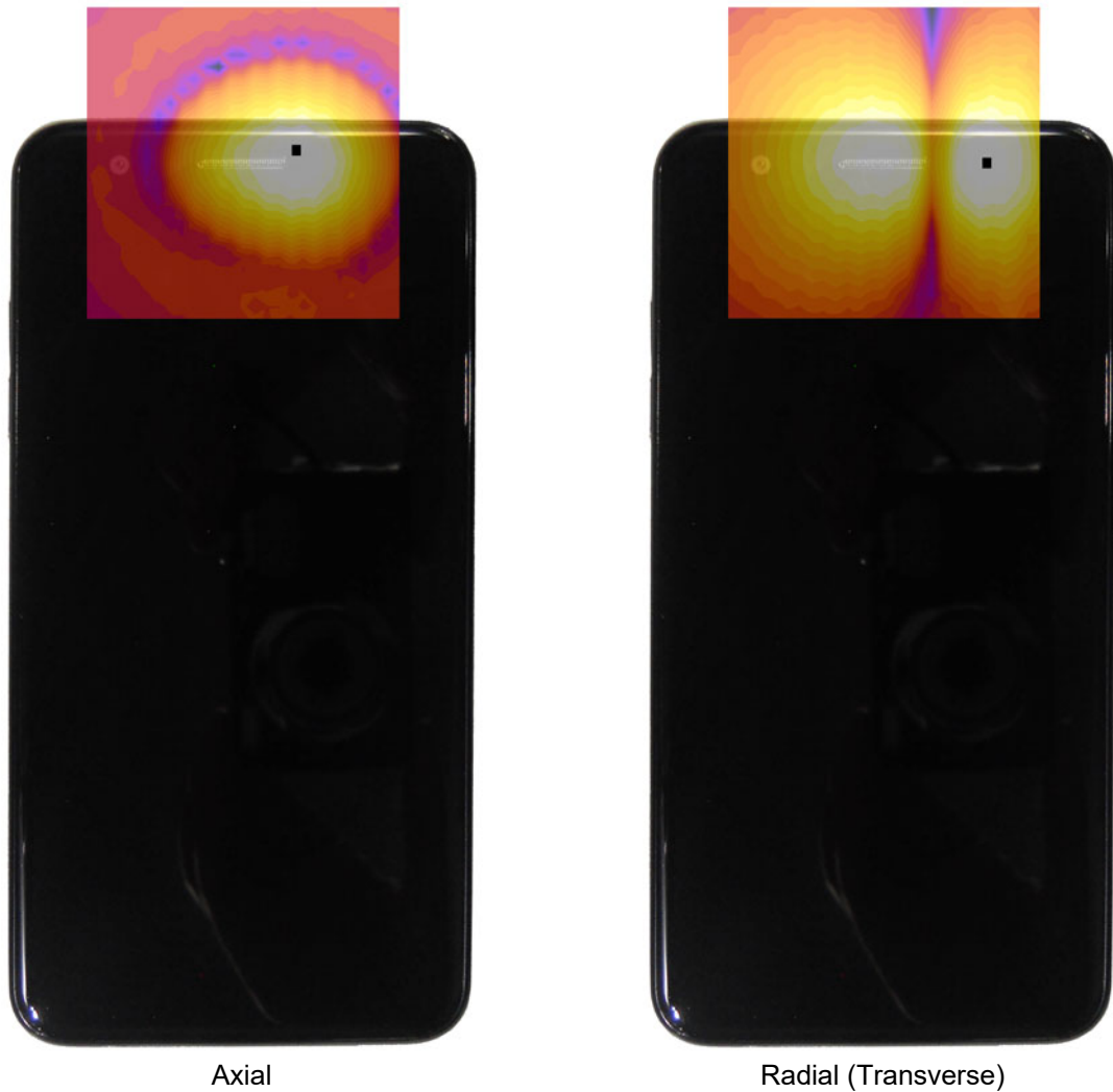
Figure 16-3 T-Coil Scan Overlay Magnetic Field Distributions
