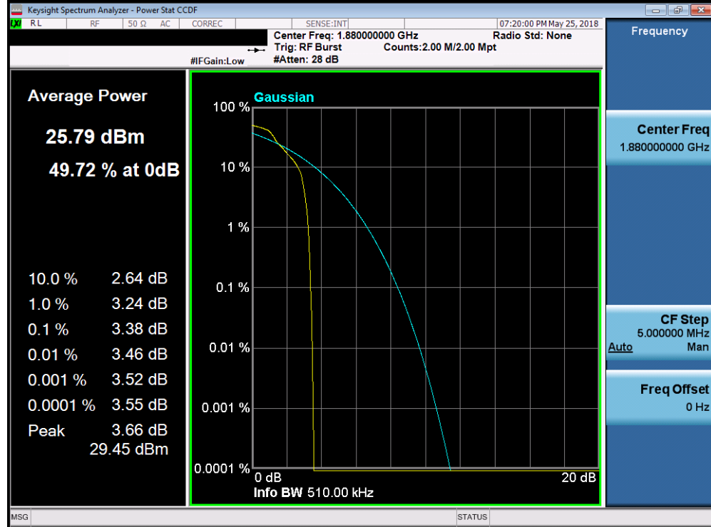
Plot 7-96. Peak-Average Ratio Plot (PCS EDGE Mode)
