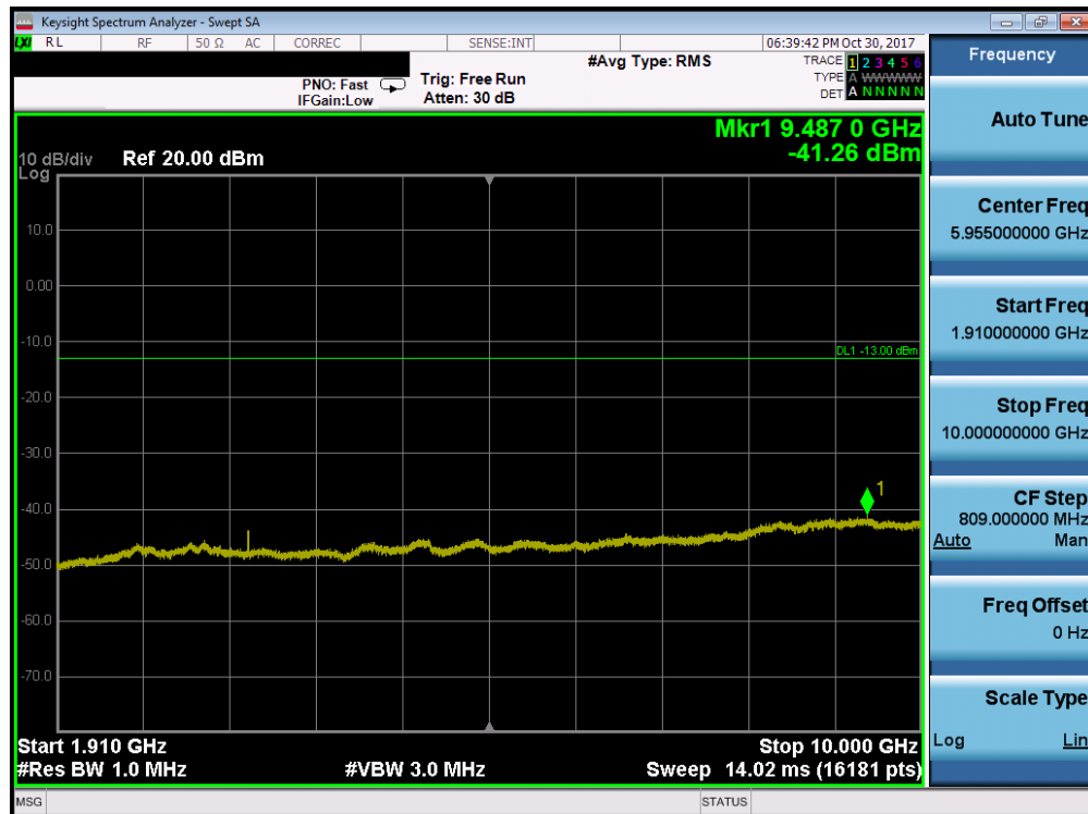
Plot 7-75. Conducted Spurious Plot (Band 2 - 10.0MHz QPSK - RB Size 1, RB Offset 0 - Low Channel)
