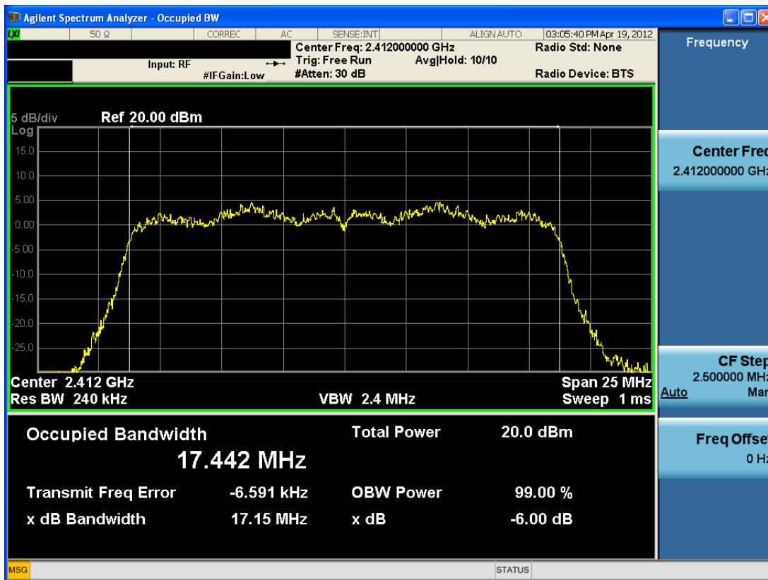
Plot 6-7. 6dB Bandwidth Plot (802.11n – Ch. 1)
