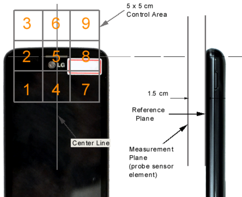
Figure 18-3 5x5 Scan grid above WD (Ear Reference Point centered scan grid shown)
