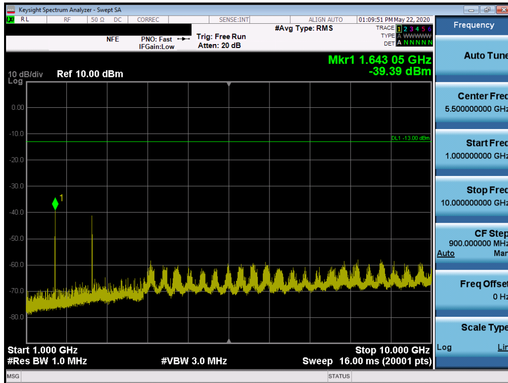
Plot 7-20. Conducted Spurious Plot (LTE Band 26 - 15MHz QPSK - RB Size 1, RB Offset 0 - Mid Channel)
