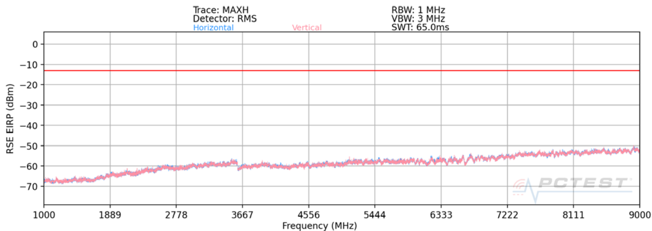
Plot 7-32. Radiated Spurious Plot (LTE Band 26)
