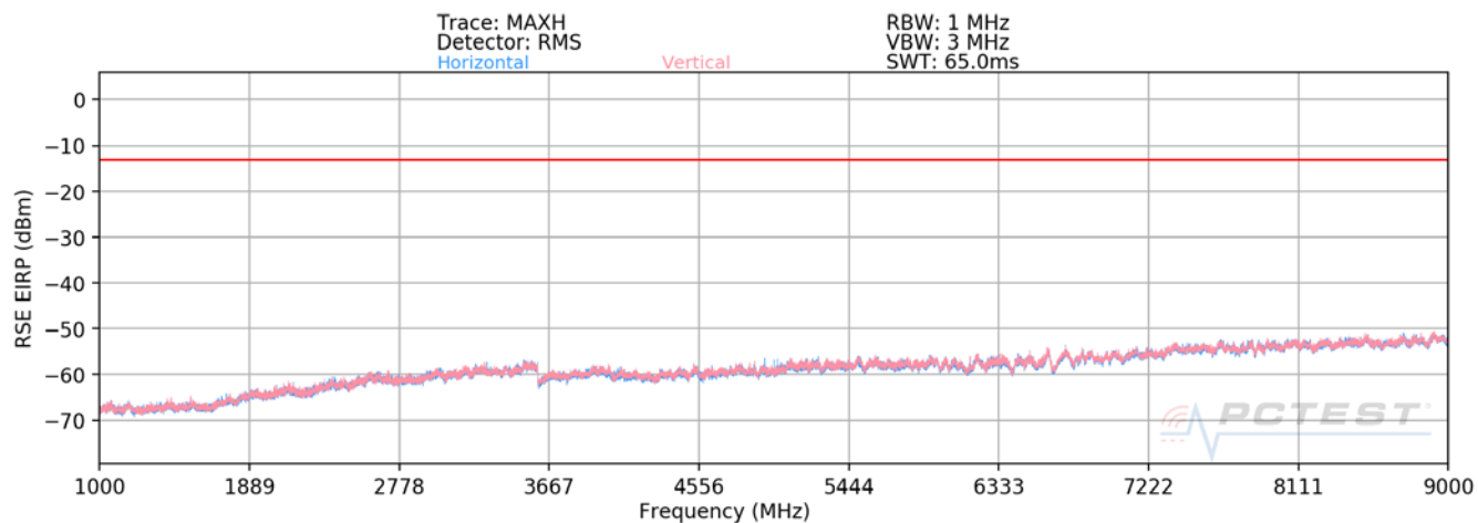
Plot 7-33. Radiated Spurious Plot (CDMA BC10)
