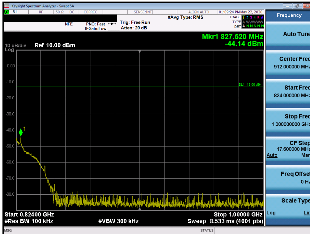
Plot 7-19. Conducted Spurious Plot (LTE Band 26 - 15MHz QPSK - RB Size 1, RB Offset 0 - Mid Channel)
