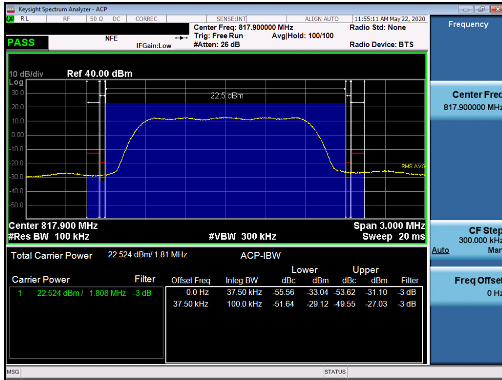
Plot 7-29. Channel Edge Plot (CDMA BC10 – Ch. 476)
