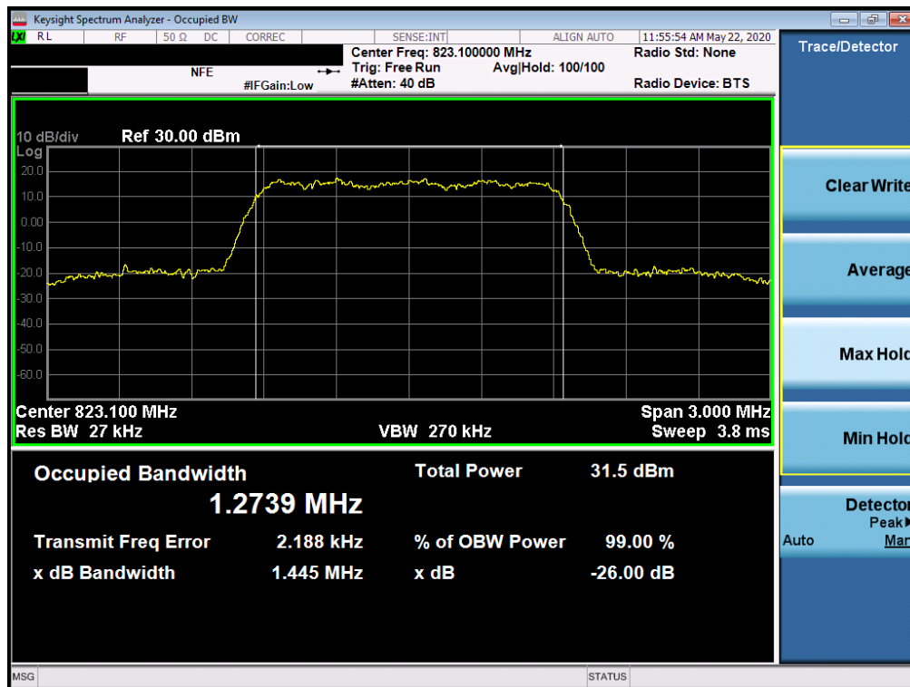
Plot 7-17. Occupied Bandwidth Plot (CDMA, Ch. 684)
