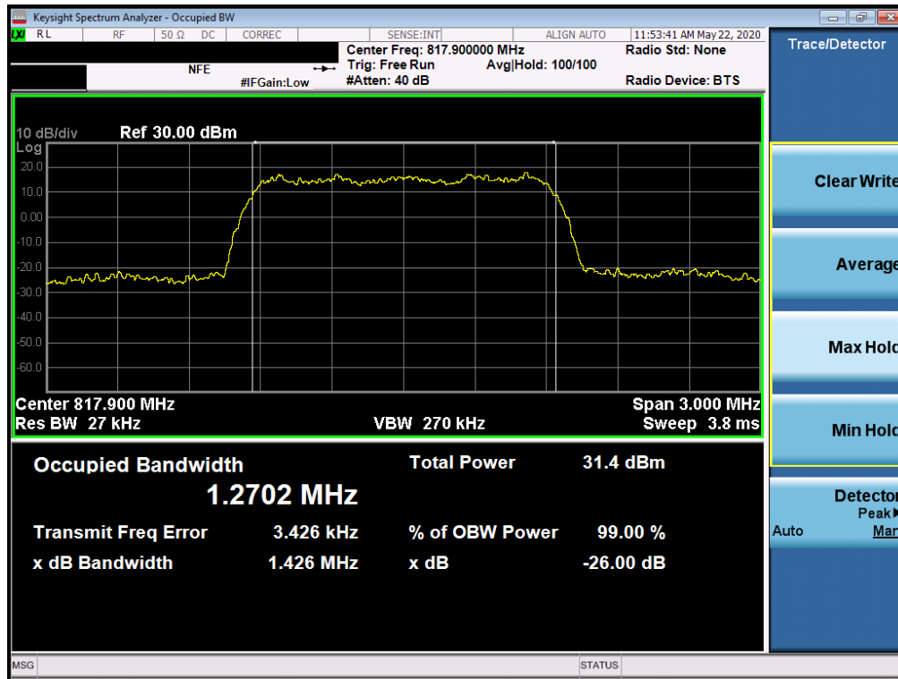
Plot 7-16. Occupied Bandwidth Plot (CDMA, Ch. 476)
