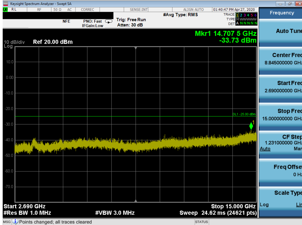
Plot 7-29. Conducted Spurious Plot (LTE Band 41(PC2) - 20MHz QPSK - RB Size 1, RB Offset 0 - Mid Channel)
