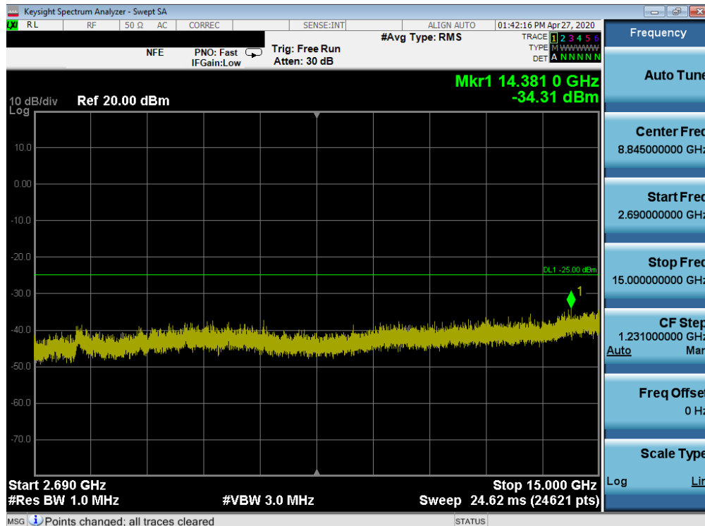
Plot 7-26. Conducted Spurious Plot (LTE Band 41(PC2) - 20MHz QPSK - RB Size 1, RB Offset 0 - Low Channel)
