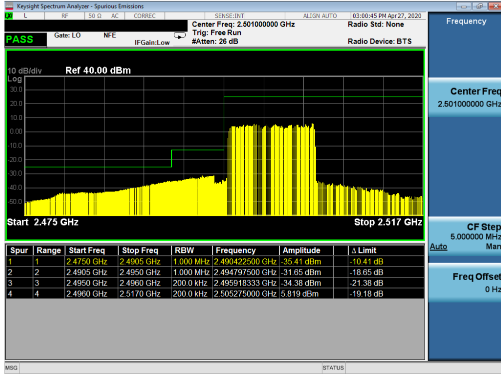
Plot 7-55. Lower ACP Plot (LTE Band 41(PC3) - 10MHz QPSK – Full RB Configuration)
