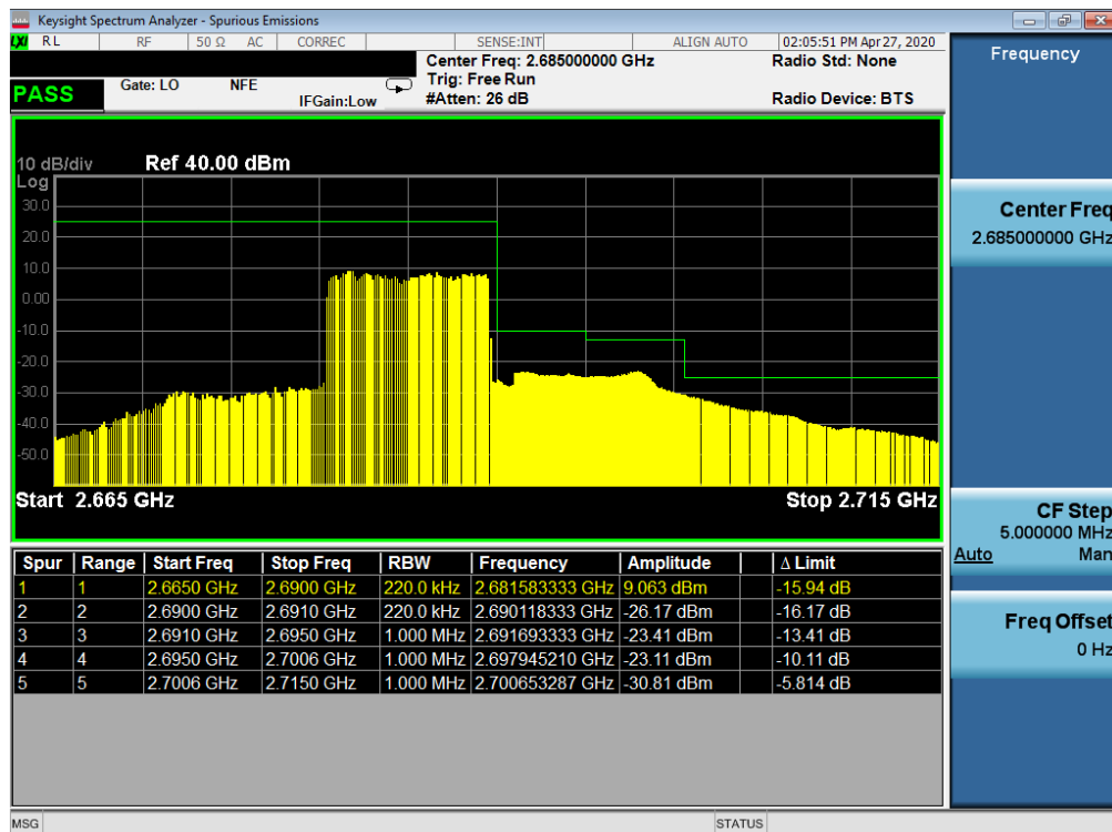
Plot 7-48. Upper ACP Plot (LTE Band 41(PC2) - 10MHz QPSK – Full RB Configuration)
