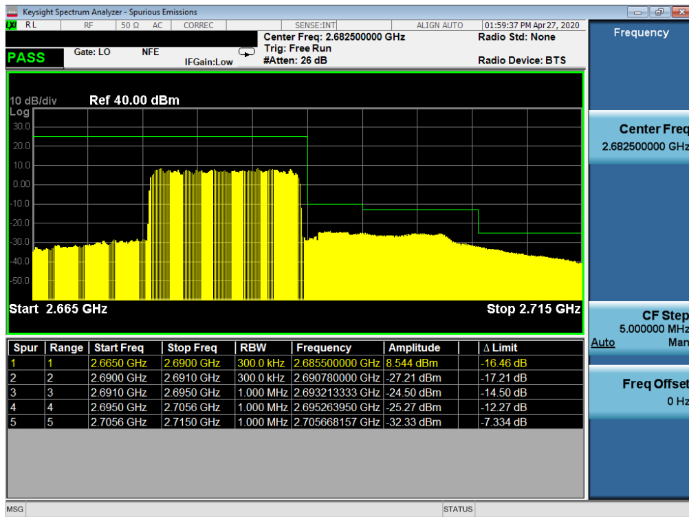
Plot 7-46. Upper ACP Plot (LTE Band 41(PC2) - 15MHz QPSK – Full RB Configuration)
