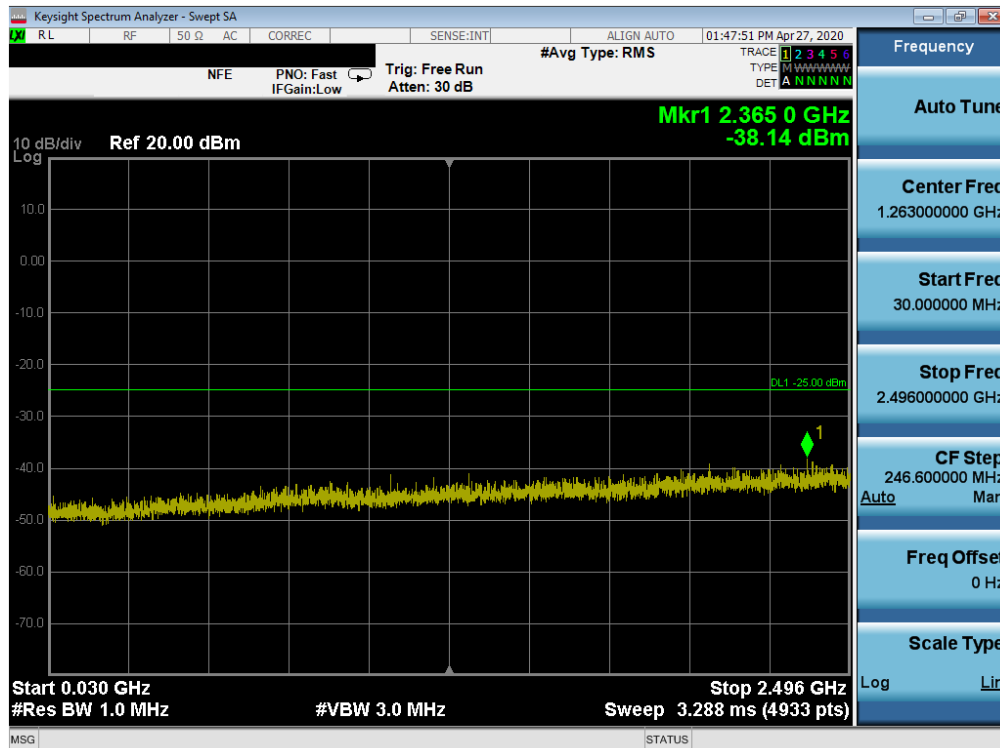
Plot 7-31. Conducted Spurious Plot (LTE Band 41(PCA) - 20MHz QPSK - RB Size 1, RB Offset 0 - High Channel)
