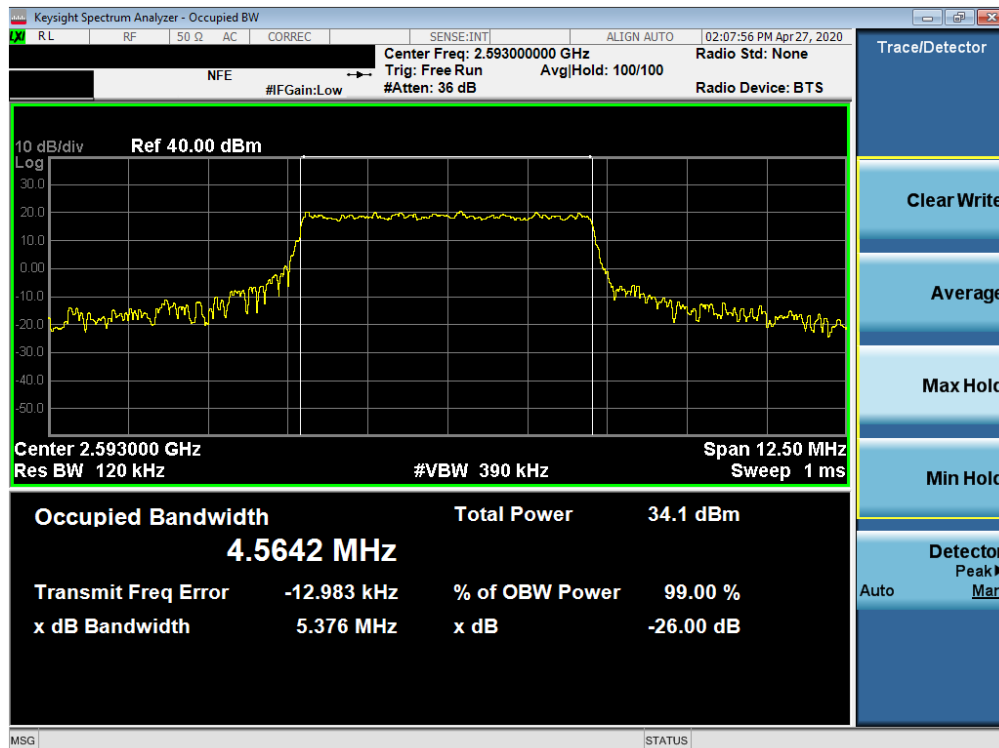
Plot 7-10. Occupied Bandwidth Plot (LTE Band 41(PC2) - 5MHz QPSK - Full RB Configuration)
