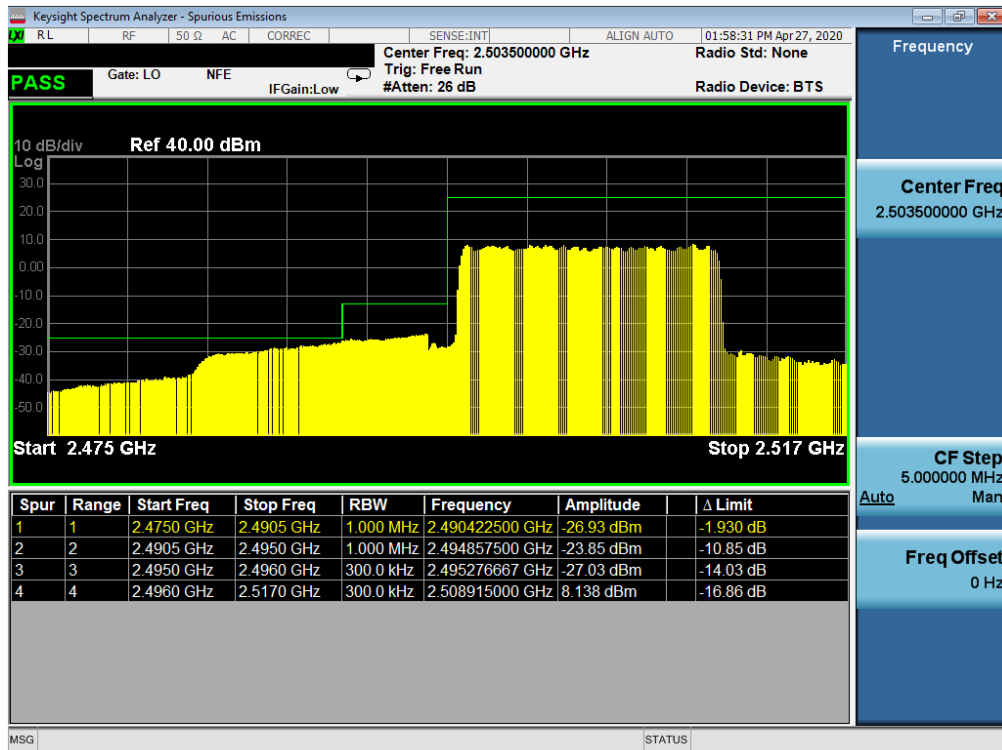
Plot 7-45. Lower ACP Plot (LTE Band 41(PC2) - 15MHz QPSK – Full RB Configuration)
