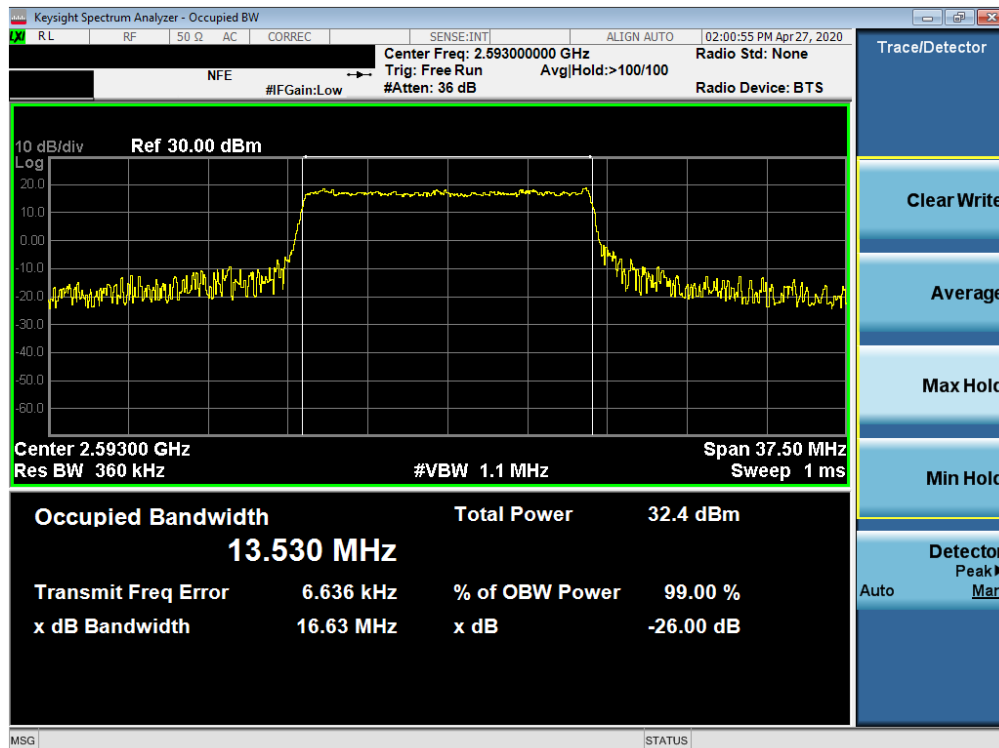
Plot 7-6. Occupied Bandwidth Plot (LTE Band 41(PC2) - 15MHz 64-QAM - Full RB Configuration)
