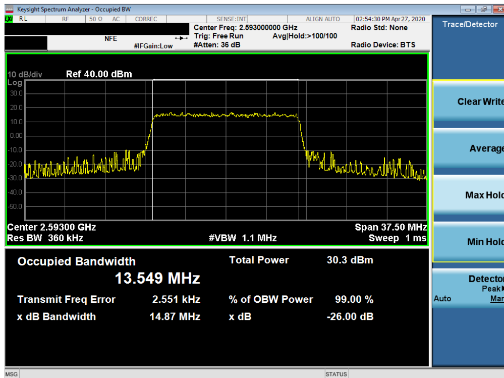
Plot 7-17. Occupied Bandwidth Plot (LTE Band 41(PC3) - 15MHz 16-QAM - Full RB Configuration)
