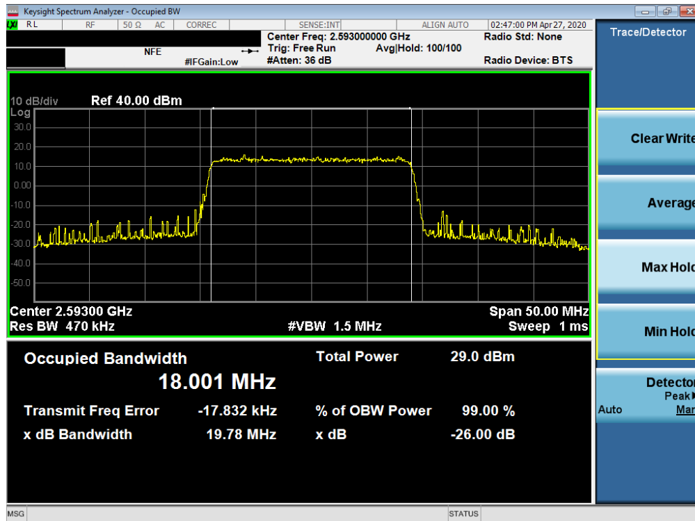
Plot 7-15. Occupied Bandwidth Plot (LTE Band 41(PC3) - 20MHz 64-QAM - Full RB Configuration)
