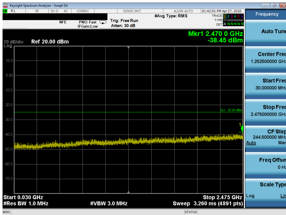
Plot 7-25. Conducted Spurious Plot (LTE Band 41(PC2) - 20MHz QPSK - RB Size 1, RB Offset 0 - Low Channel)
