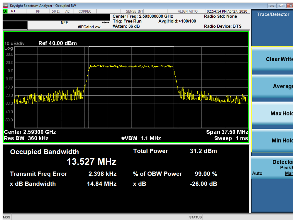
Plot 7-16. Occupied Bandwidth Plot (LTE Band 41(PC3) - 15MHz QPSK - Full RB Configuration)
