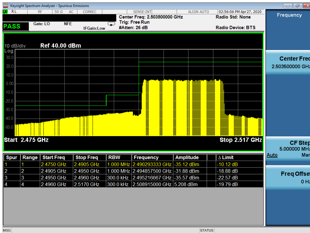
Plot 7-53. Lower ACP Plot (LTE Band 41(PC3) - 15MHz QPSK – Full RB Configuration)
