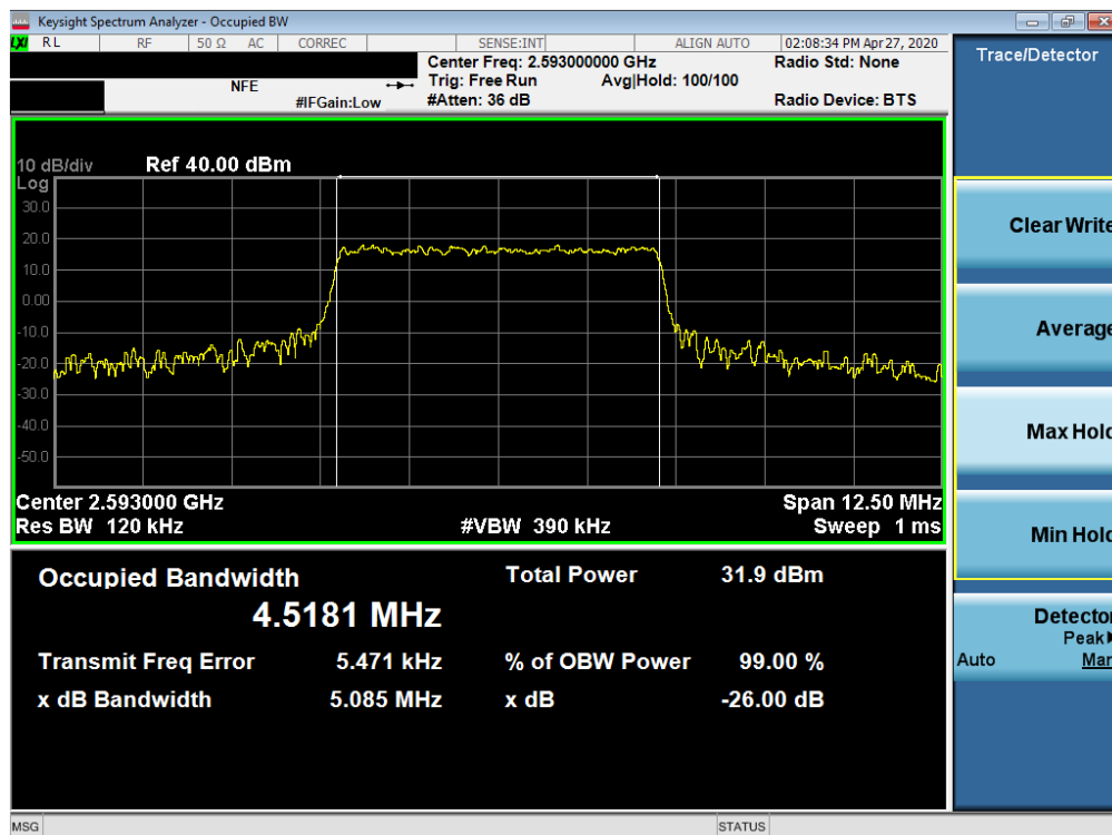
Plot 7-12. Occupied Bandwidth Plot (LTE Band 41(PC2) - 5MHz 64-QAM - Full RB Configuration)
