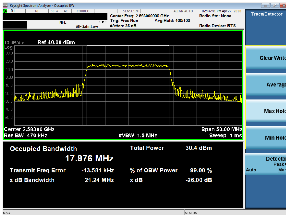
Plot 7-14. Occupied Bandwidth Plot (LTE Band 41(PC3) - 20MHz 16-QAM - Full RB Configuration)
