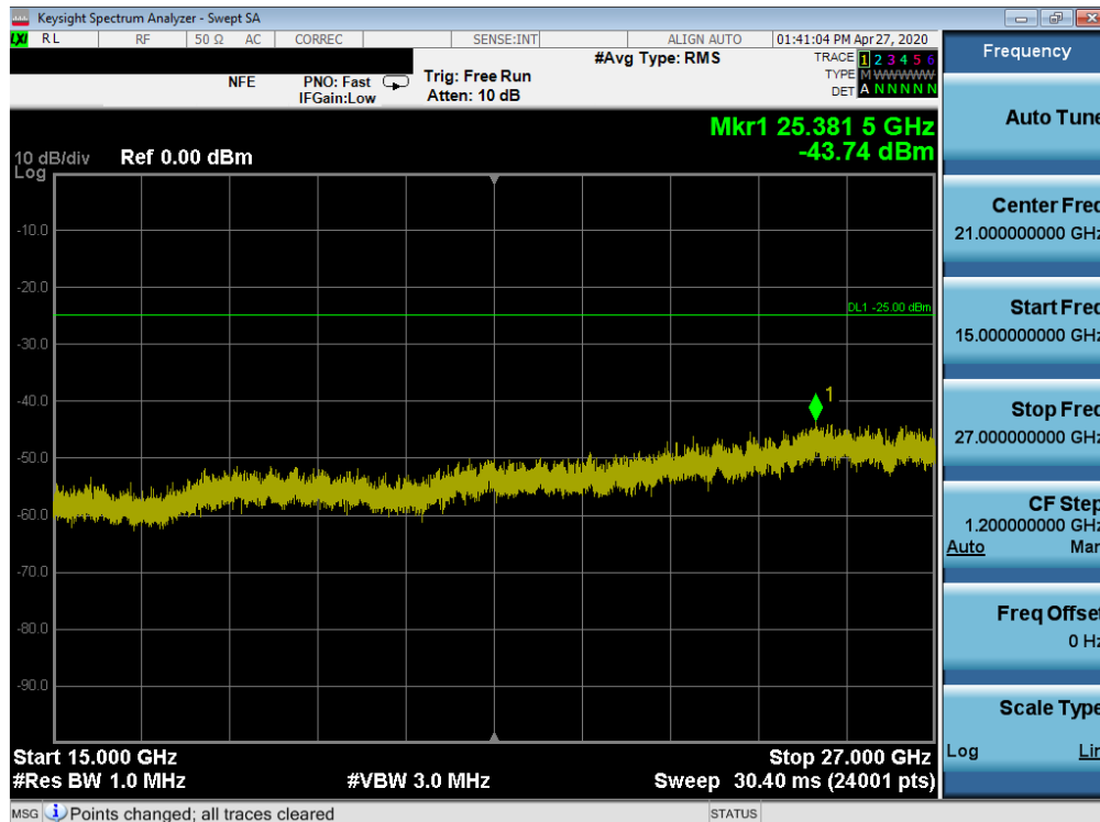
Plot 7-30. Conducted Spurious Plot (LTE Band 41(PC2) - 20MHz QPSK - RB Size 1, RB Offset 0 - Mid Channel)
