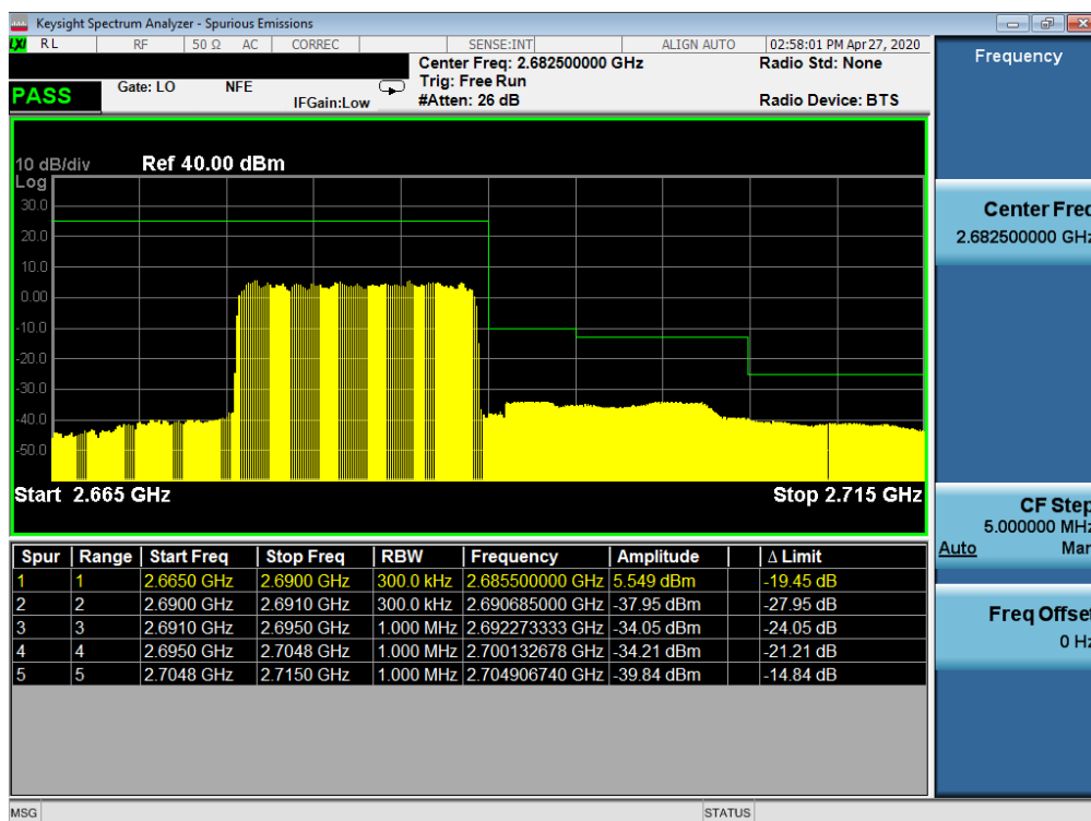
Plot 7-54. Upper ACP Plot (LTE Band 41(PC3) - 15MHz QPSK – Full RB Configuration)
