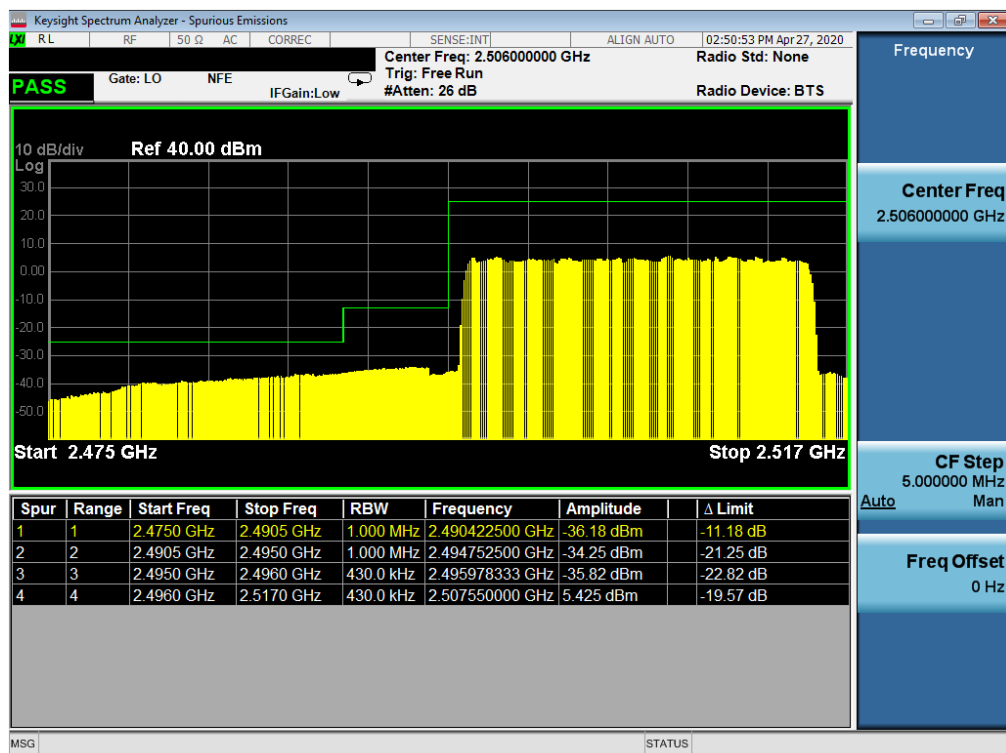
Plot 7-51. Lower ACP Plot (LTE Band 41(PC3) - 20MHz QPSK – Full RB Configuration)
