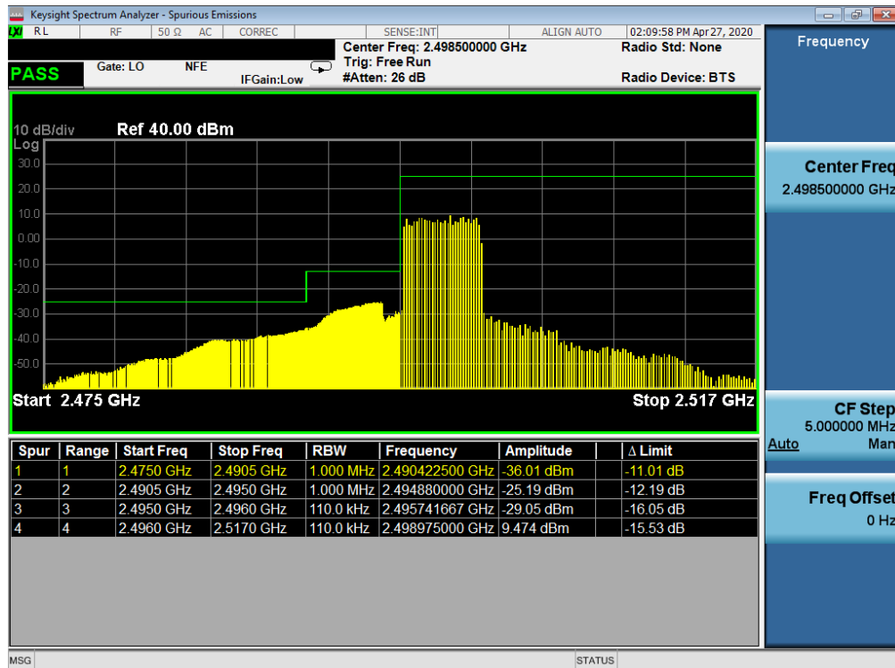
Plot 7-49. Lower ACP Plot (LTE Band 41(PC2) - 5MHz QPSK – Full RB Configuration)
