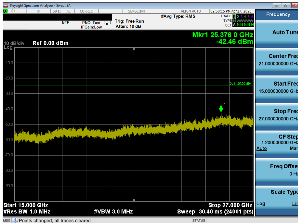
Plot 7-36. Conducted Spurious Plot (LTE Band 41(PC3) - 20MHz QPSK - RB Size 1, RB Offset 0 - Low Channel)
