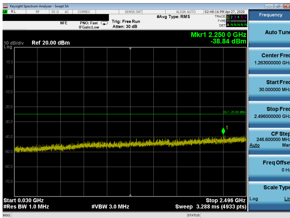
Plot 7-37. Conducted Spurious Plot (LTE Band 41(PC3) - 20MHz QPSK - RB Size 1, RB Offset 0 - Mid Channel)
