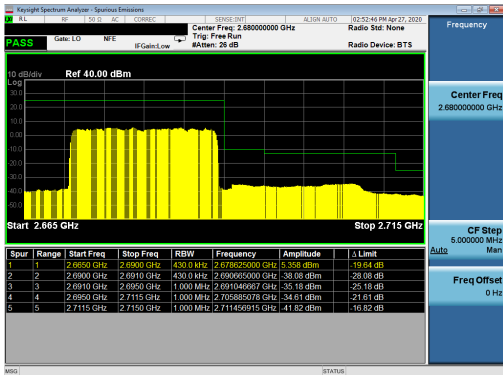
Plot 7-52. Upper ACP Plot (LTE Band 41(PC3) - 20MHz QPSK – Full RB Configuration)
