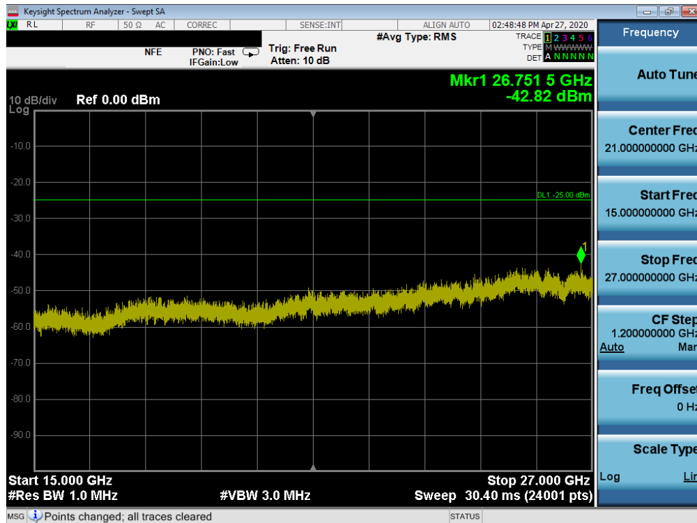
Plot 7-39. Conducted Spurious Plot (LTE Band 41(PC3) - 20MHz QPSK - RB Size 1, RB Offset 0 - Mid Channel)
