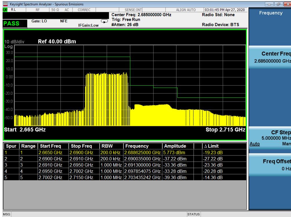
Plot 7-56. Upper ACP Plot (LTE Band 41(PC3) - 10MHz QPSK – Full RB Configuration)
