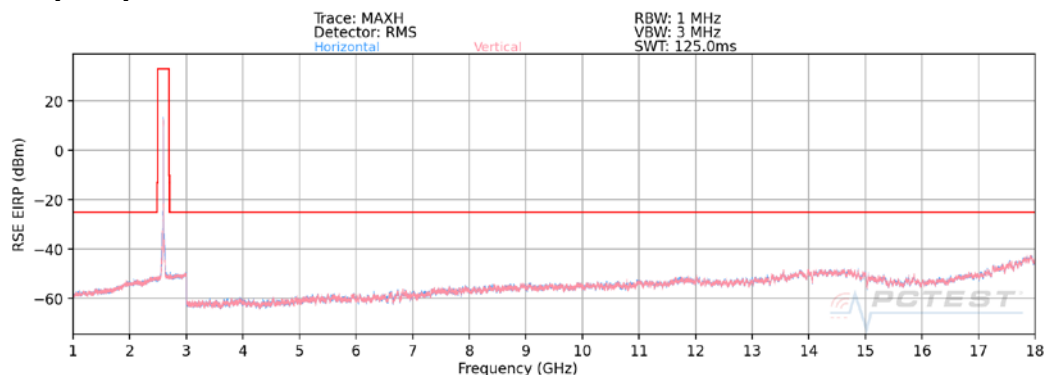
Plot 7-60. Radiated Spurious Plot (LTE Band 41(PC2))
