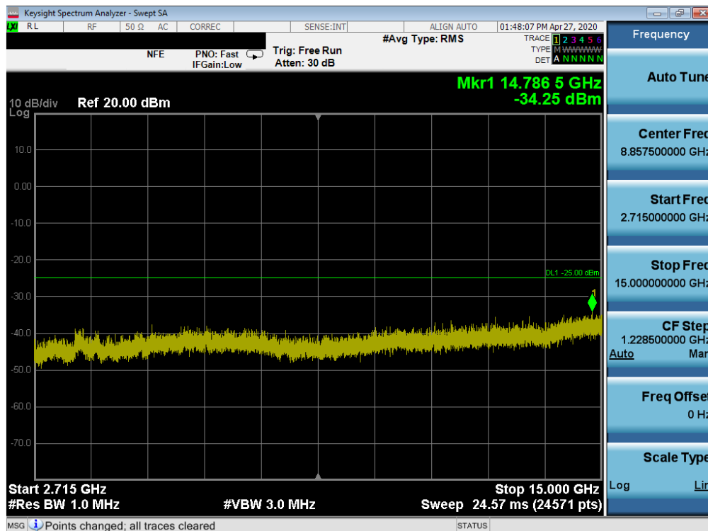
Plot 7-32. Conducted Spurious Plot (LTE Band 41(PCA) - 20MHz QPSK - RB Size 1, RB Offset 0 - High Channel)
