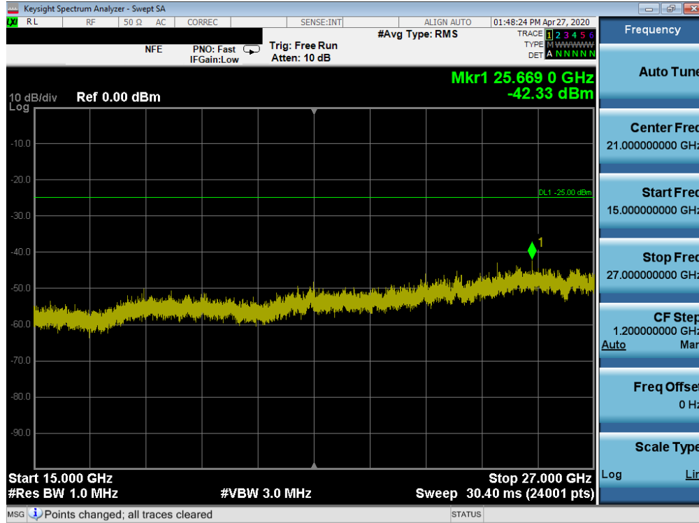
Plot 7-33. Conducted Spurious Plot (LTE Band 41(PC2) - 20MHz QPSK - RB Size 1, RB Offset 0 - High Channel)
