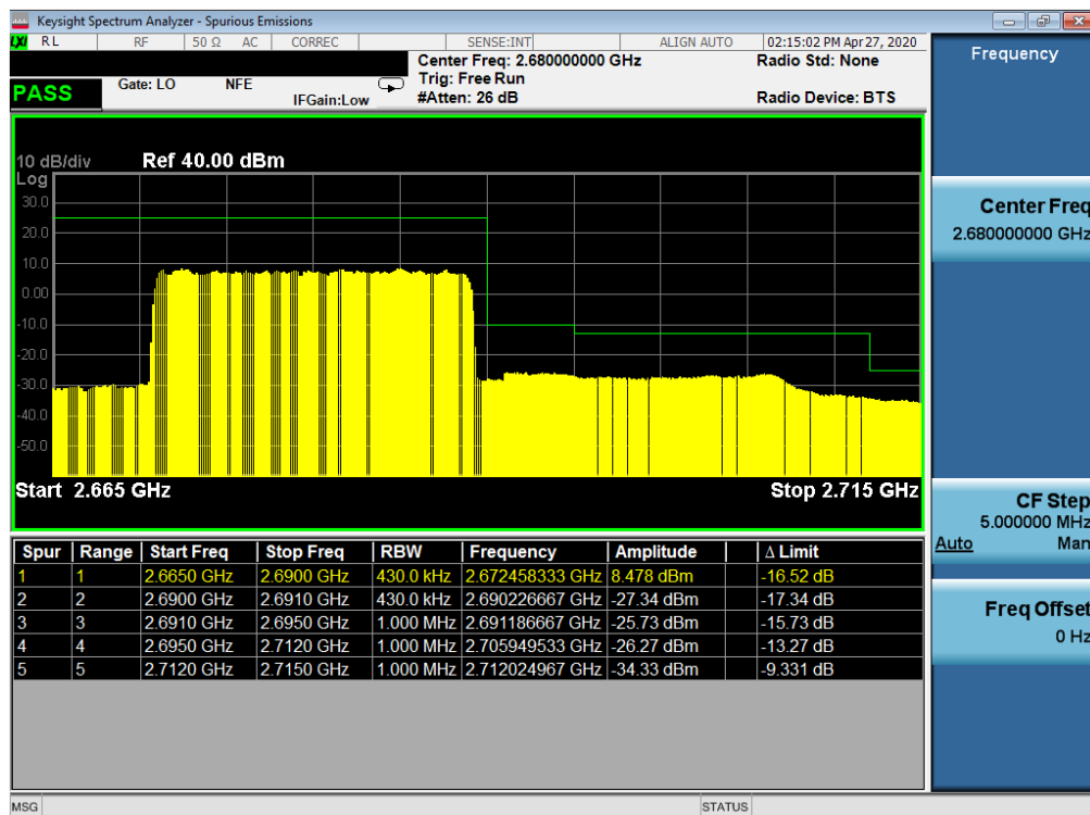
Plot 7-44. Upper ACP Plot (LTE Band 41(PC2) - 20MHz QPSK – Full RB Configuration)
