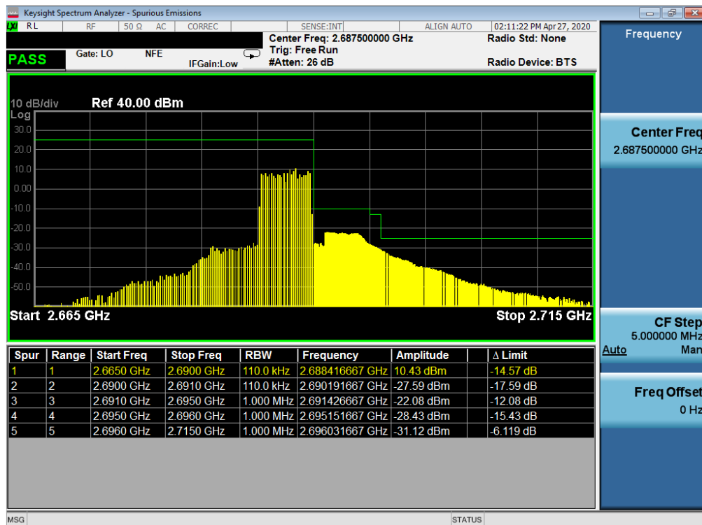
Plot 7-50. Upper ACP Plot (LTE Band 41(PC2) - 5MHz QPSK – Full RB Configuration)
