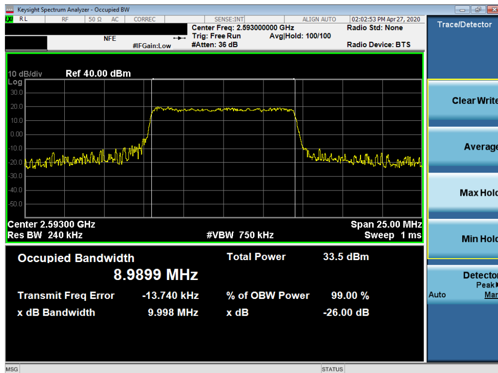
Plot 7-8. Occupied Bandwidth Plot (LTE Band 41(PC2) - 10MHz 16-QAM - Full RB Configuration)
