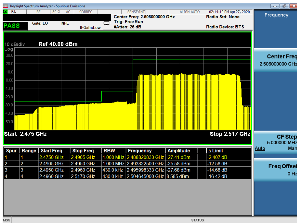
Plot 7-43. Lower ACP Plot (LTE Band 41(PC2) - 20MHz QPSK – Full RB Configuration)
