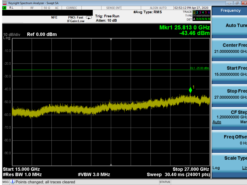
Plot 7-42. Conducted Spurious Plot (LTE Band 41(PC3) - 20MHz QPSK - RB Size 1, RB Offset 0 - High Channel)
