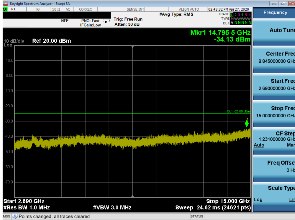
Plot 7-38. Conducted Spurious Plot (LTE Band 41(PC3) - 20MHz QPSK - RB Size 1, RB Offset 0 - Mid Channel)
