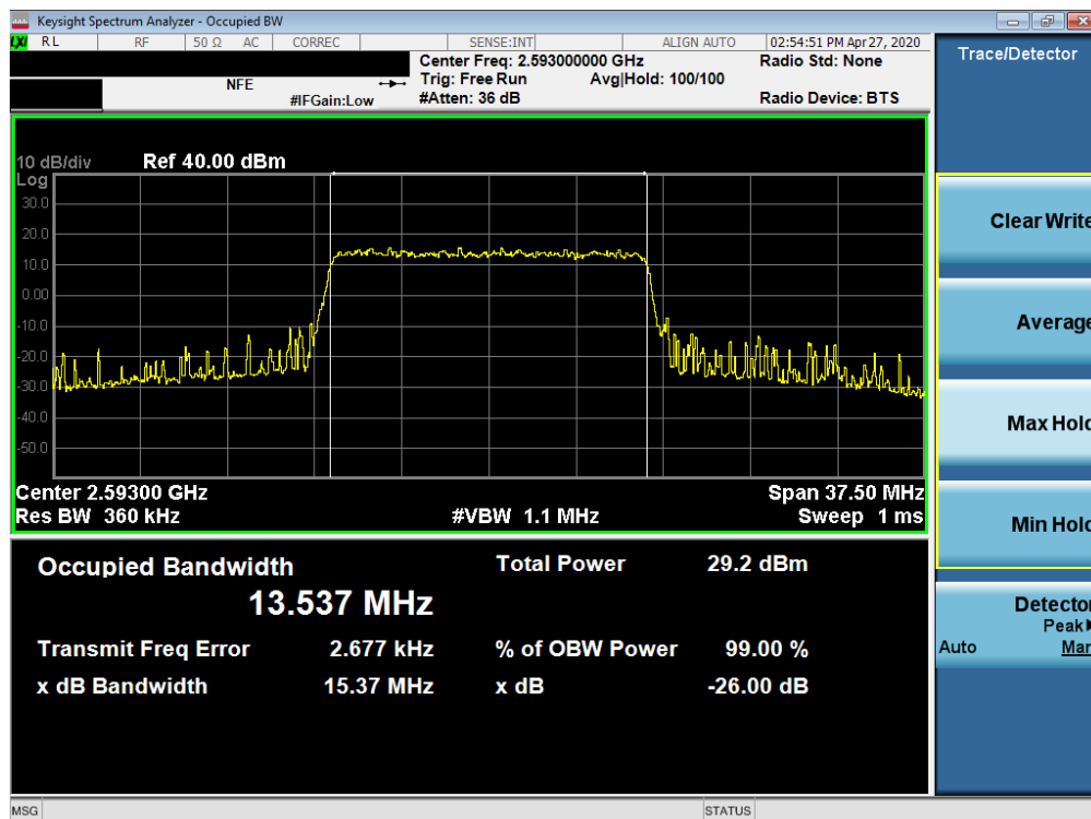
Plot 7-18. Occupied Bandwidth Plot (LTE Band 41(PC3) - 15MHz 64-QAM - Full RB Configuration)
