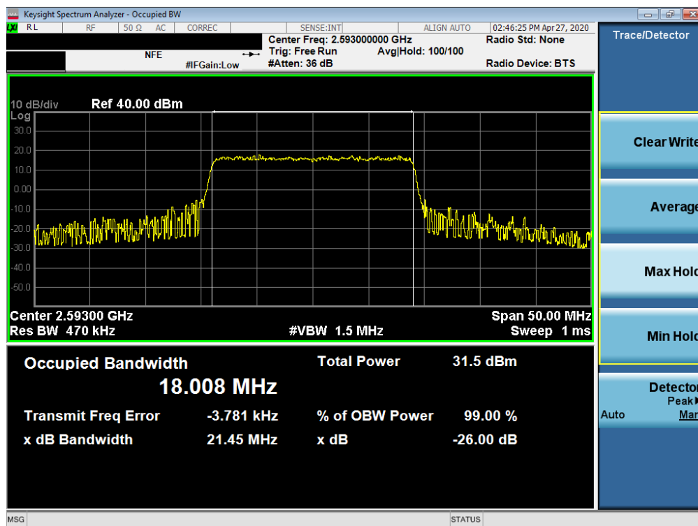
Plot 7-13. Occupied Bandwidth Plot (LTE Band 41(PC3) - 20MHz QPSK - Full RB Configuration)
