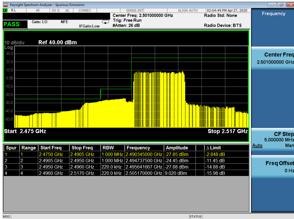
Plot 7-47. Lower ACP Plot (LTE Band 41(PC2) - 10MHz QPSK – Full RB Configuration)
