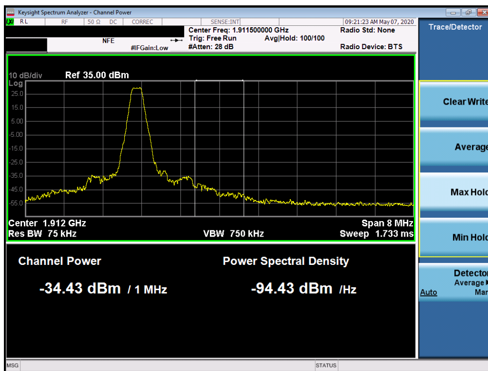
Plot 7-71. Extended Upper Band Edge Plot (GPRS PCS – Ch. 810)
