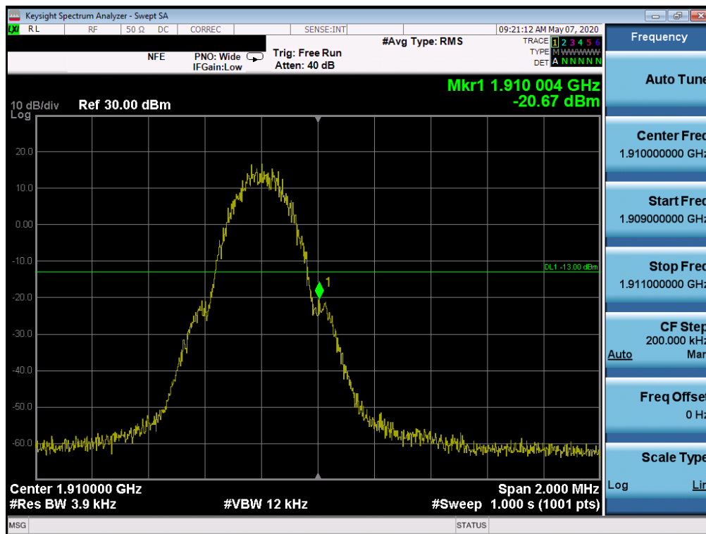
Plot 7-70. Upper Band Edge Plot (GPRS PCS – Ch. 810)
