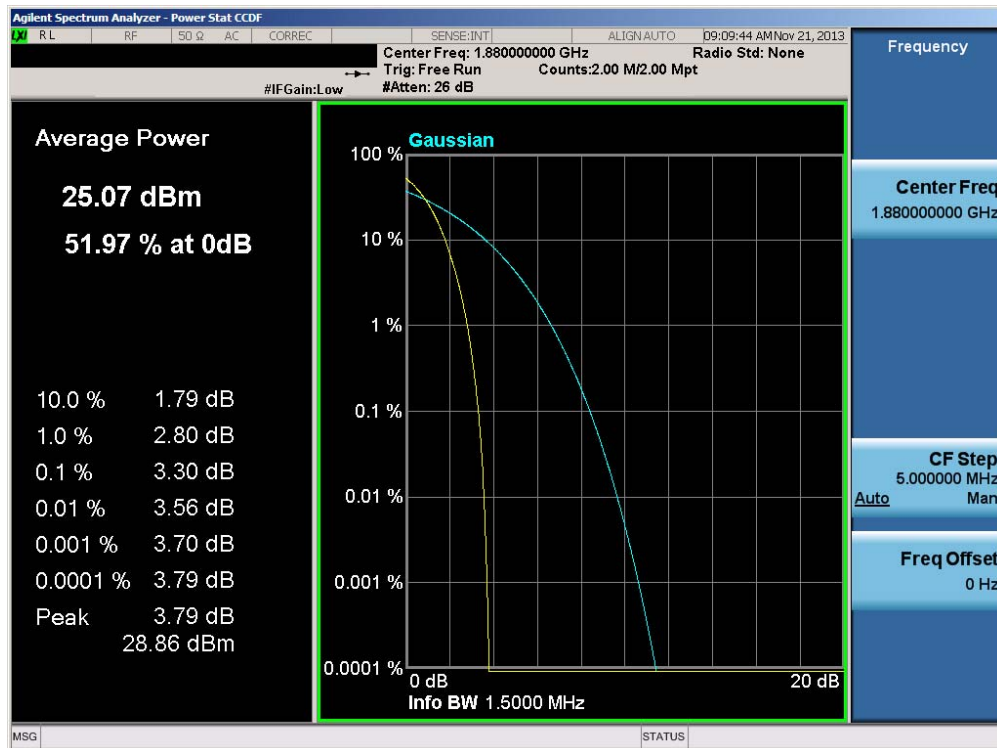
Plot 6-24. Peak-Average Ratio Plot (PCS CDMA Mode – Ch. 600)
