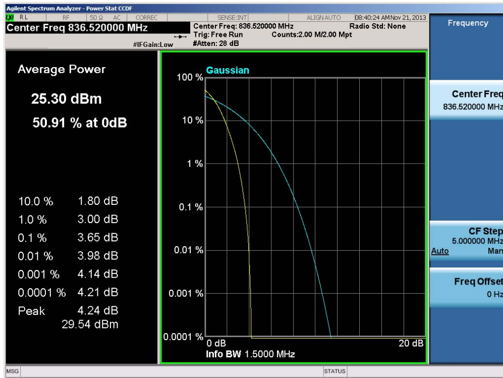
Plot 6-23. Peak-Average Ratio Plot (Cellular CDMA Mode – Ch. 384)
