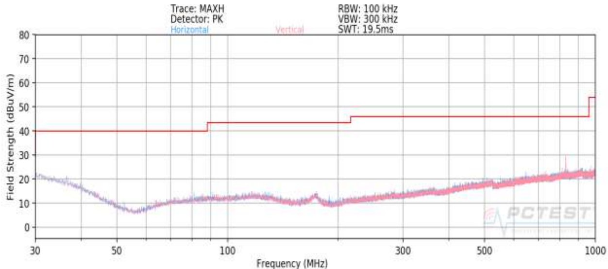
Plot 7-13. Radiated Spurious Plot below 1GHz
