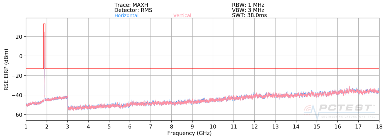
Plot 7-6. Radiated Spurious Plot above 1GHz (Band 2)
