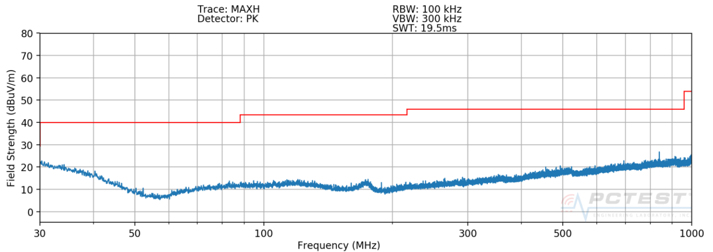
Plot 7-31. Radiated Spurious Plot below 1GHz
