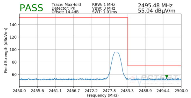
Plot 7-30. Radiated Restricted Upper Band Edge Measurement (Peak)
