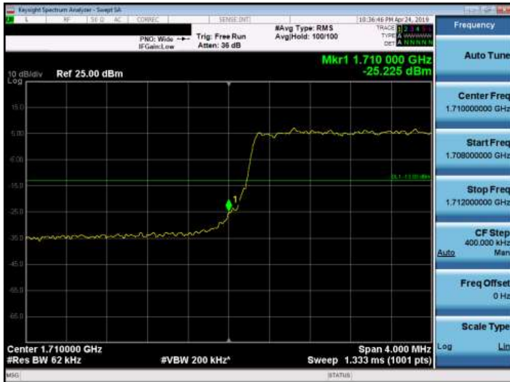
Plot 7-150. Lower Band Edge Plot (Band 66/4 - 5.0MHz QPSK - Full RB Configuration)
