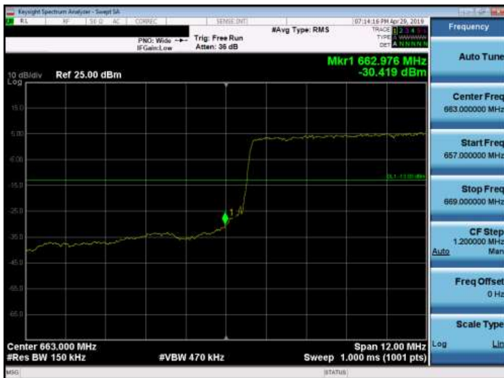
Plot 7-108. Lower Band Edge Plot (Band 71 - 15.0MHz QPSK - Full RB Configuration)
