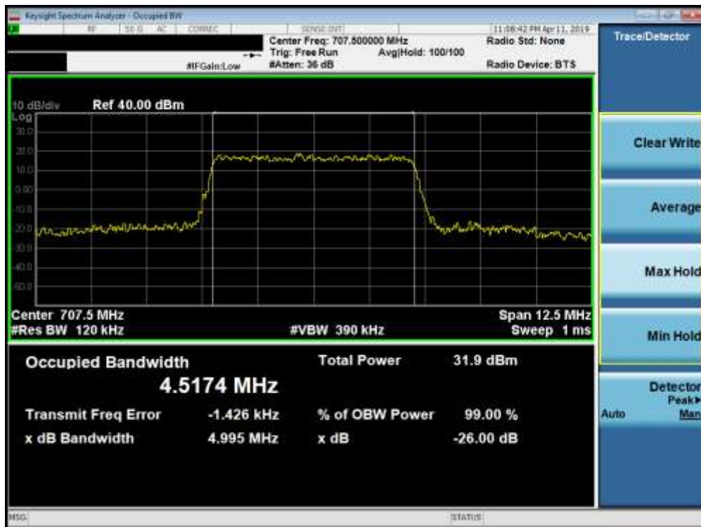
Plot 7-13. Occupied Bandwidth Plot (Band 12/17 - 5.0MHz QPSK - Full RB Configuration)
