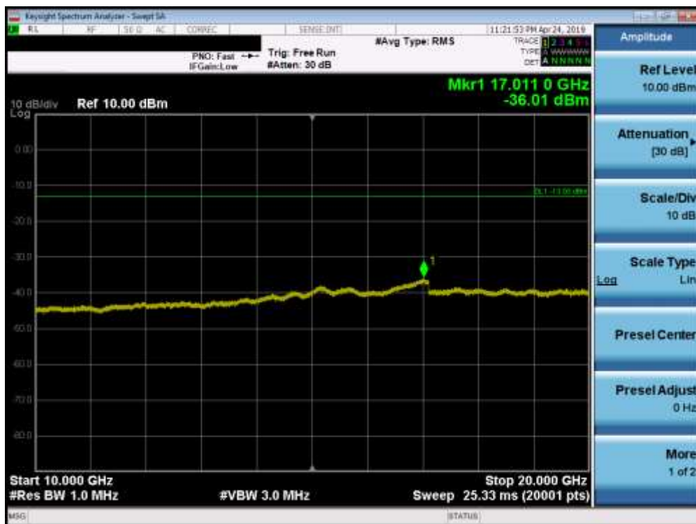
Plot 7-100. Conducted Spurious Plot (Band 2 - 20.0MHz QPSK - RB Size 1, RB Offset 0 - Mid Channel)
