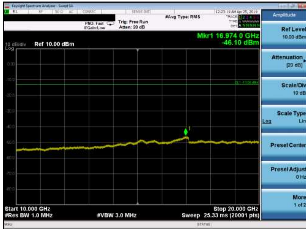
Plot 7-103. Conducted Spurious Plot (Band 2 - 20.0MHz QPSK - RB Size 1, RB Offset 0 - High Channel)
