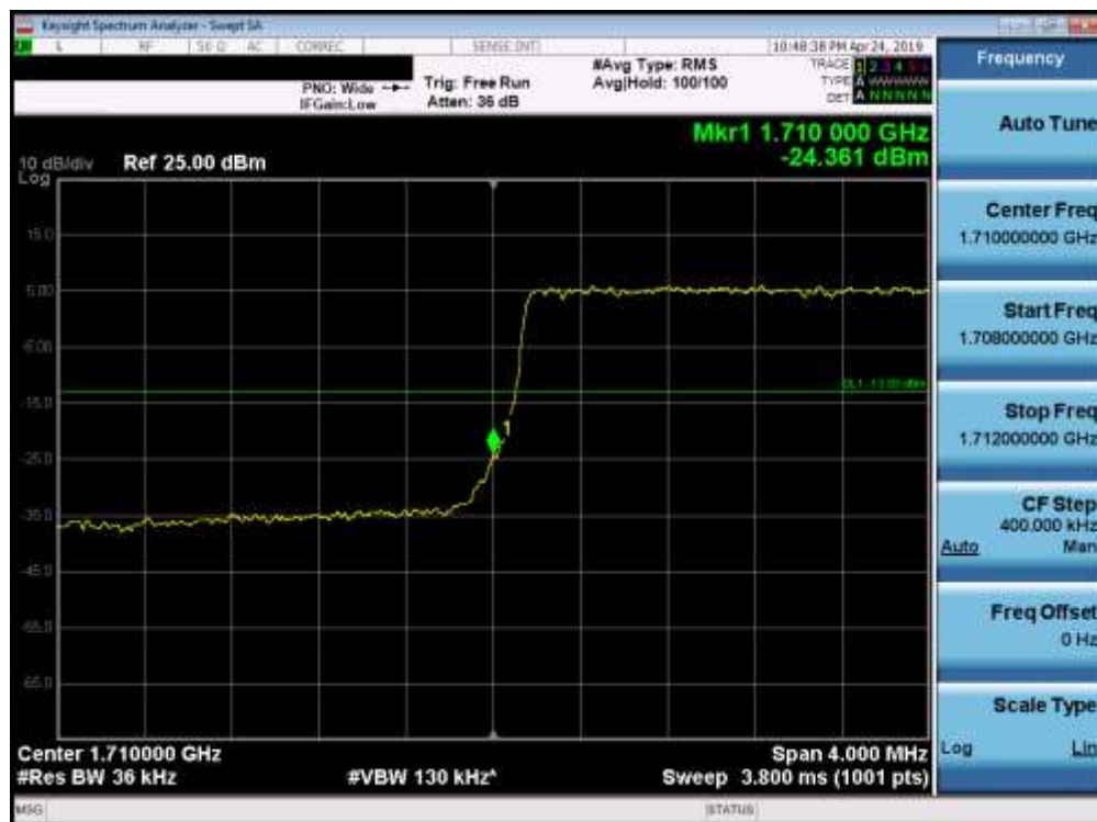
Plot 7-144. Lower Band Edge Plot (Band 66/4 - 3.0MHz QPSK - Full RB Configuration)
