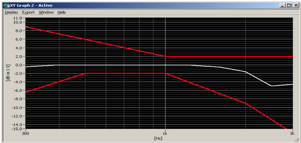
Figure 6-1 Axial Frequency Response
