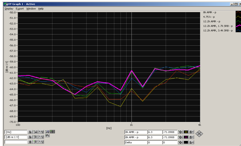
Figure 5-1 UMTS Audio Band Magnetic Noise
