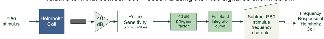
Figure 4-7 Frequency Response Validation
