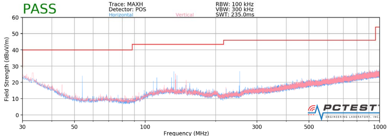
Plot 7-41. Radiated Spurious Plot below 1GHz
